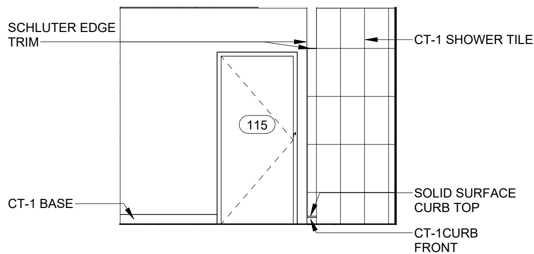
6 SHOWER ELEVATION D A2.2 SCALE: 1/4" = 1'-0"
