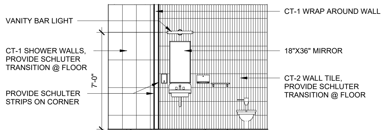
7 TYP. WET WALL A2.2 SCALE: 1/4" = 1'-0"
