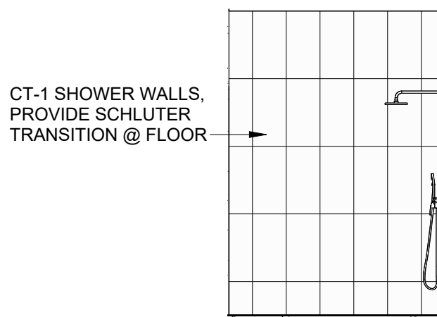
3 SHOWER ELEVATION A A2.2 SCALE: 1/4" = 1'-0"
