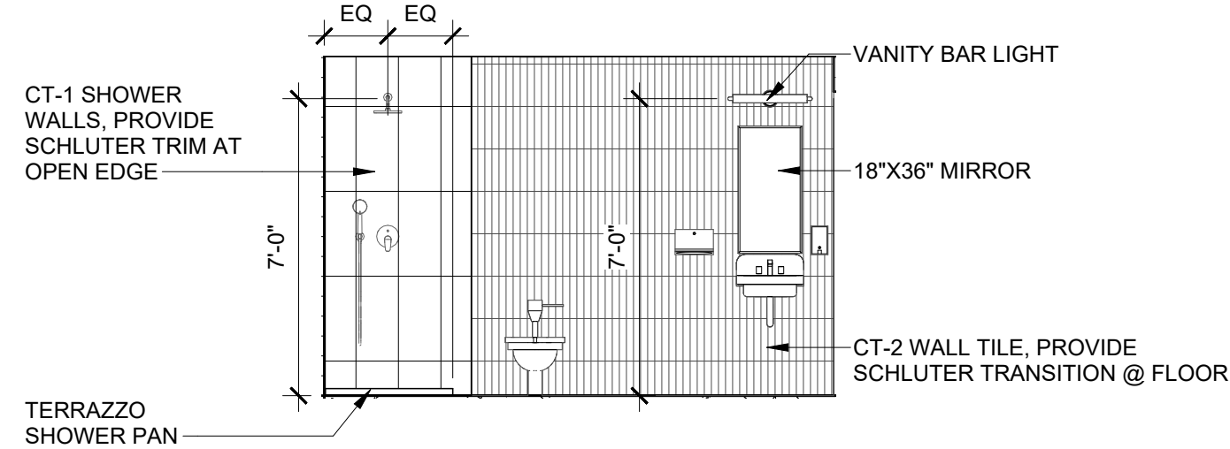
1 134 TLT ELEVATION A2.2 SCALE: 1/4" = 1'-0"
