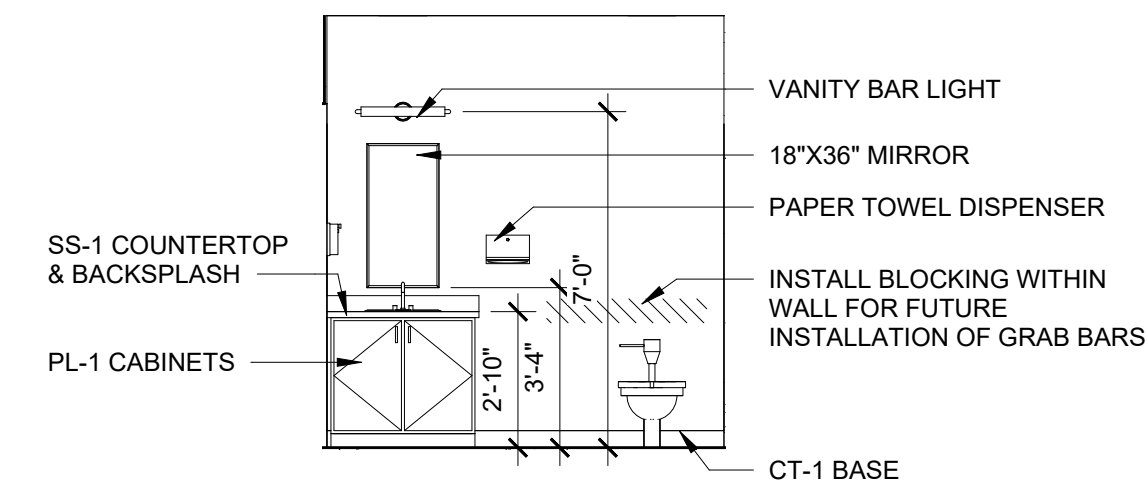
2 CHIEF TLT ELEVATION A2.2 SCALE: 1/4" = 1'-0"
