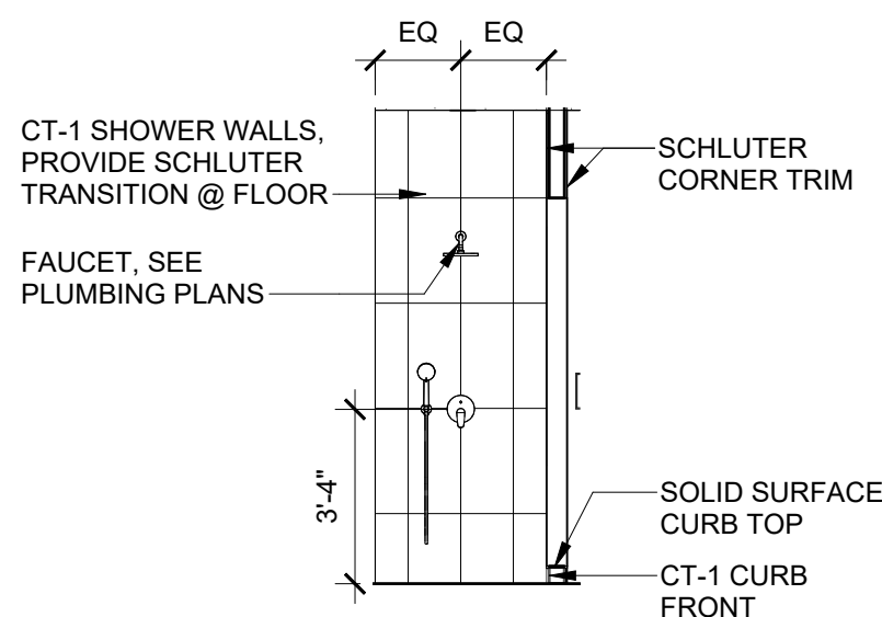
4 SHOWER ELEVATION B A2.2 SCALE: 1/4" = 1'-0"
