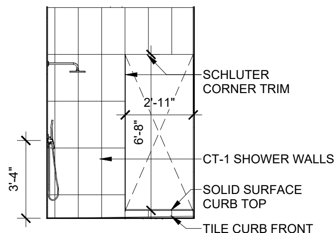
5 SHOWER ELEVATION C A2.2 SCALE: 1/4" = 1'-0"
