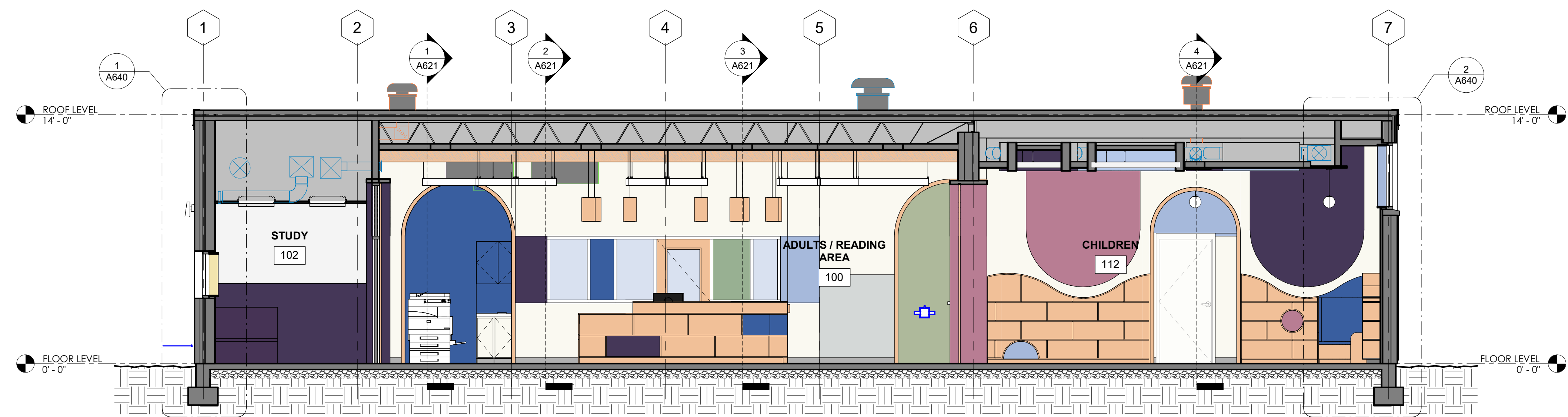
4 W/E BUILDING SECTION LOOKING NORTH 1/4" = 1'-0"
