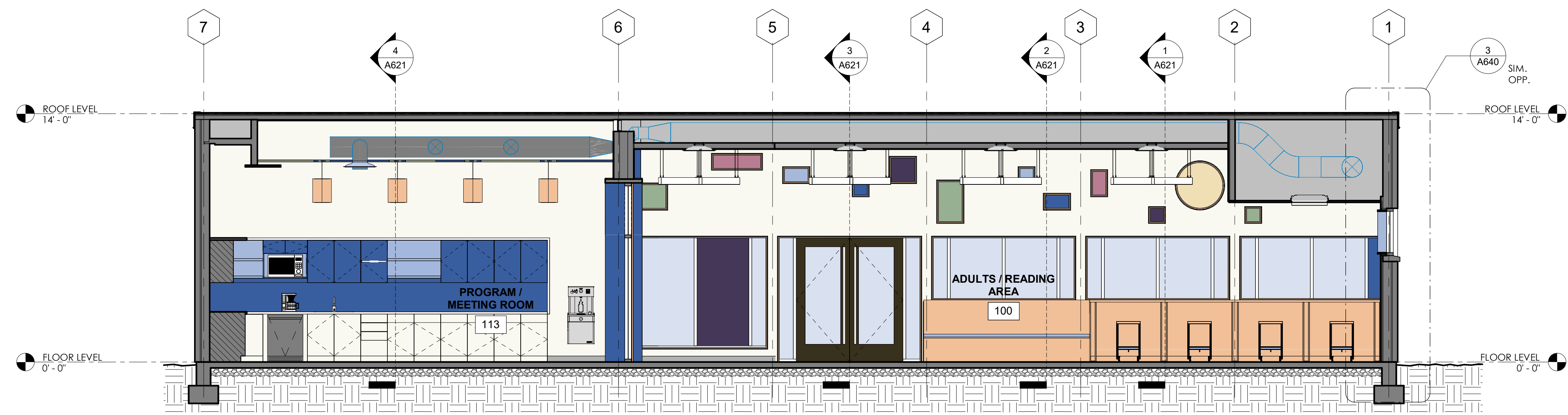
1 W/E BUILDING SECTION LOOKING SOUTH 1/4" = 1'-0"
