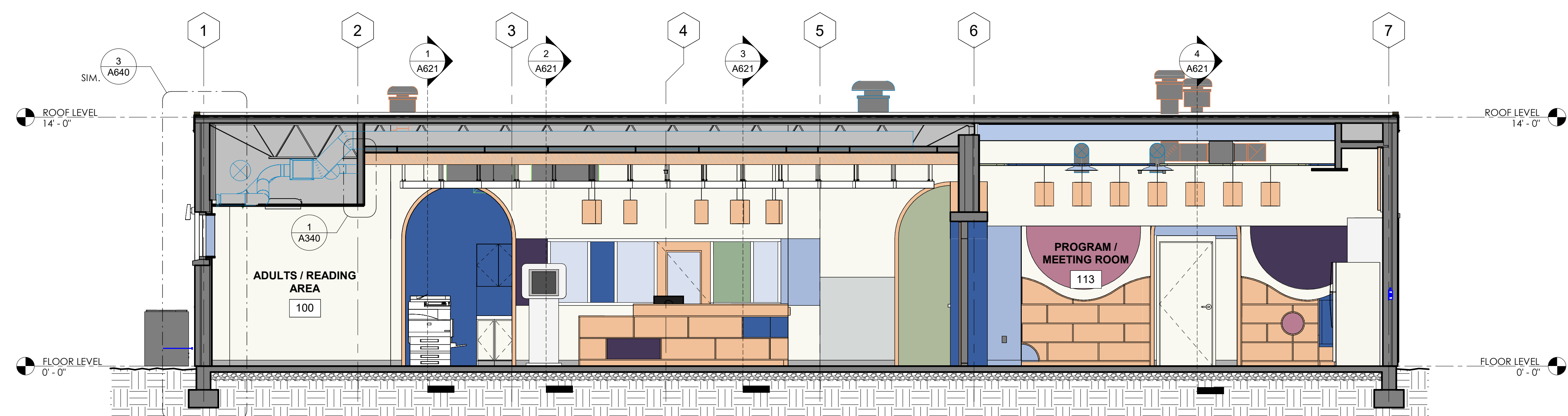
2 W/E BUILDING SECTION LOOKING NORTH 1/4" = 1'-0"
