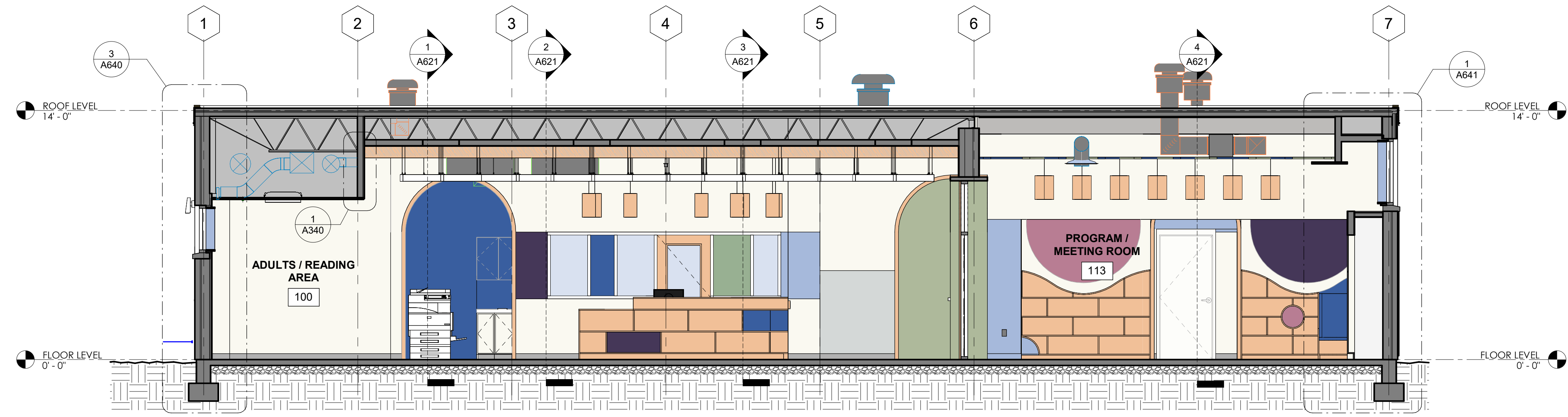
3 W/E BUILDING SECTION LOOKING NORTH 1/4" = 1'-0"
