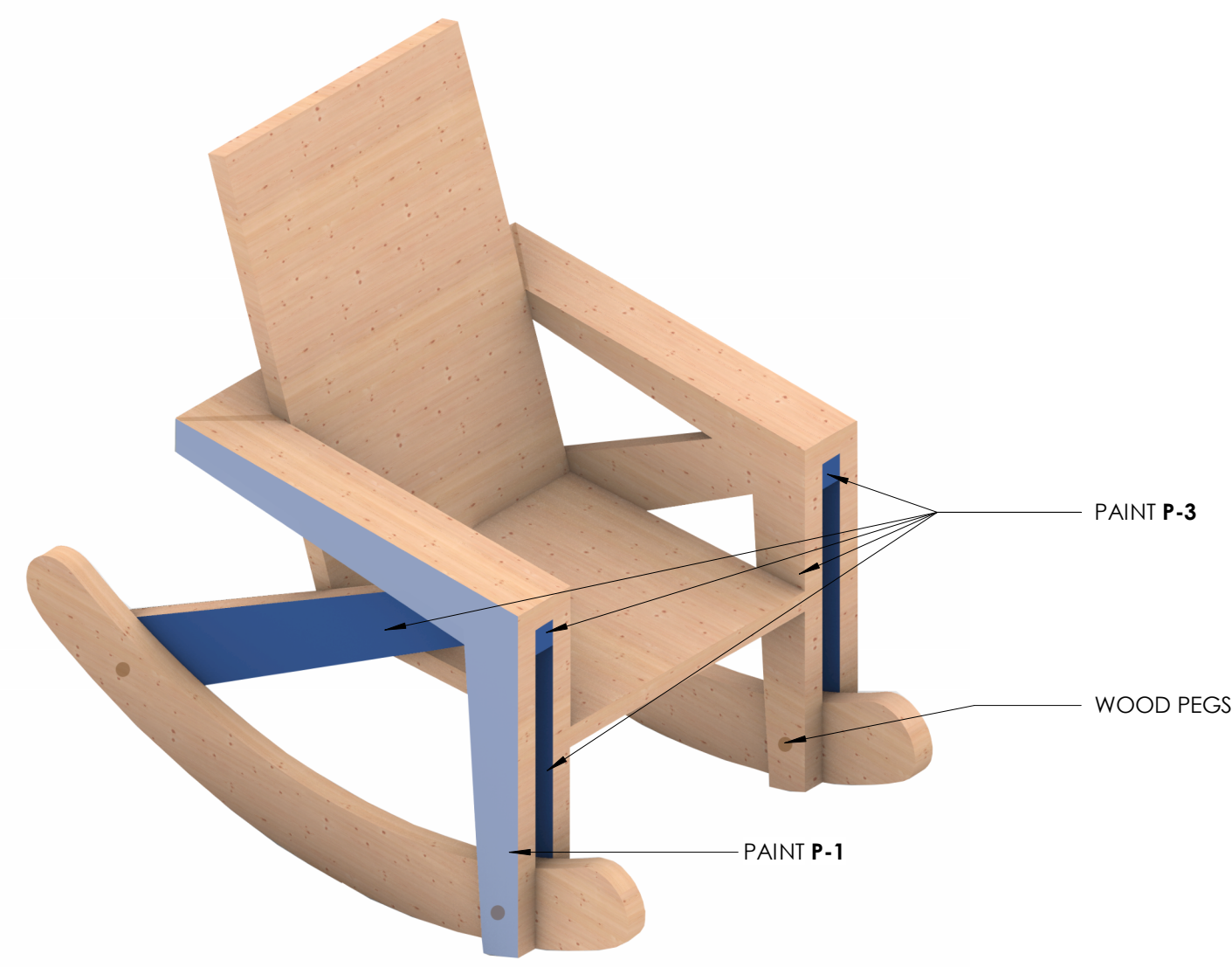
1 ADULT ARROW ROCKER CHAIR AXONOMETRIC A842
