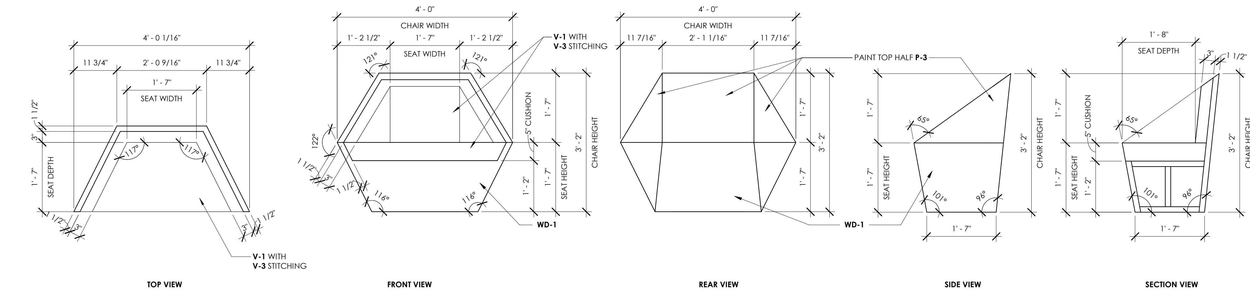
4 TEEN TAG CHAIR (CONTRACTOR TO PROVIDE QUANTITY OF TWO PLUS ONE SAMPLE) 3/4" = 1'-0"
