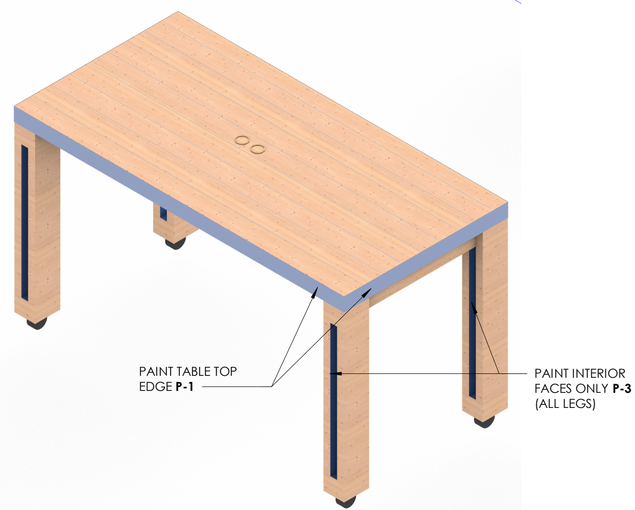
5 BUTCHER'S BLOCK TABLE AXONOMETRIC A842
