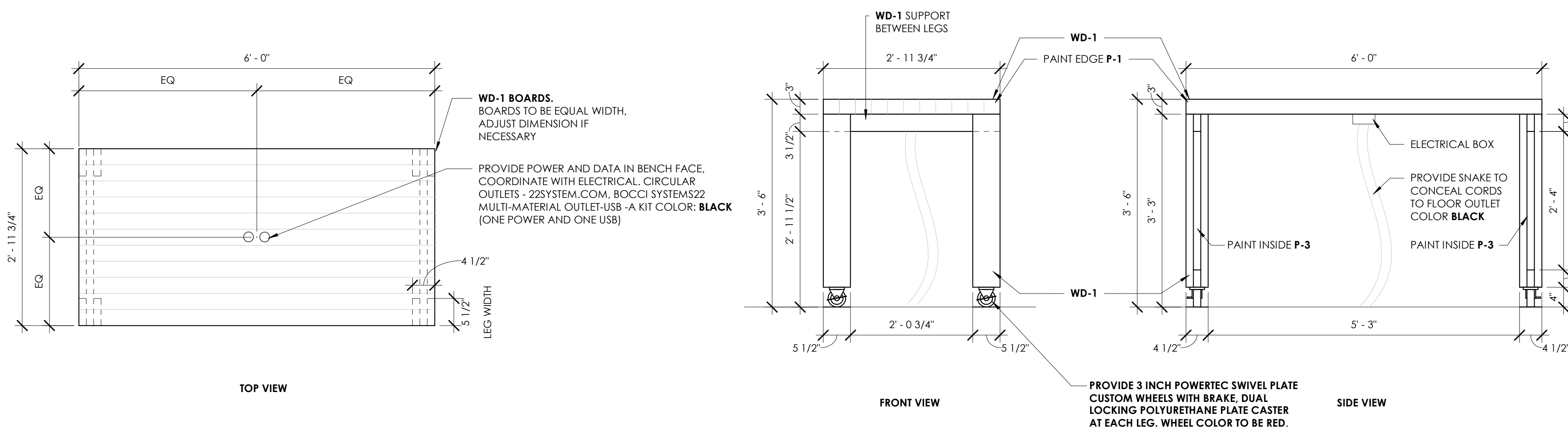
6 BUTCHER'S BLOCK TABLE (CONTRACTOR TO PROVIDE QUANTITY OF THREE) 3/4" = 1'-0"
