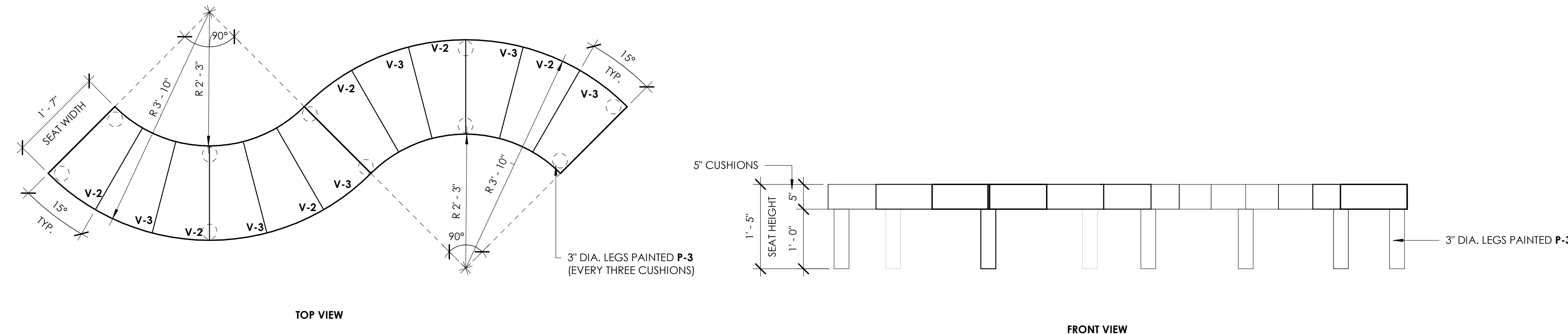
8 CHILDREN'S DOOR SWING BENCH (CONTRACTOR TO PROVIDE QUANTITY OF ONE) 3/4" = 1'-0"
