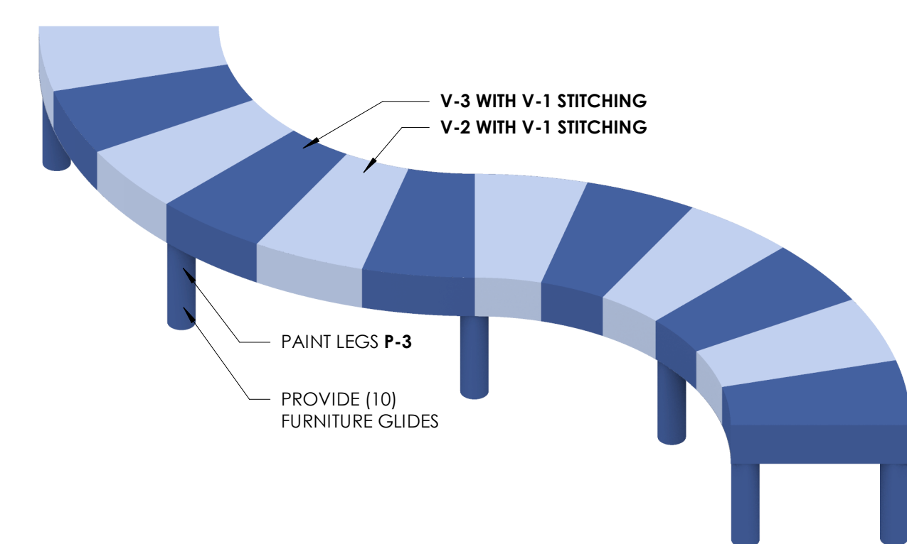
7 CHILDREN'S DOOR SWING BENCH AXONOMETRIC A842
