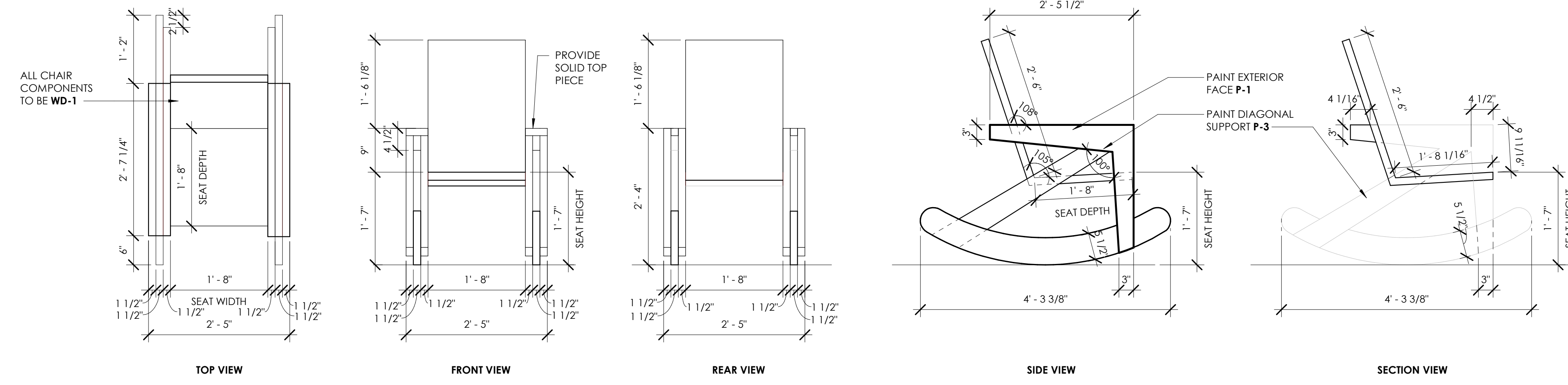
2 ADULT ARROW ROCKER CHAIR (CONTRACTOR TO PROVIDE QUANTITY OF TWO PLUS ONE SAMPLE) 3/4" = 1'-0"
