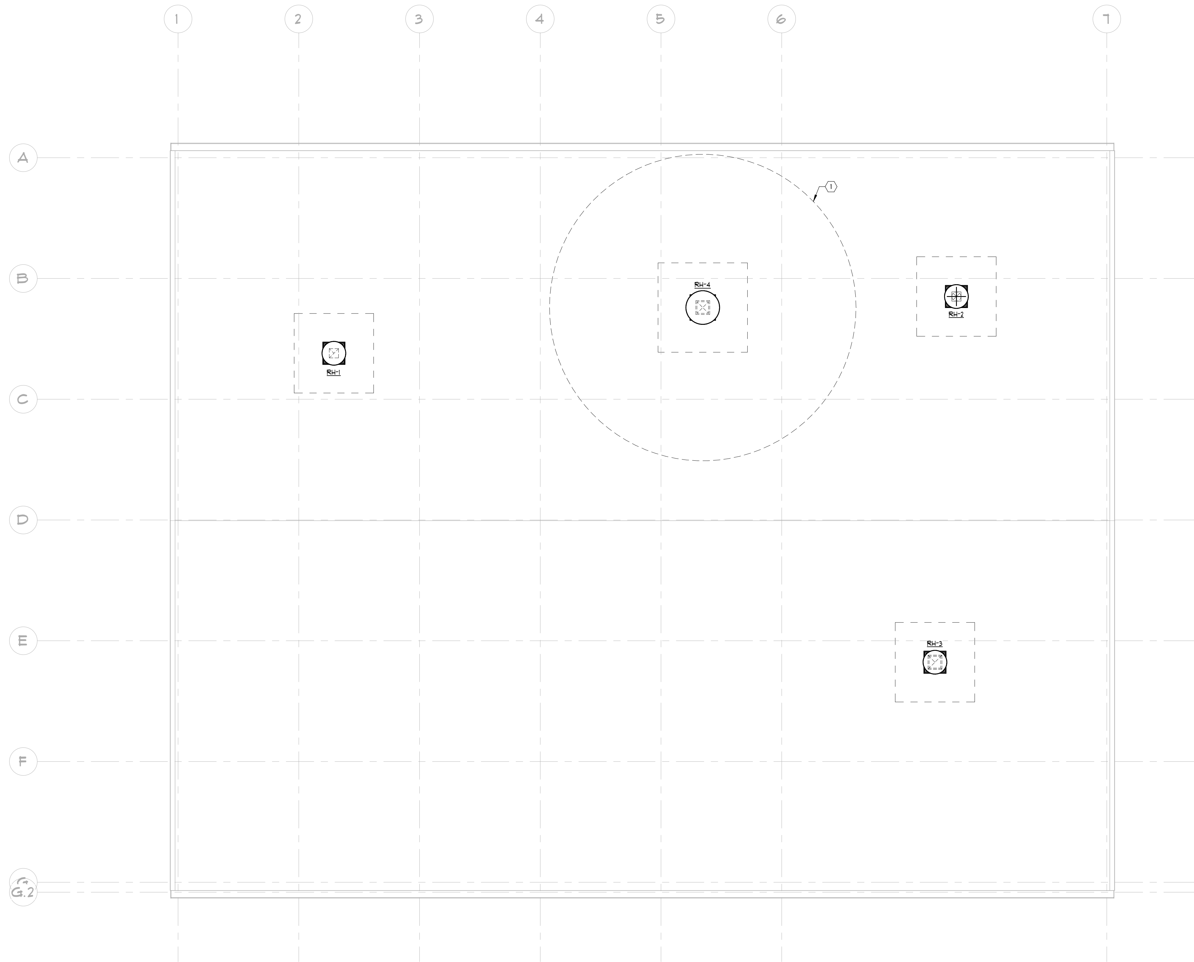
1 ROOF PLAN - HVAC 1/4" = 1'-0" KEY NOTES: ① EXHAUST AND PLUMBING VENT TERMINATIONS TO BE NO LESS THAN 10' FROM OUTSIDE AIR INTAKE.
