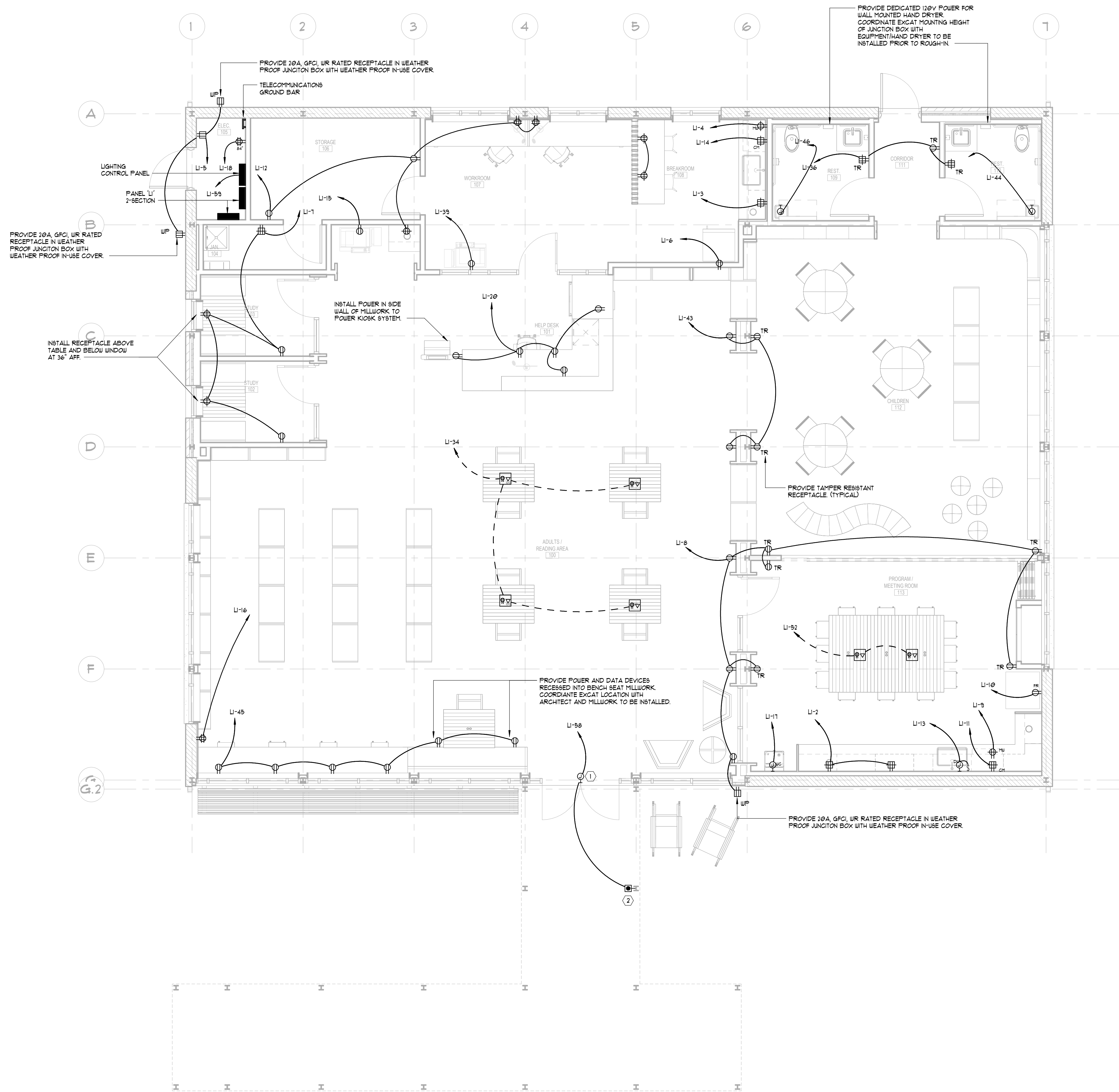
ELECTRICAL FLOOR PLAN - LEVEL 01 1/4" = 1'-0" NORTH
