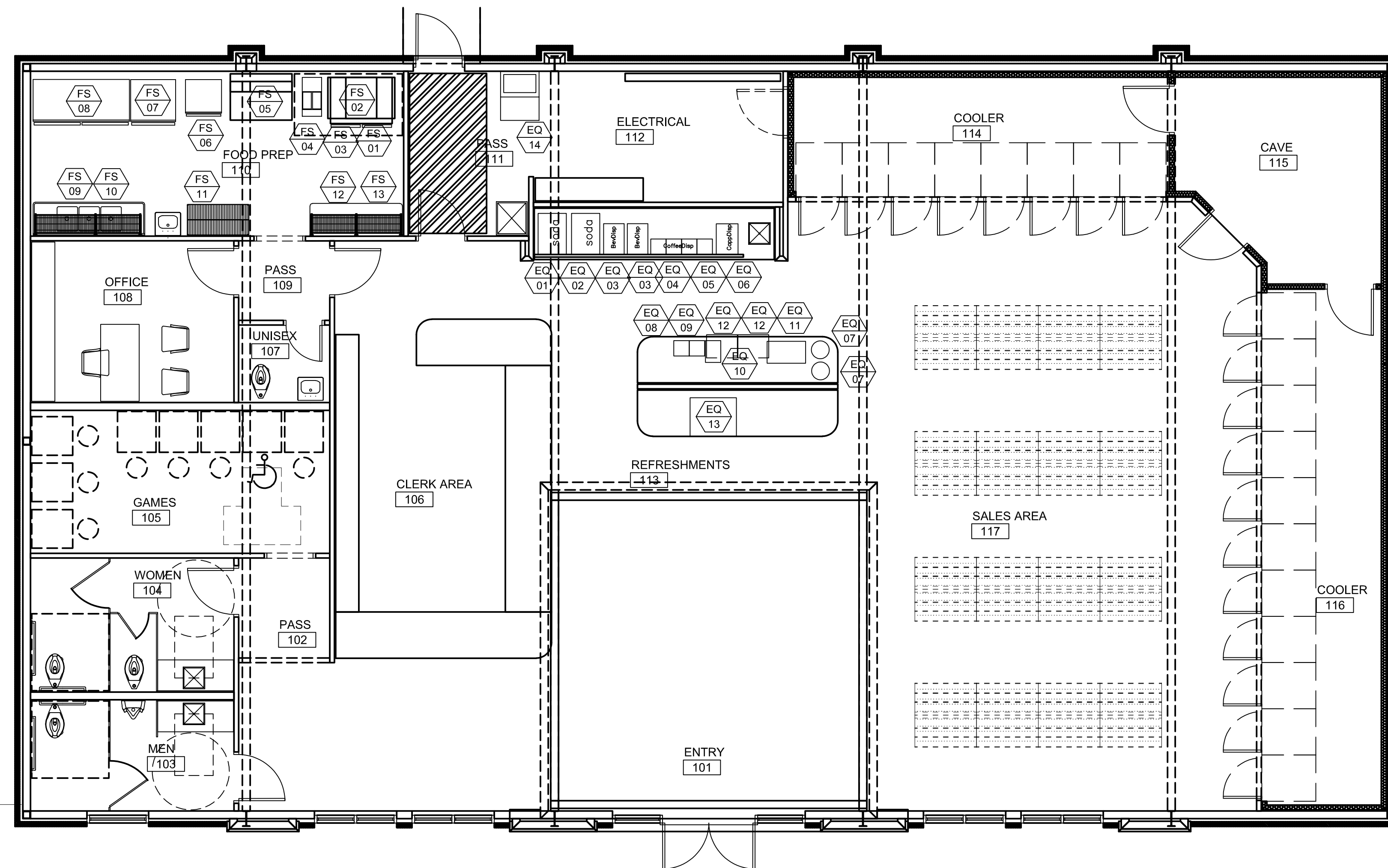
PROJECT NORTH EQUIPMENT PLAN SCALE: 3/16" = 1'-0"
