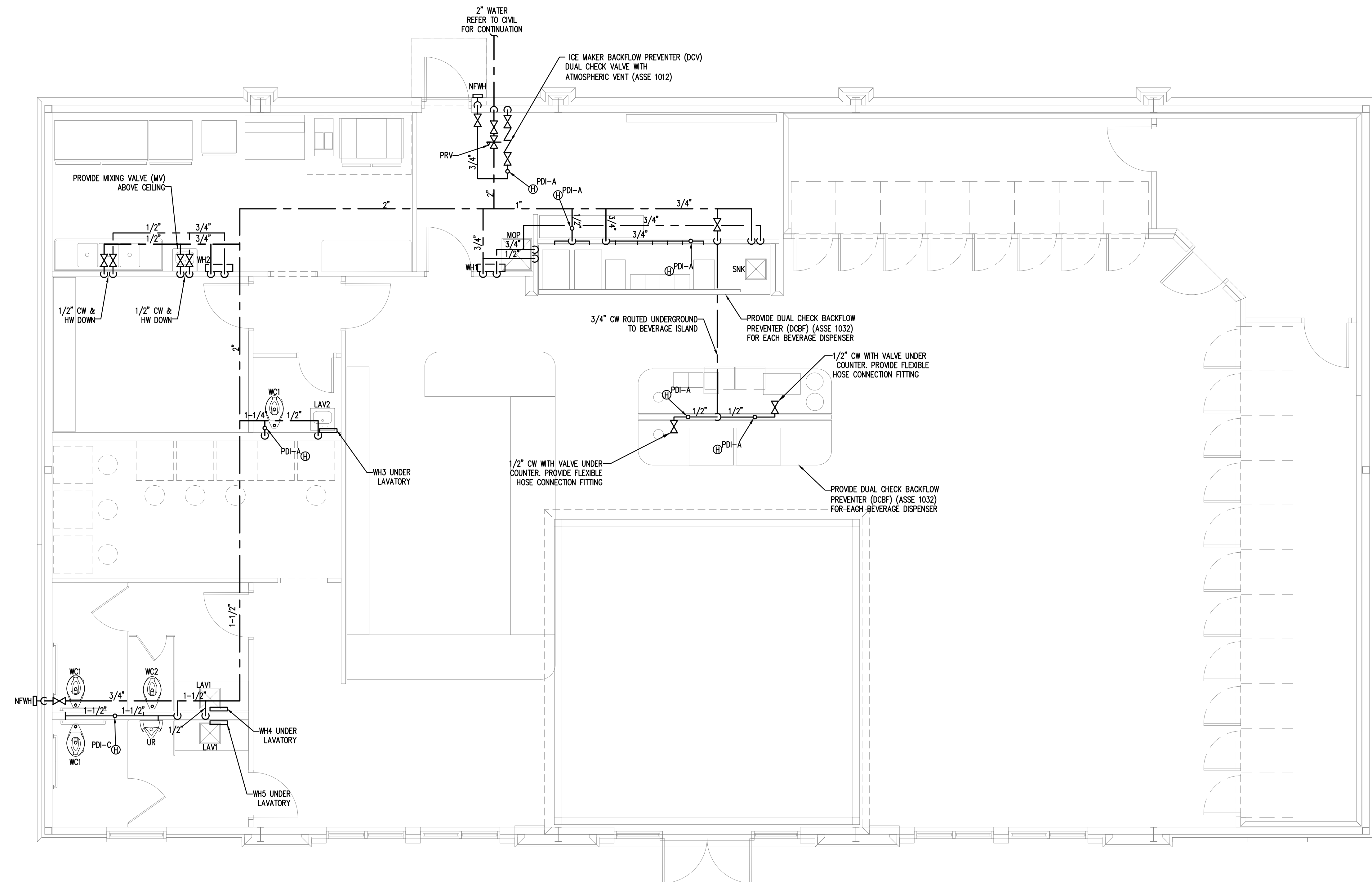
1 PLUMBING PLAN - WATER SCALE: 1/4"=1'-0"
