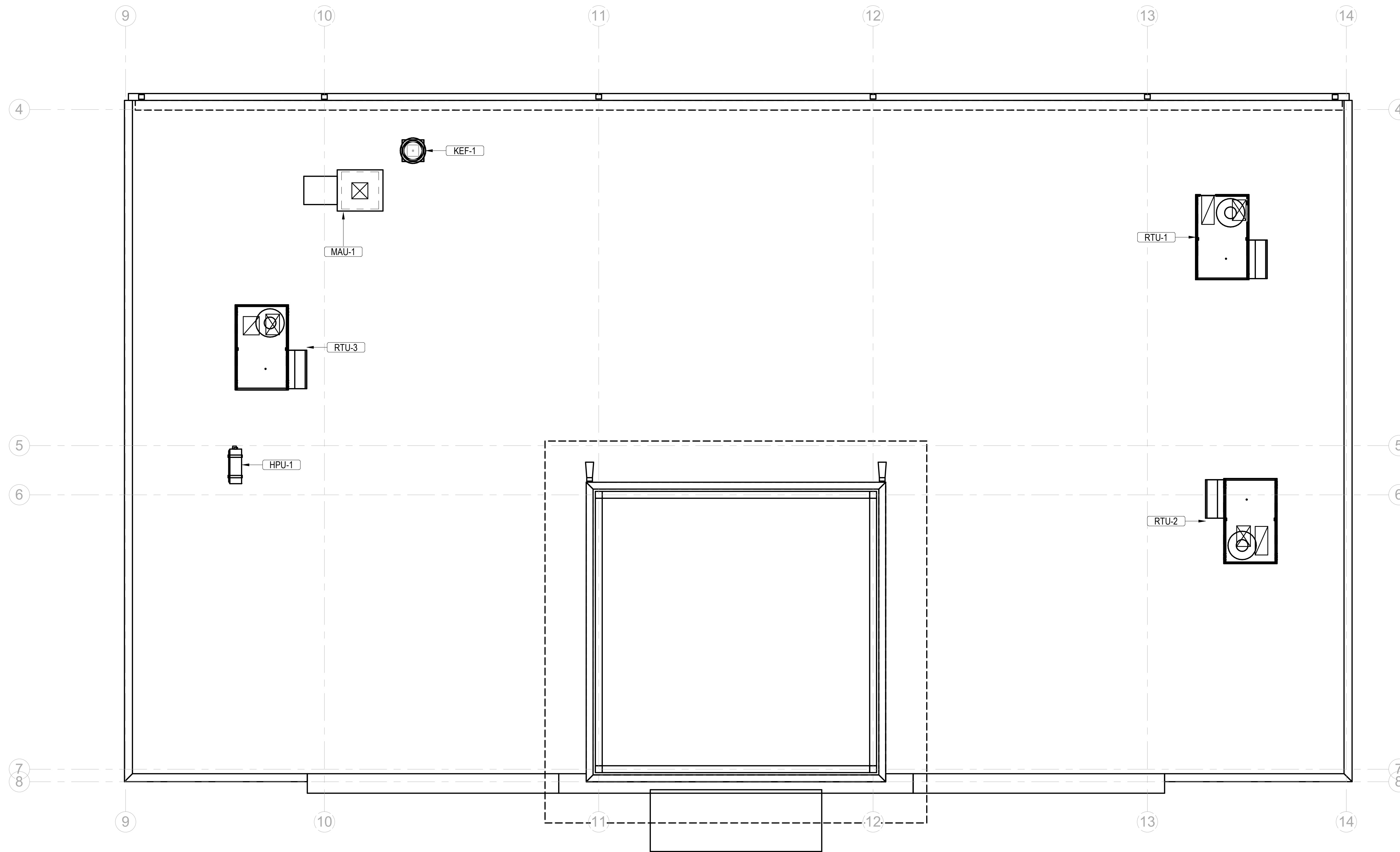
1 LEVEL 2 HVAC PLAN M1.2 1/4" = 1'-0"
