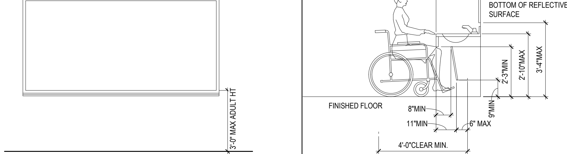
02 TYP. MARKERBOARD MOUNTING HEIGHT 3/8" = 1'-0"
