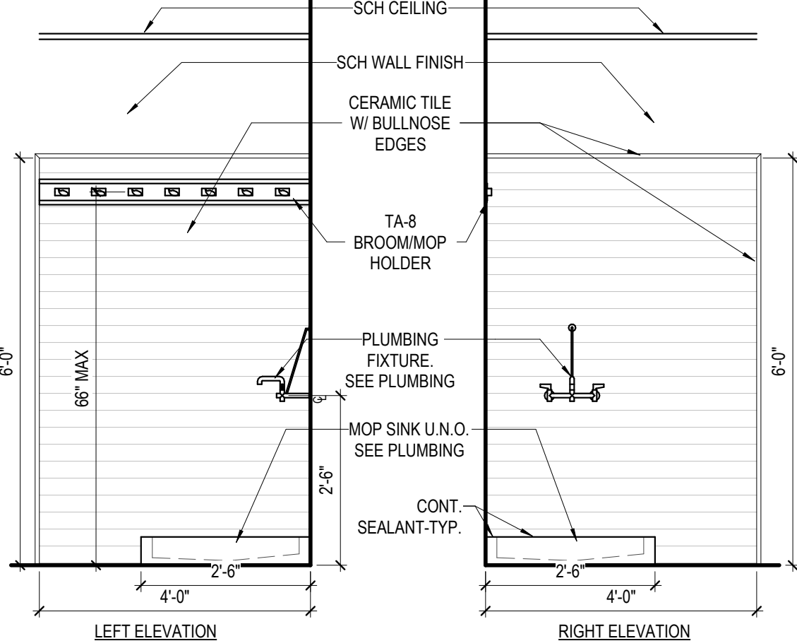
04 TYP CUSTODIAL CLOSET 1/2" = 1'-0"
