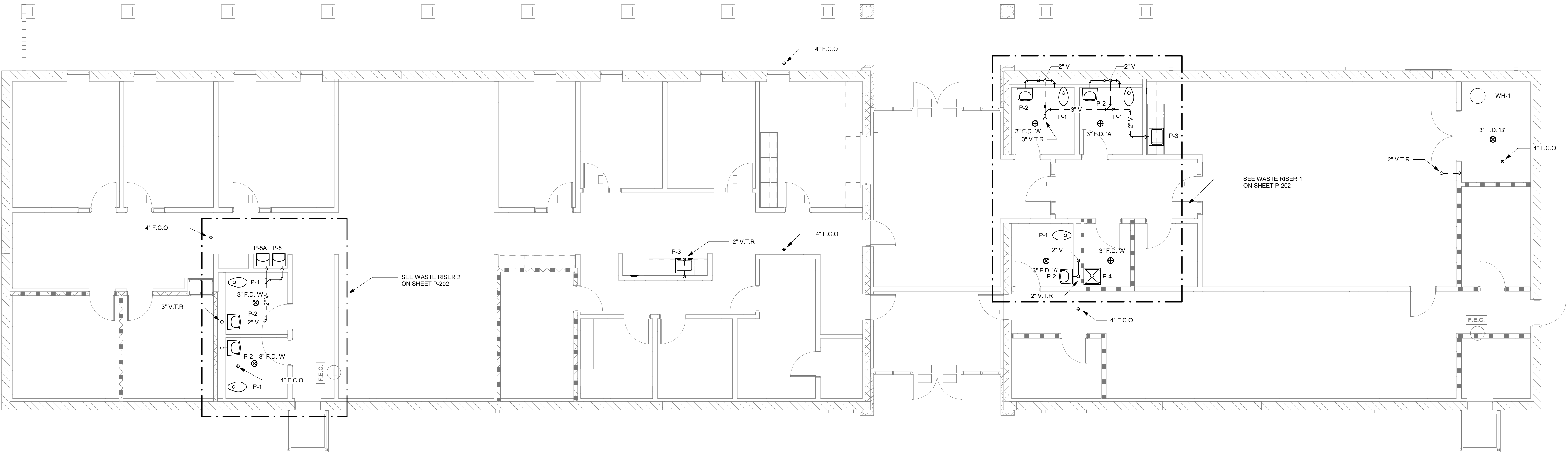
PLUMBING FLOOR PLAN - WASTE PIPING - ABOVE SLAB SCALE: 3/16" = 1'-0"
