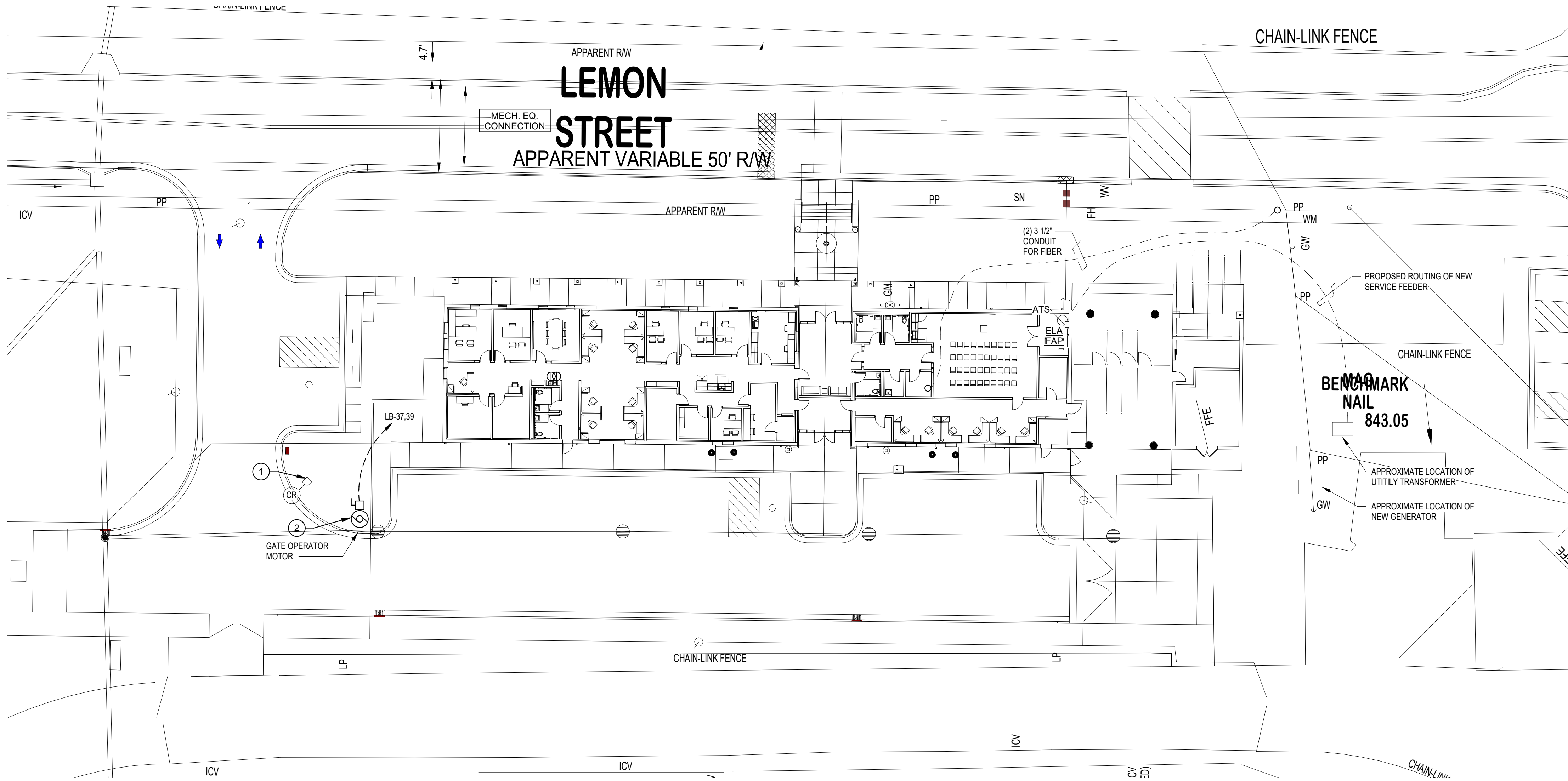
ELECTRICAL SITE PLAN SCALE: 1" = 20'-0"
