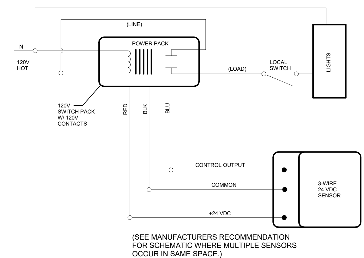
2 WIRING DIAGRAM-SENSOR CONTROL-LIGHTING E2.1 NO SCALE
