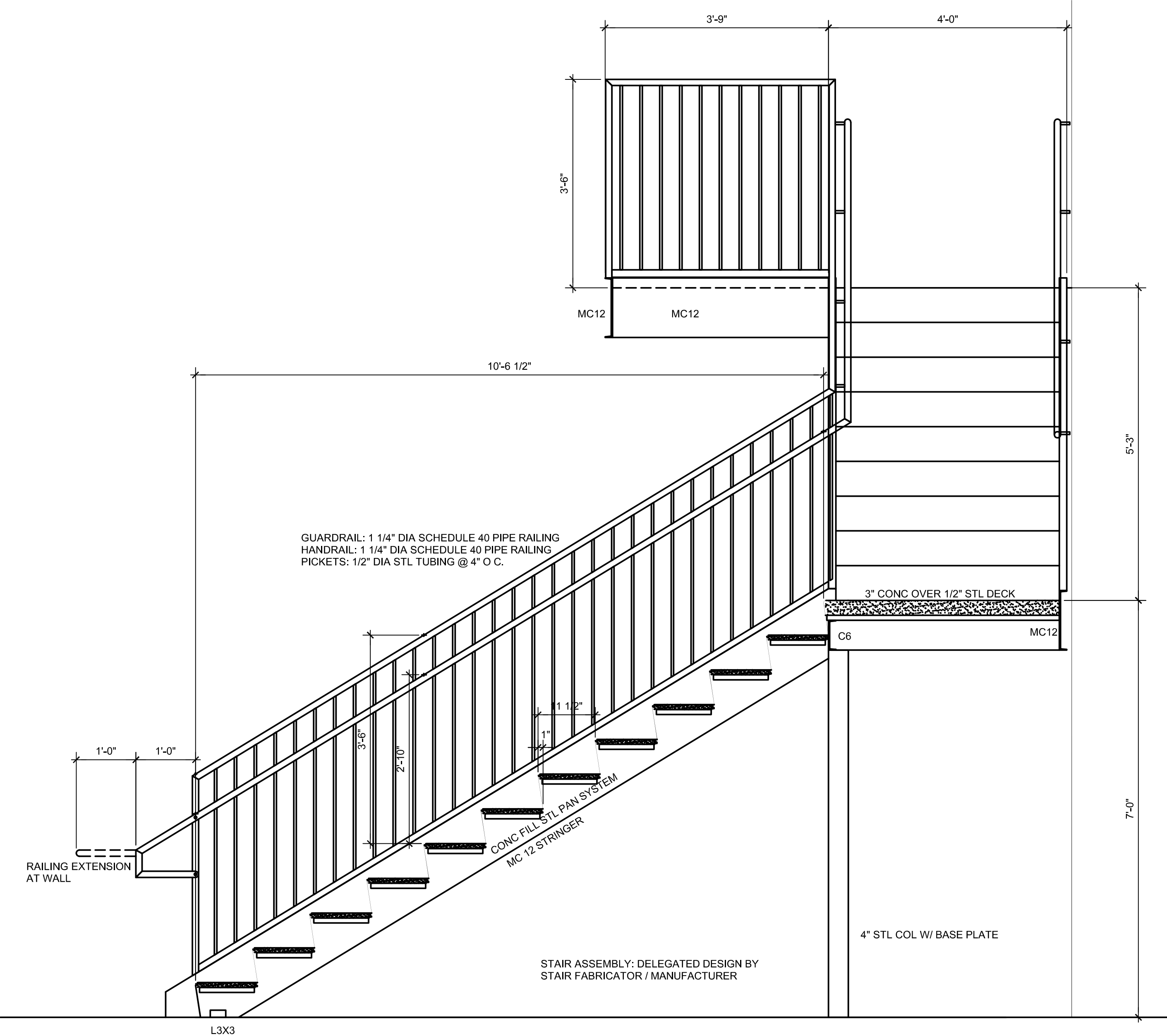
D3 STAIR SECTION: STAIR E110 SCALE: 3/4" = 1'-0"
