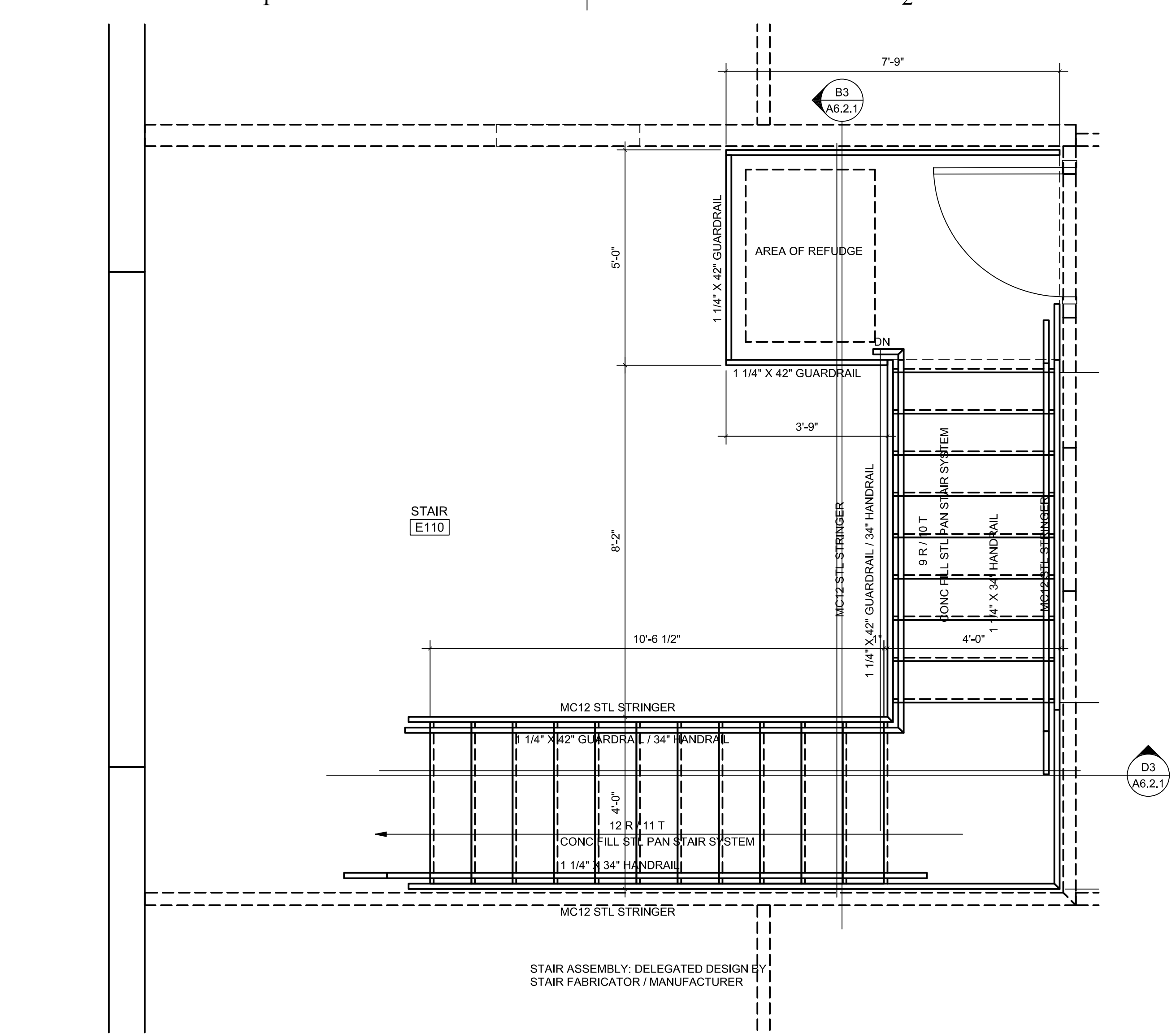
ENLARGED PLAN AT SECOND FLOOR: STAIR E110 SCALE: 1/2" = 1'-0"
