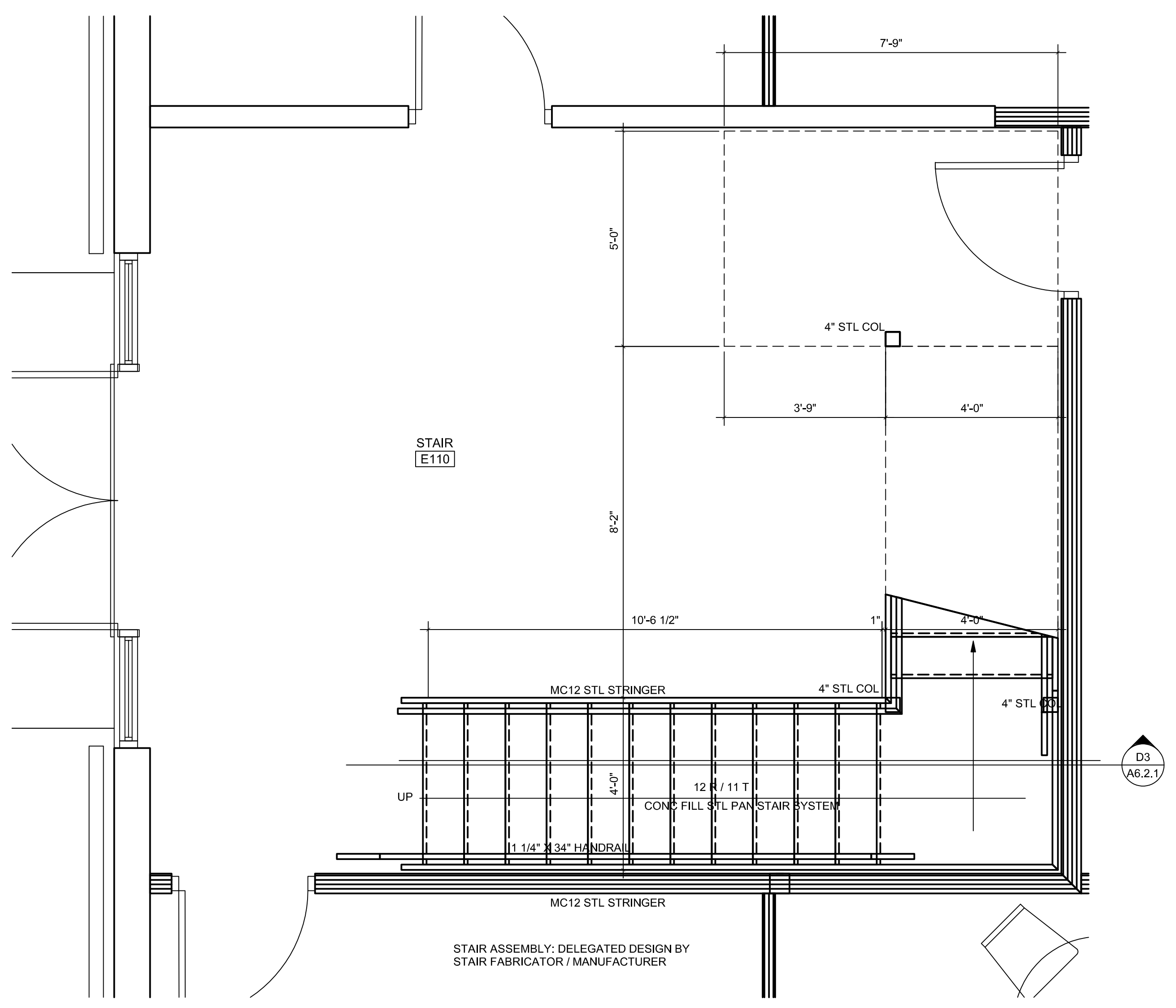
ENLARGED PLAN AT FIRST FLOOR: STAIR E110 SCALE: 1/2" = 1'-0"
