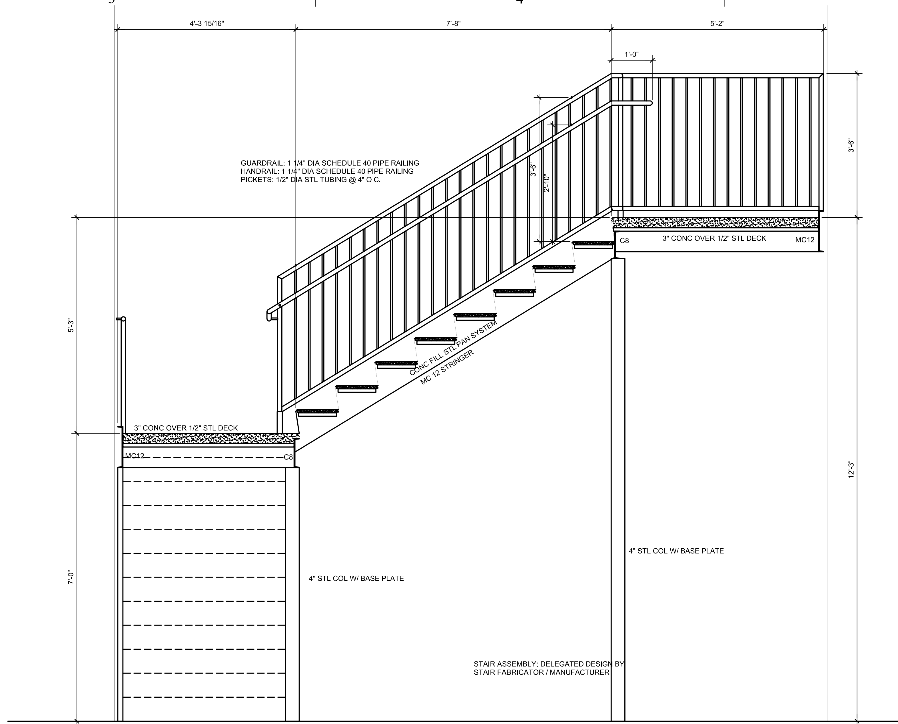
B3 STAIR SECTION: STAIR E110 SCALE: 3/4" = 1'-0"
