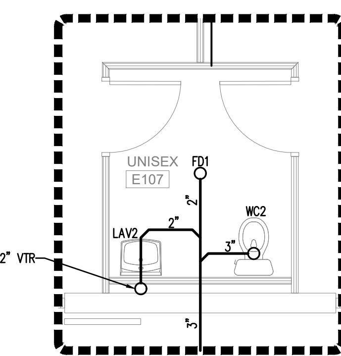
5 EDUCATION CLASSROOM RESTROOM PLUMBING PLAN - SEWER SCALE: 1/4"=1'-0"
