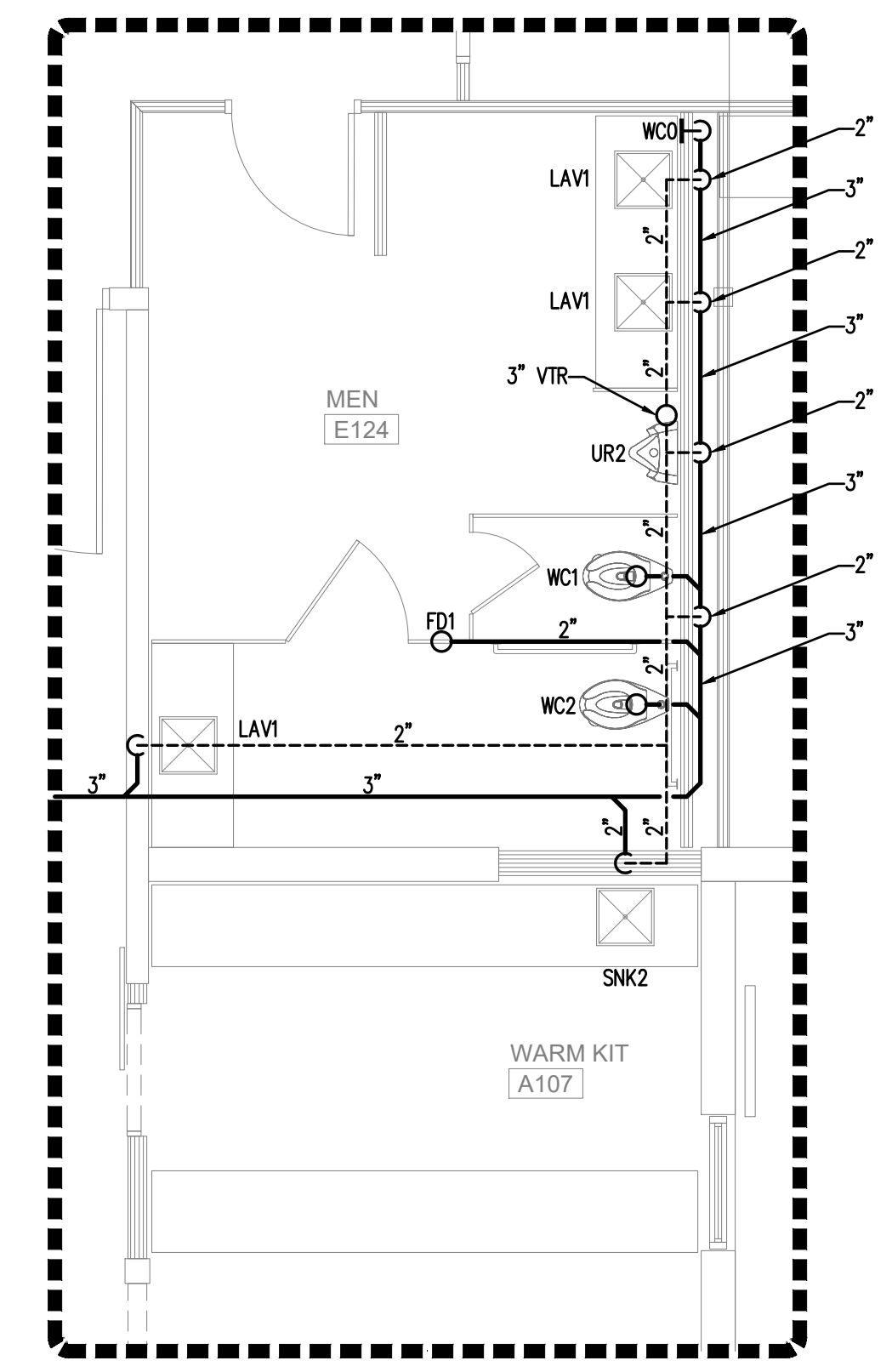
9 EDUCATION MEN'S RESTROOM PLUMBING PLAN - SEWER SCALE: 1/4"=1'-0"
