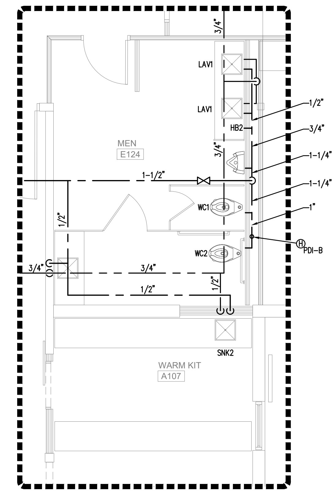
10 EDUCATION MEN'S RESTROOM PLUMBING PLAN - WATER SCALE: 1/4"=1'-0"
