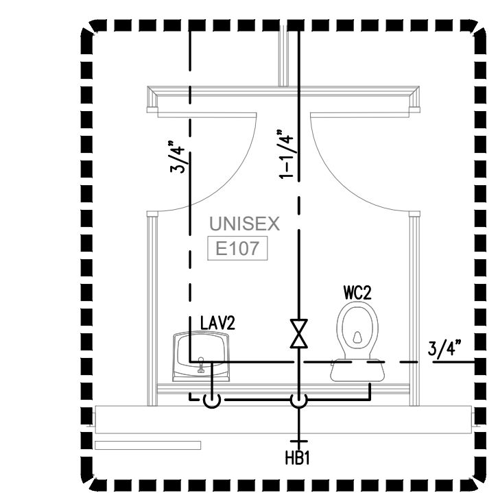
6 EDUCATION CLASSROOM RESTROOM PLUMBING PLAN - WATER SCALE: 1/4"=1'-0"
