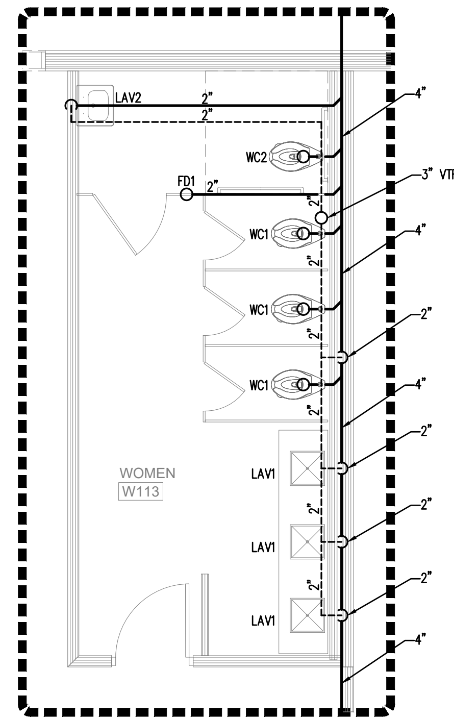
1 WORSHIP MEN'S RESTROOM PLUMBING PLAN - SEWER SCALE: 1/4"=1'-0"
