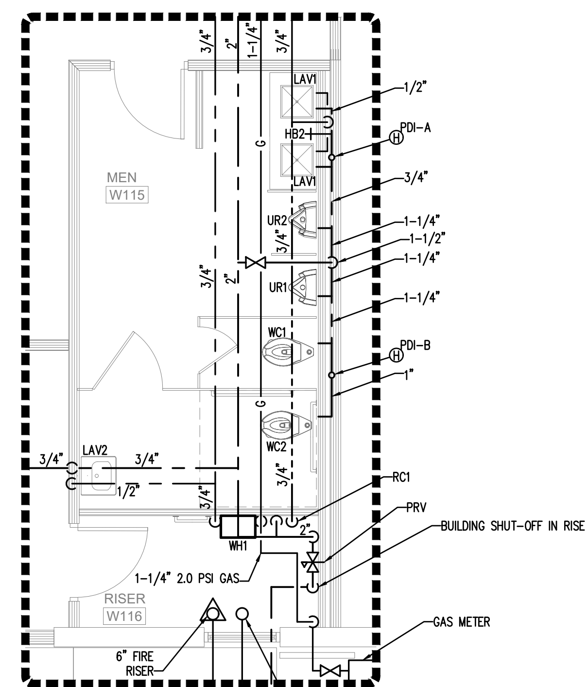
4 WORSHIP MEN'S RESTROOM PLUMBING PLAN - WATER SCALE: 1/4"=1'-0"
