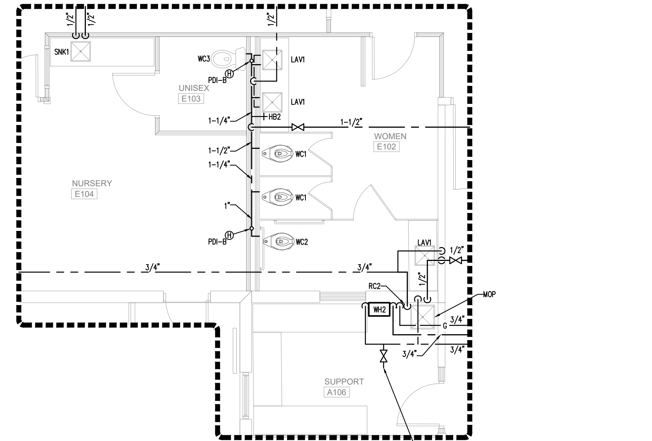
8 EDUCATION WOMEN'S RESTROOM PLUMBING PLAN - WATER SCALE: 1/4"=1'-0"
