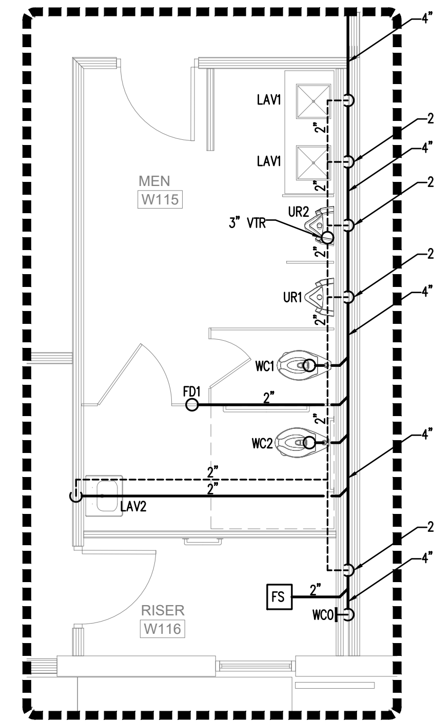
3 WORSHIP MEN'S RESTROOM PLUMBING PLAN - SEWER SCALE: 1/4"=1'-0"
