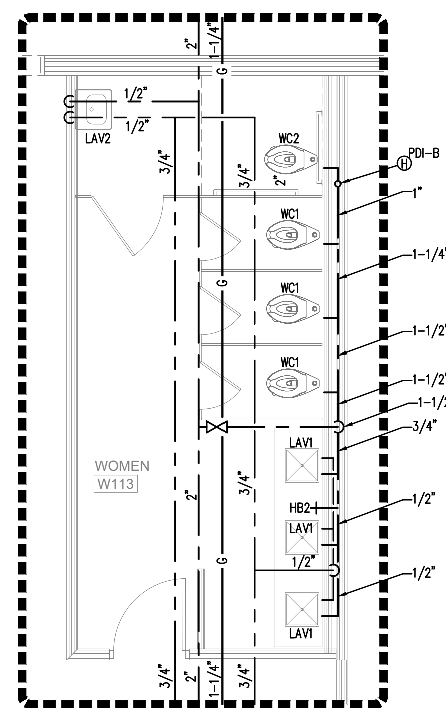
2 WORSHIP MEN'S RESTROOM PLUMBING PLAN - WATER SCALE: 1/4"=1'-0"
