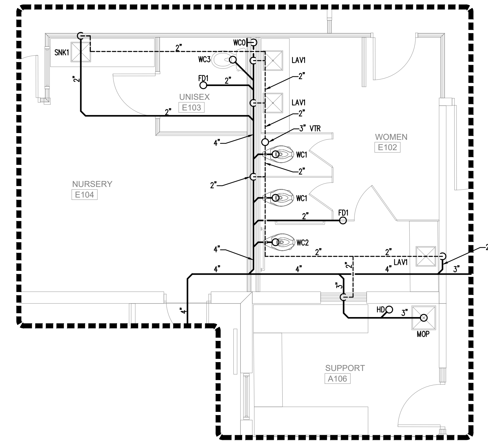
7 EDUCATION WOMEN'S RESTROOM PLUMBING PLAN - SEWER SCALE: 1/4"=1'-0"
