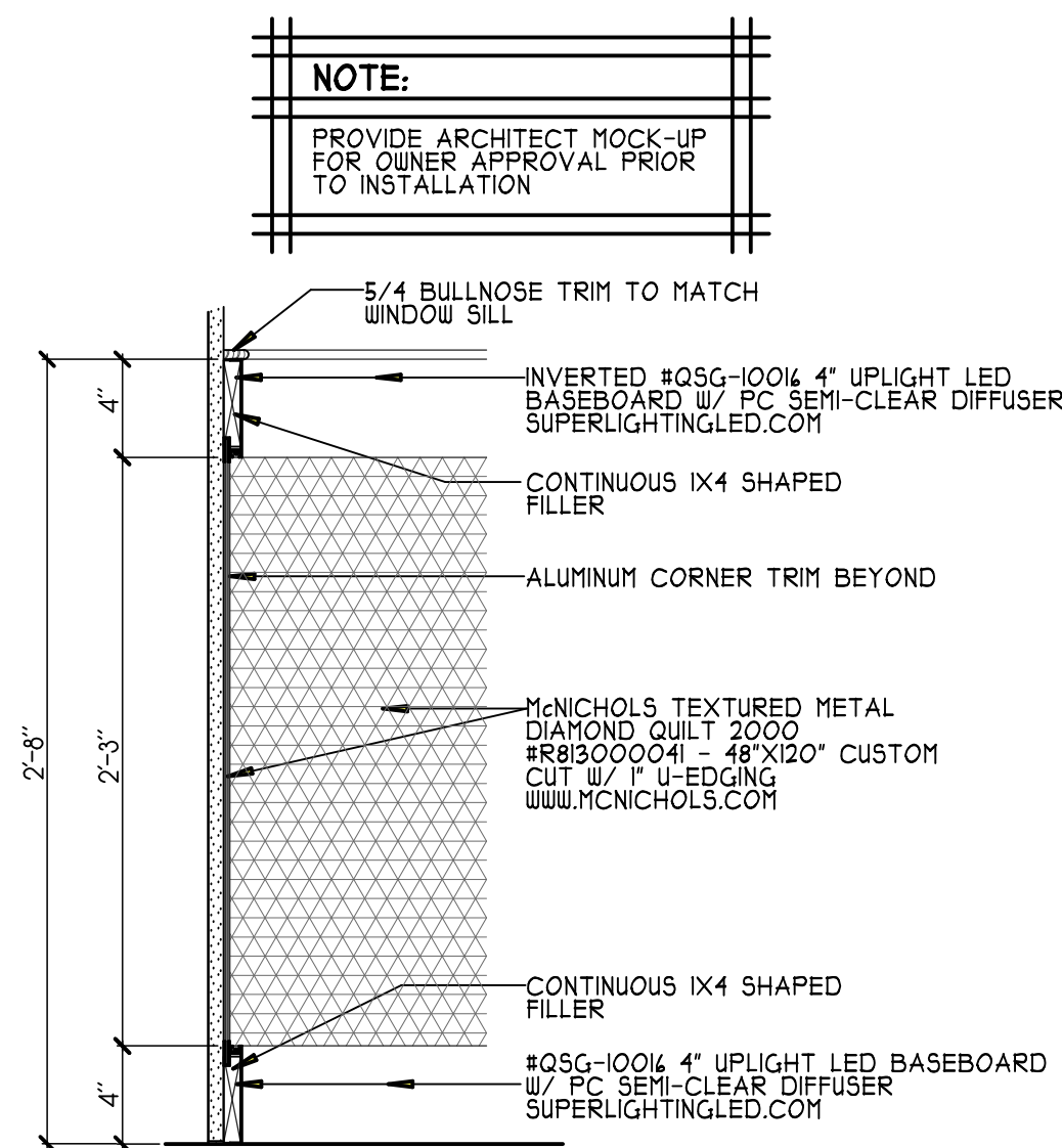
WAINSCOT DETAIL SCALE: 1 1/2" = 1'-0"
