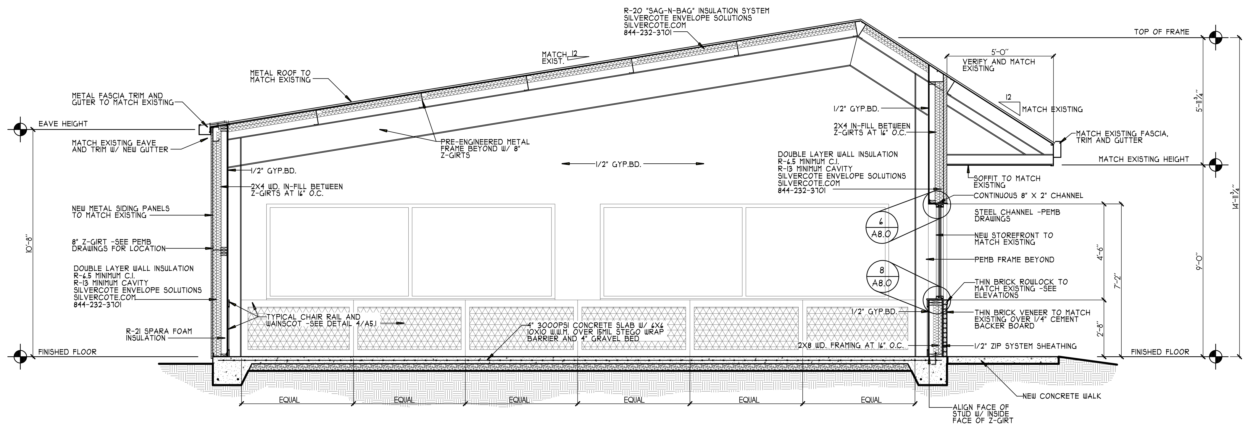
TRANSVERSE SECTION AT DINING SCALE: 3/8" = 1'-0"
