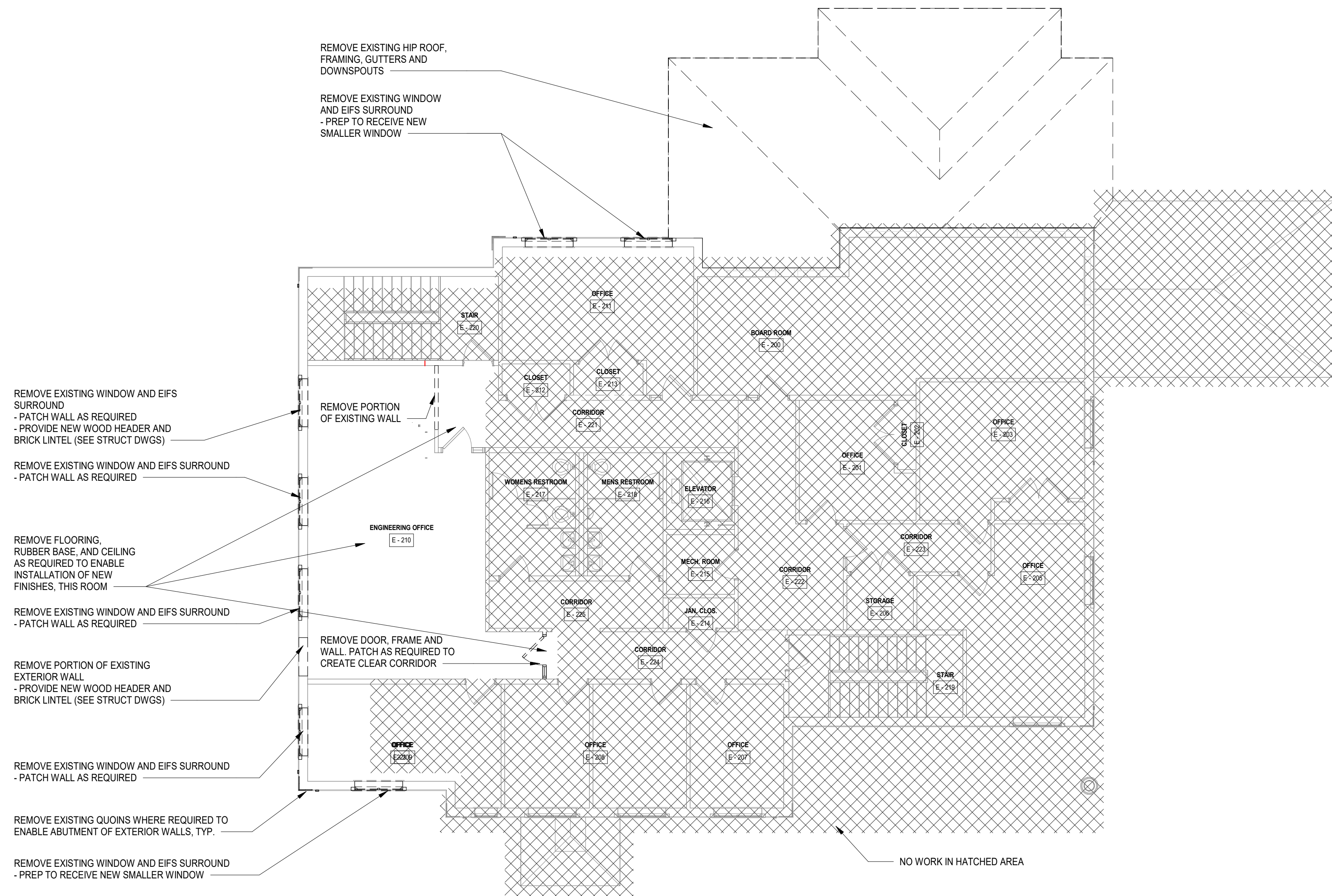
1 SECOND FLOOR DEMOLITION PLAN SCALE: 1/8" = 1'-0"
