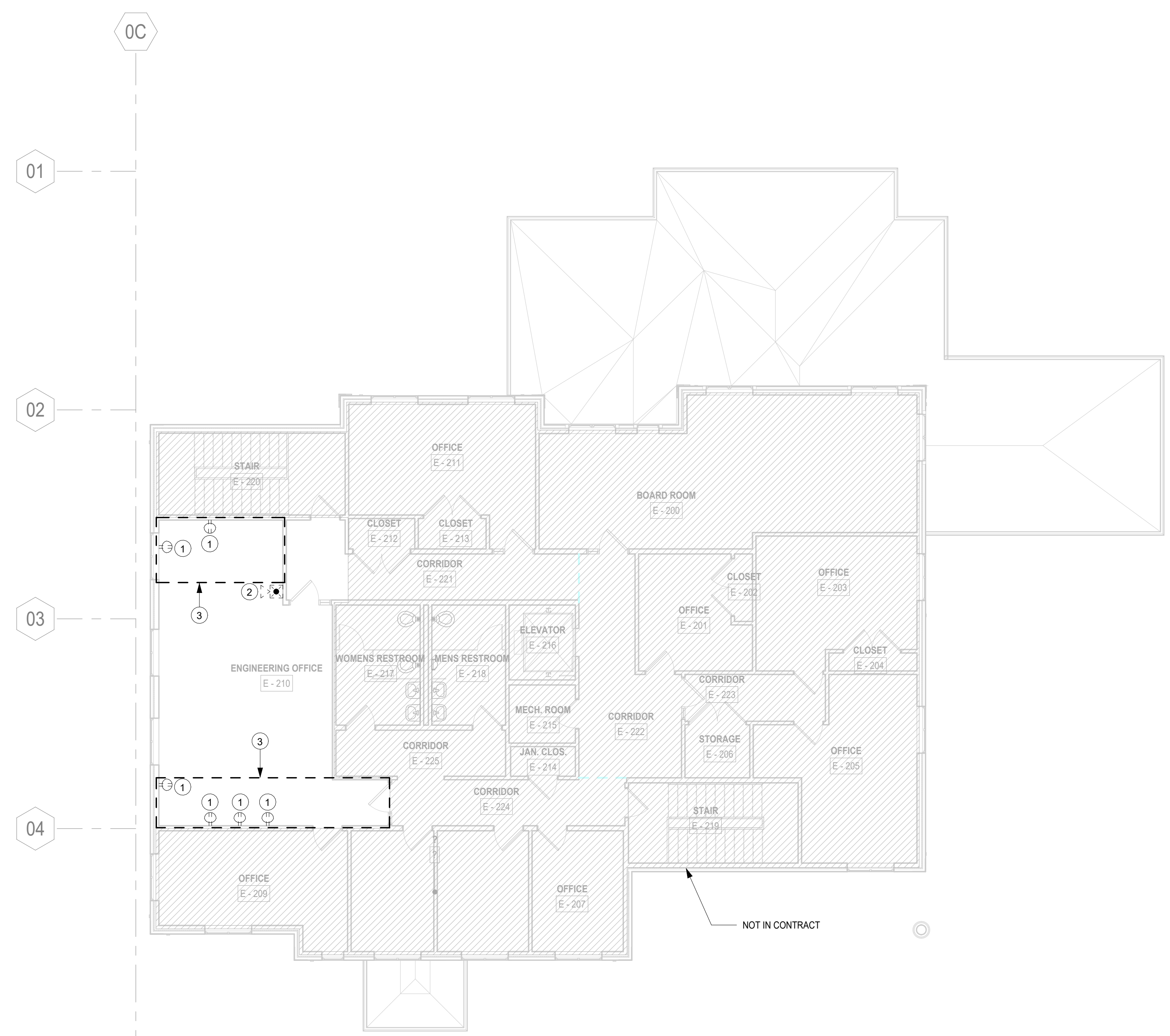
1 SECOND FLOOR POWER & SYSTEMS PLAN - DEMOLITION SCALE: 1/8" = 1'-0"
