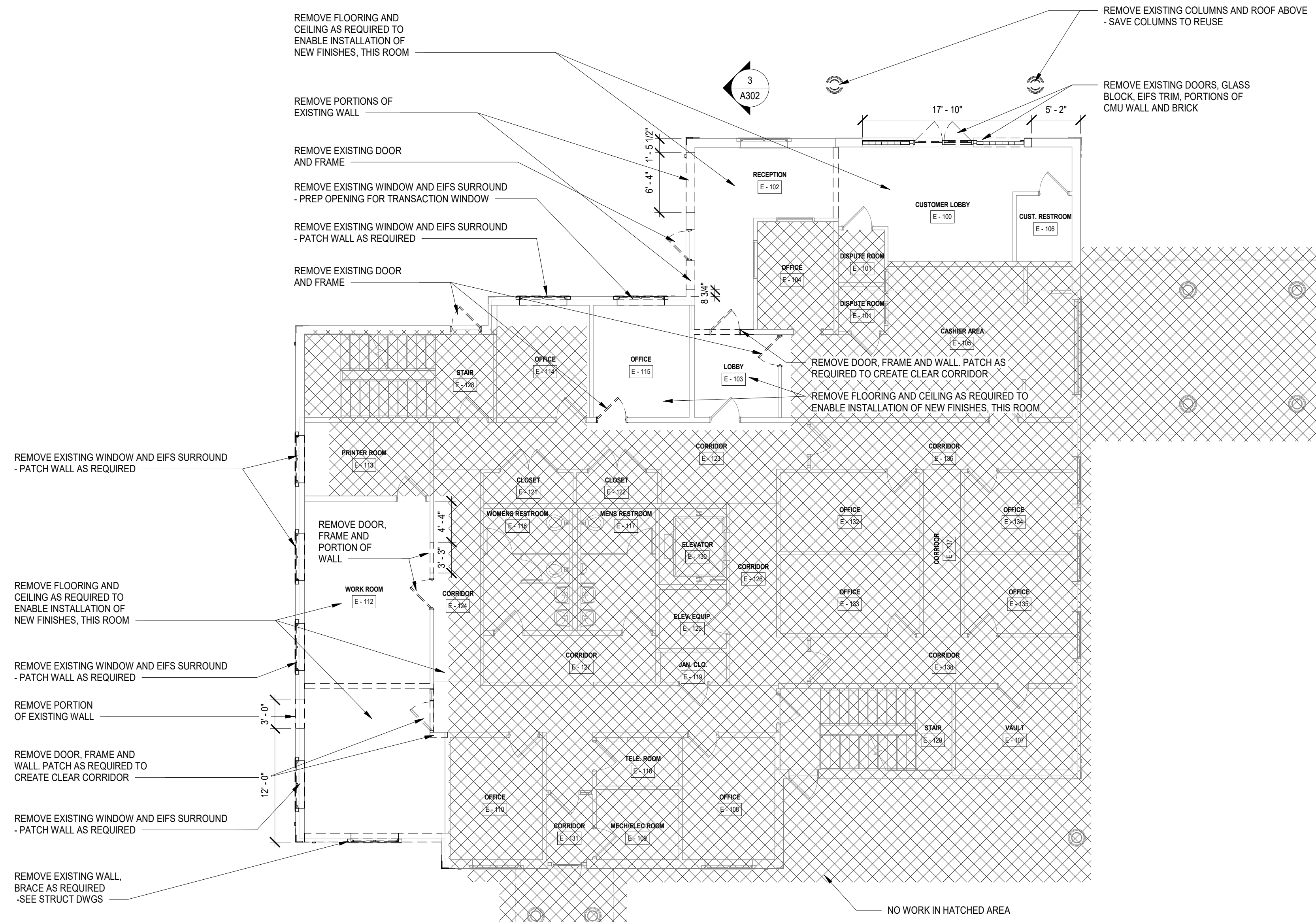
1 FIRST FLOOR DEMOLITION PLAN SCALE: 1/8" = 1'-0"
