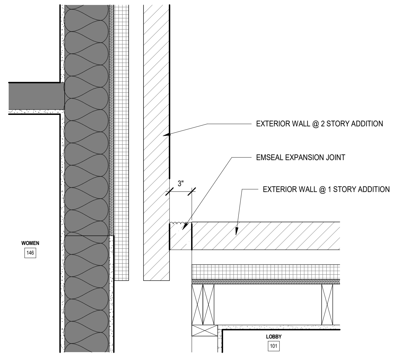
1 EXT WALL EXPANSION JOINT SCALE: 1 1/2" = 1'-0"
