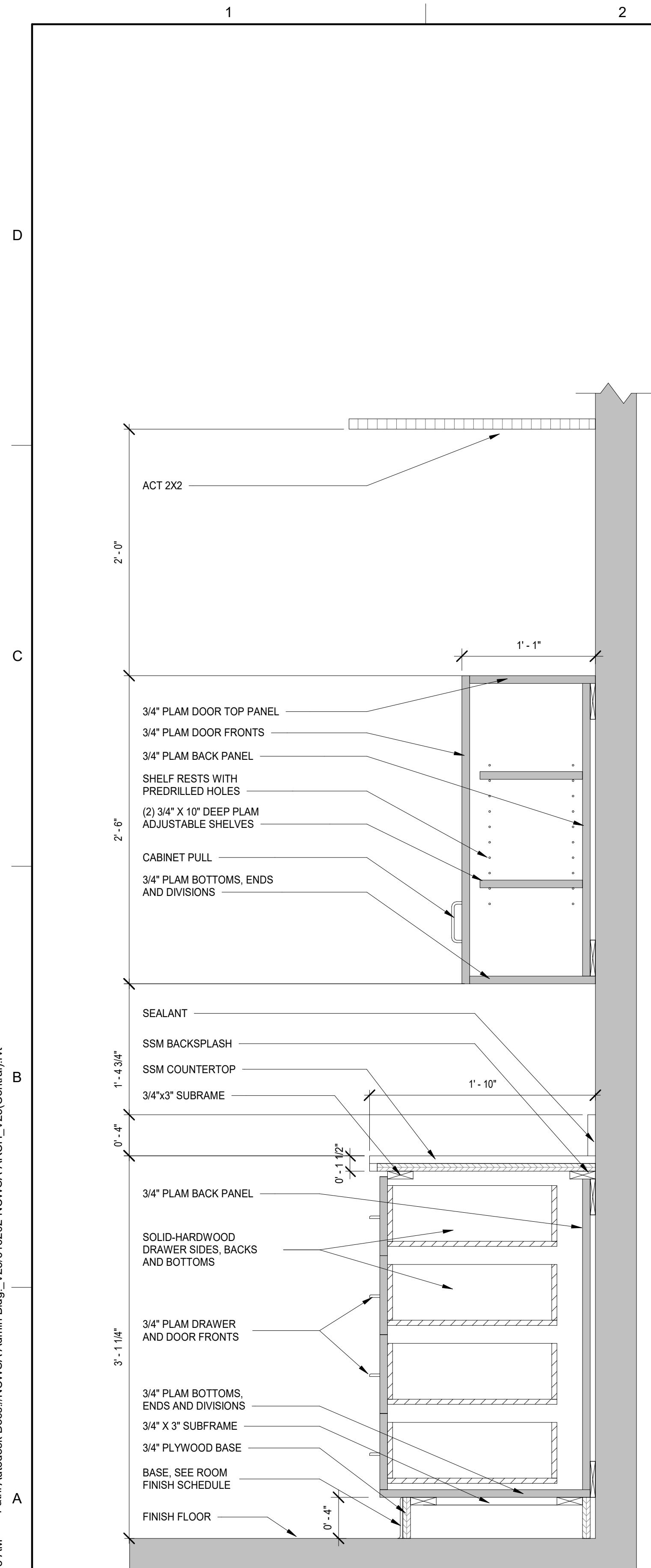
1 PRINTING AREA TOP & BOTTOM CASEWORK DETAILS SCALE: 1 1/2" = 1'-0"
