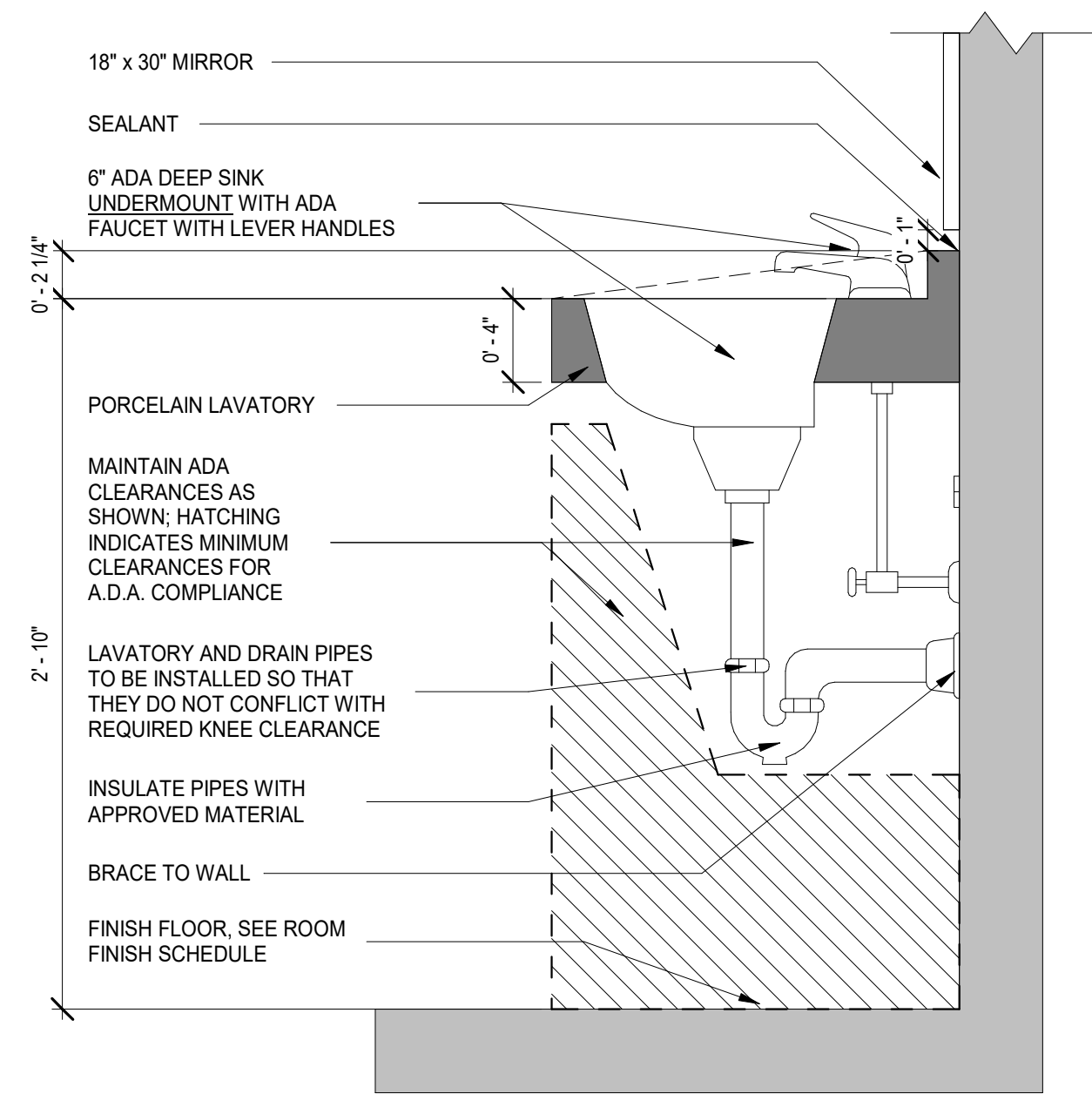
2 MILLWORK SINK DETAIL SCALE: 1 1/2" = 1'-0"
