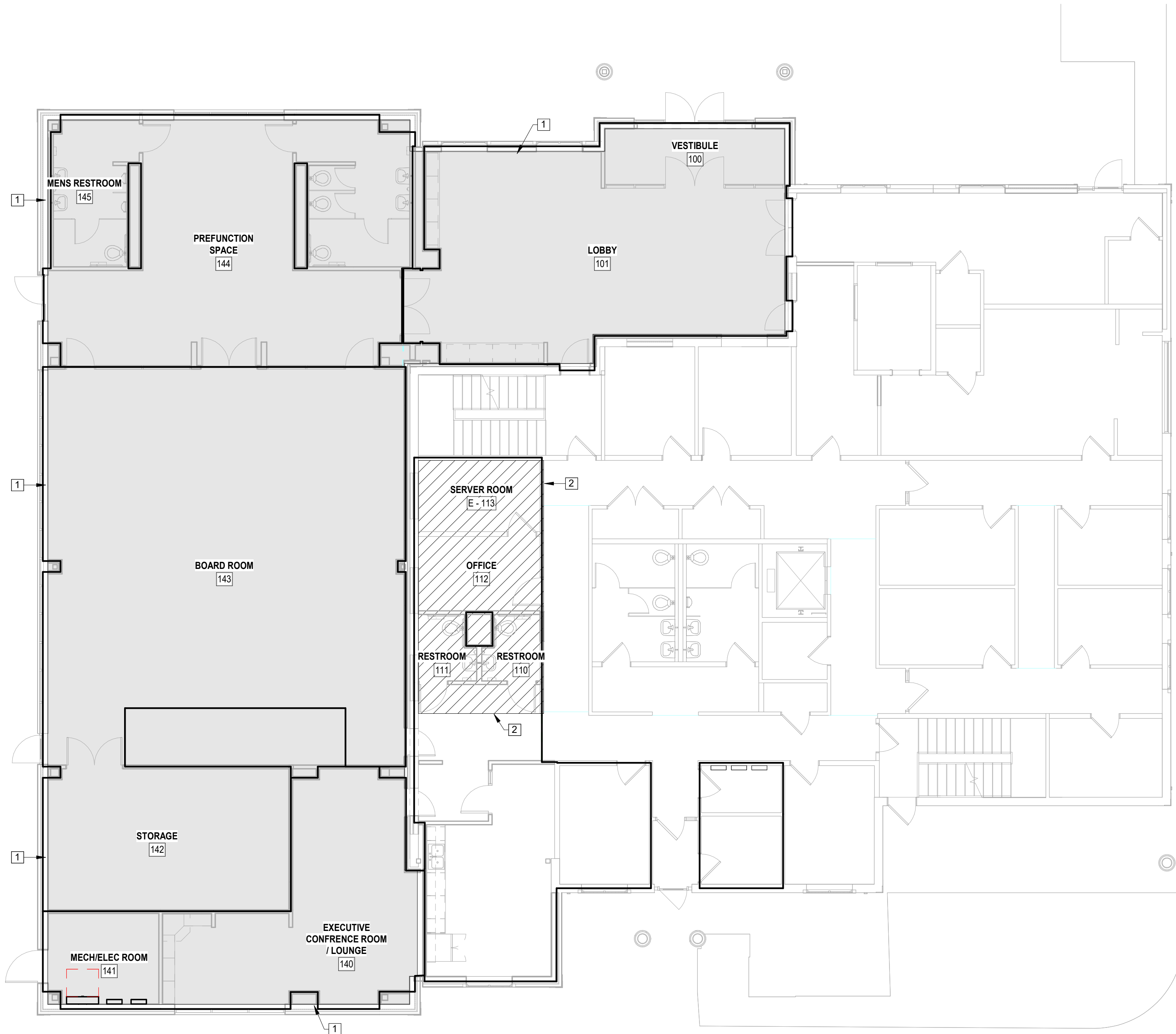
1 FIRST FLOOR FIRE PROTECTION PLAN SCALE: 1/8" = 1'-0"
