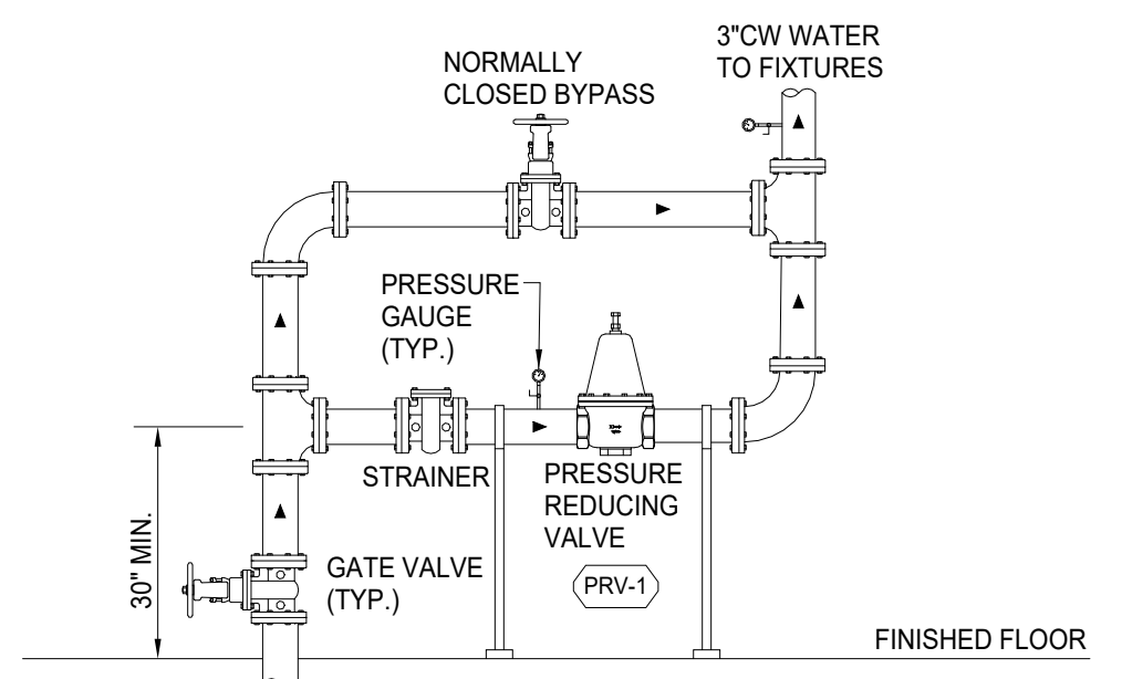
3 BUILDING WATER SERVICE DETAIL SCALE: NONE
