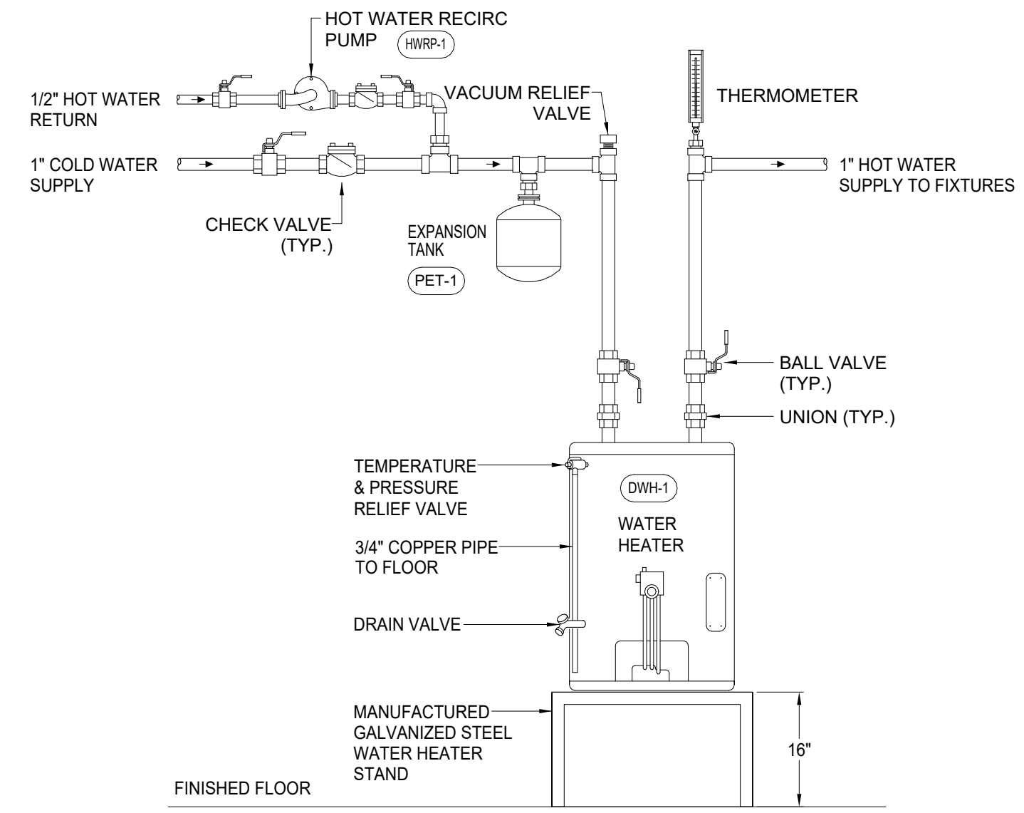
1 ELECTRIC WATER HEATER DETAIL SCALE: NONE
