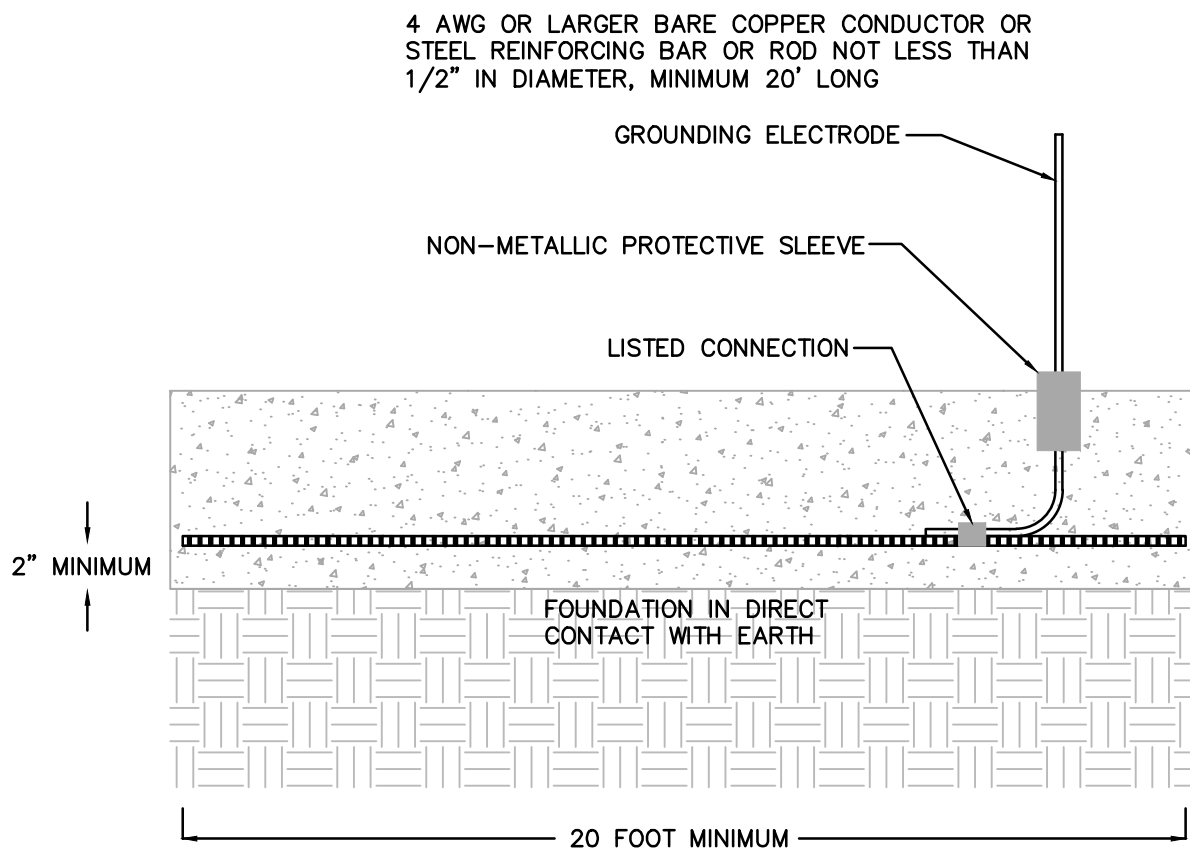
CONCRETE ENCASED ELECTRODE DETAIL
