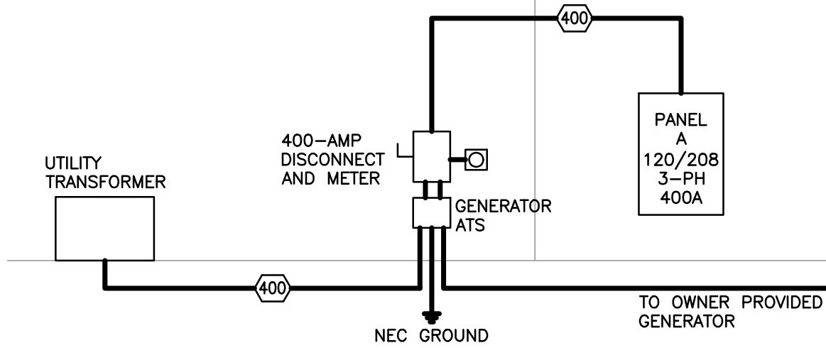
ELECTRICAL RISER DIAGRAM
