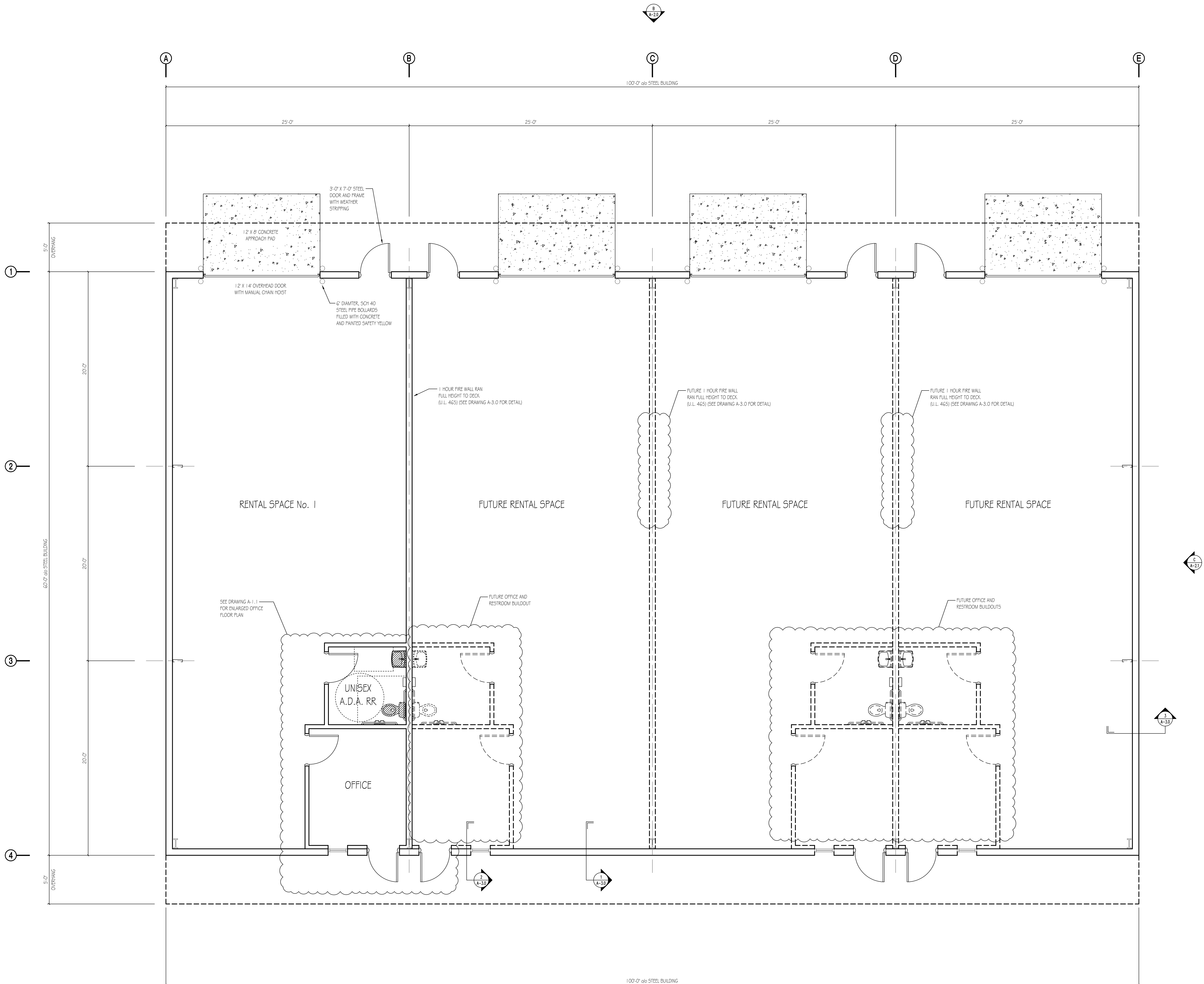
Building Floor Plan SCALE: 1/4" = 1'-0"
