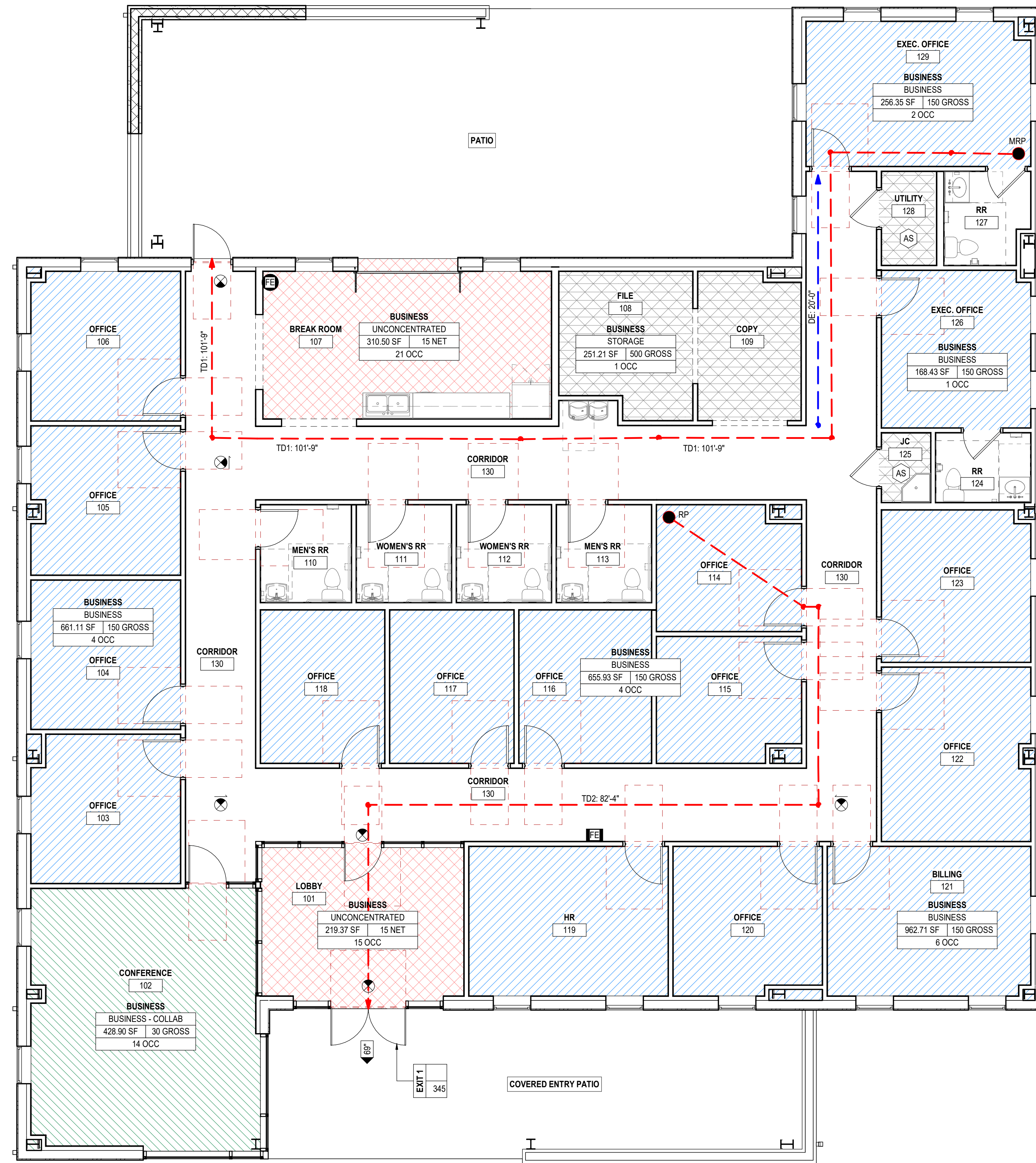
1 LIFE SAFETY PLAN LS101 | 3/16" = 1'-0"
