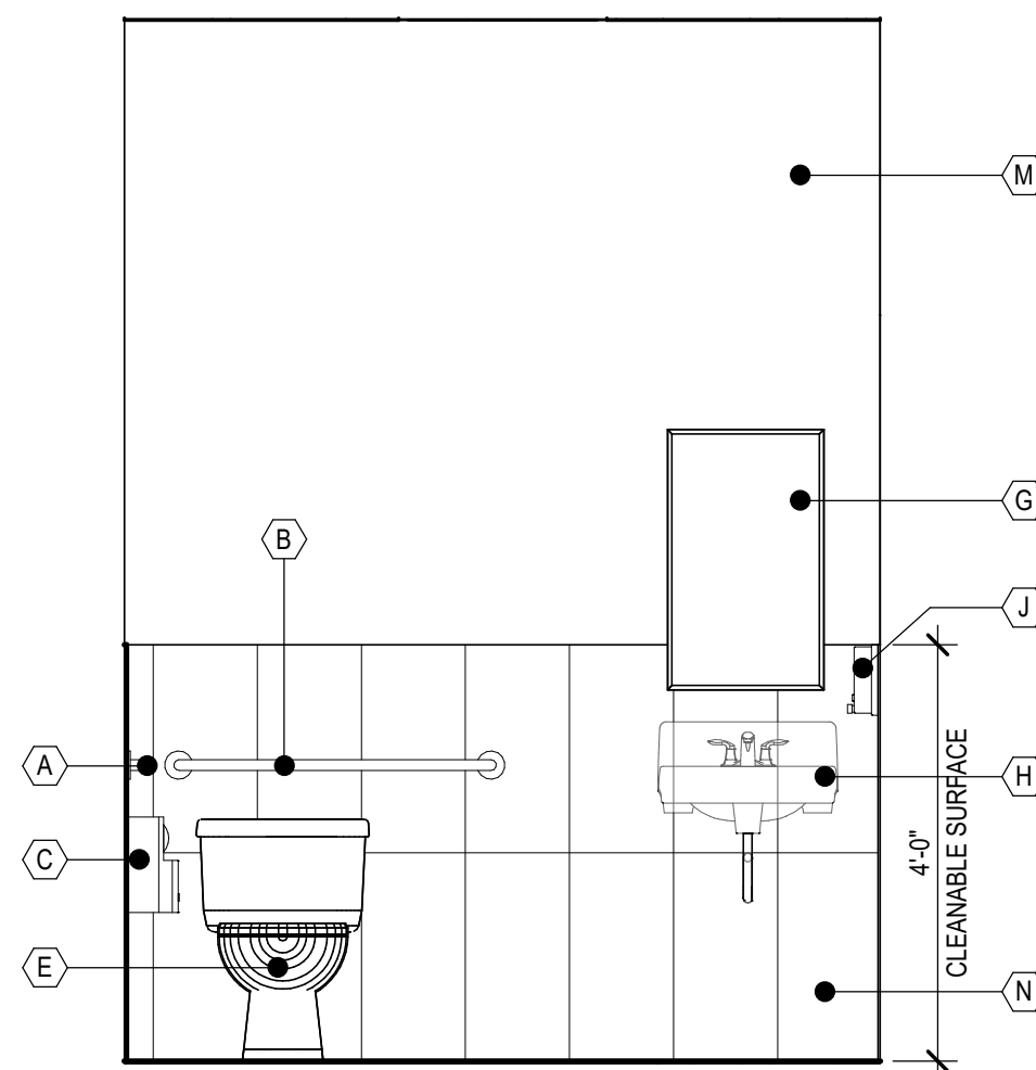
2 RR 110 - ELEVATION 2 A-505 | 1/2" = 1'-0"
