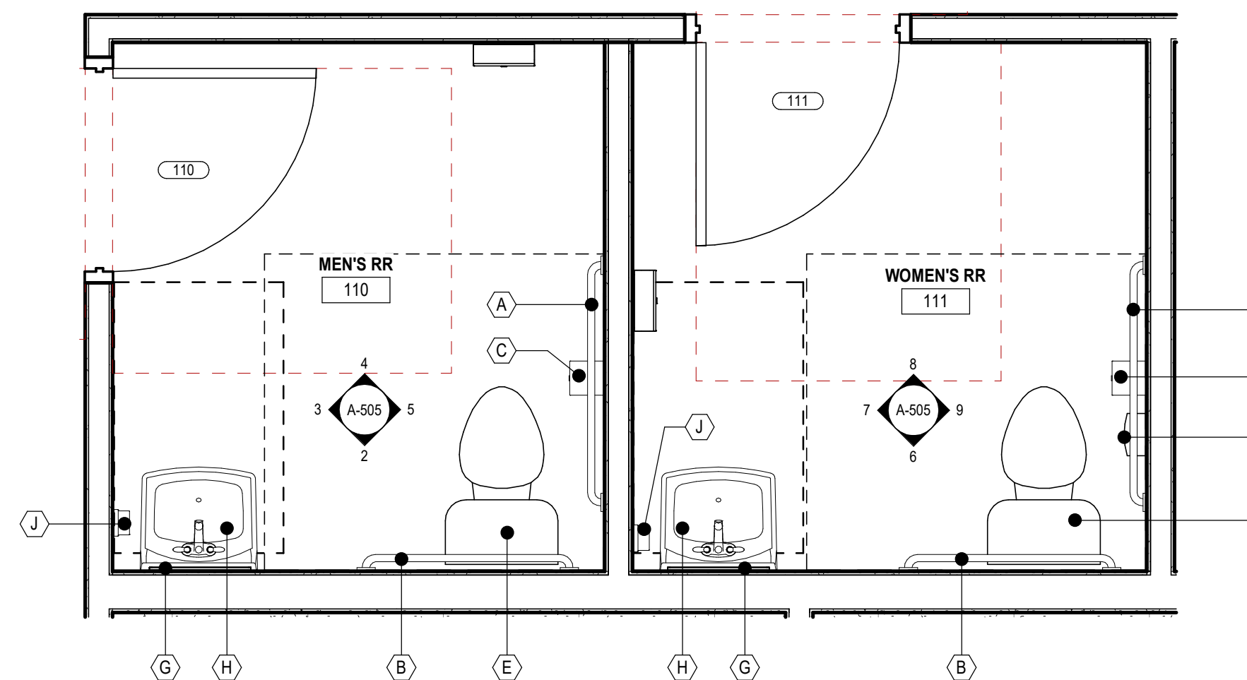
1 TYP. ENLARGED RESTROOM FLOOR PLANS A-505 | 1/2" = 1'-0"
