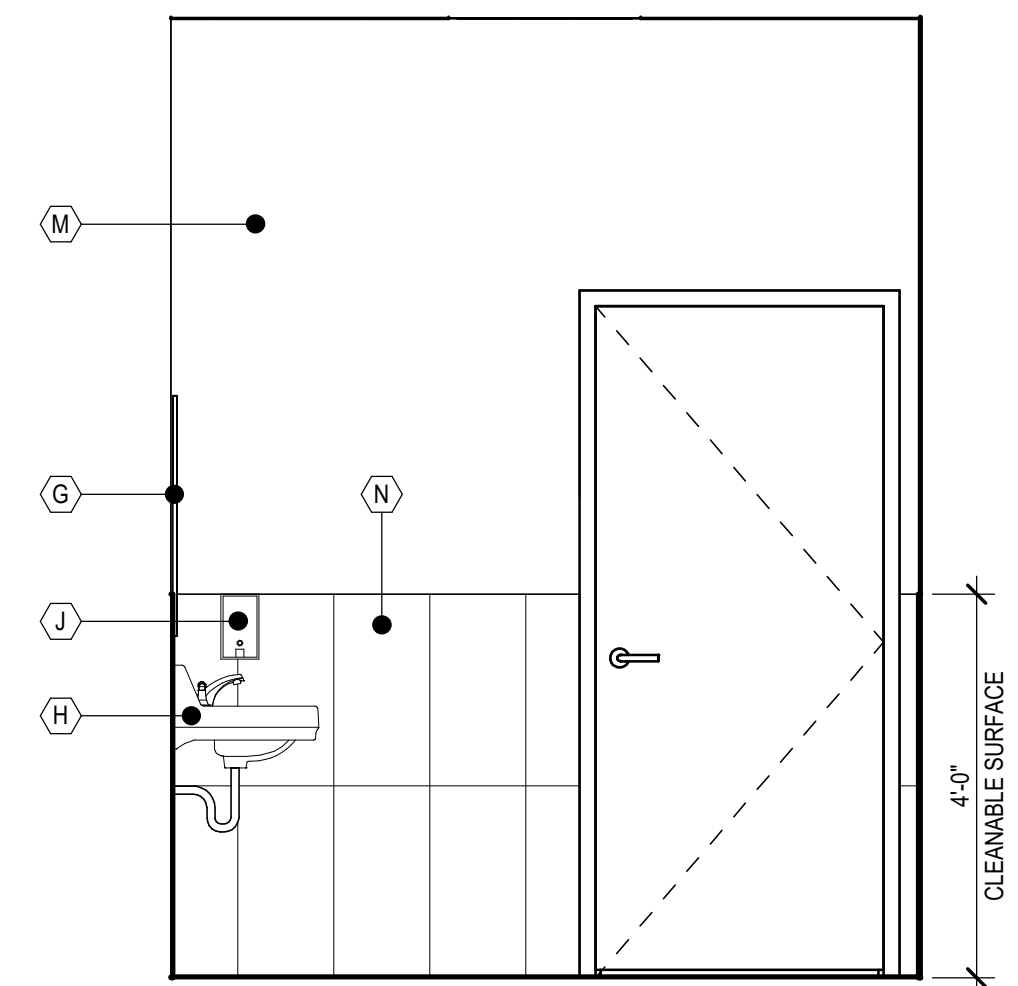
3 RR 110 - ELEVATION 3 A-505 | 1/2" = 1'-0"
