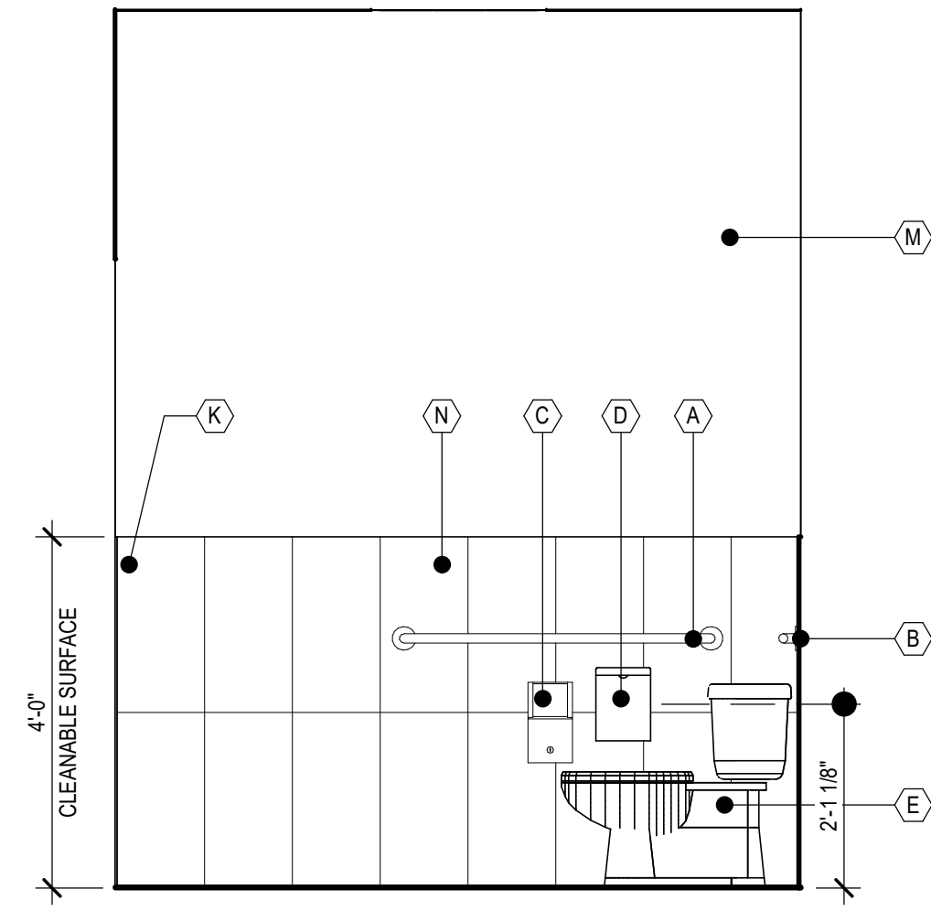
9 RR 111 - ELEVATION 9 A-505 | 1/2" = 1'-0"
