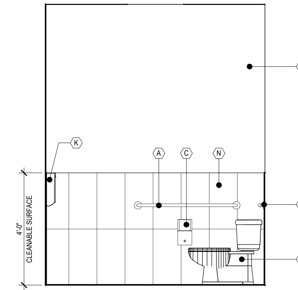
5 RR 110 - ELEVATION 5 A-505 | 1/2" = 1'-0"
