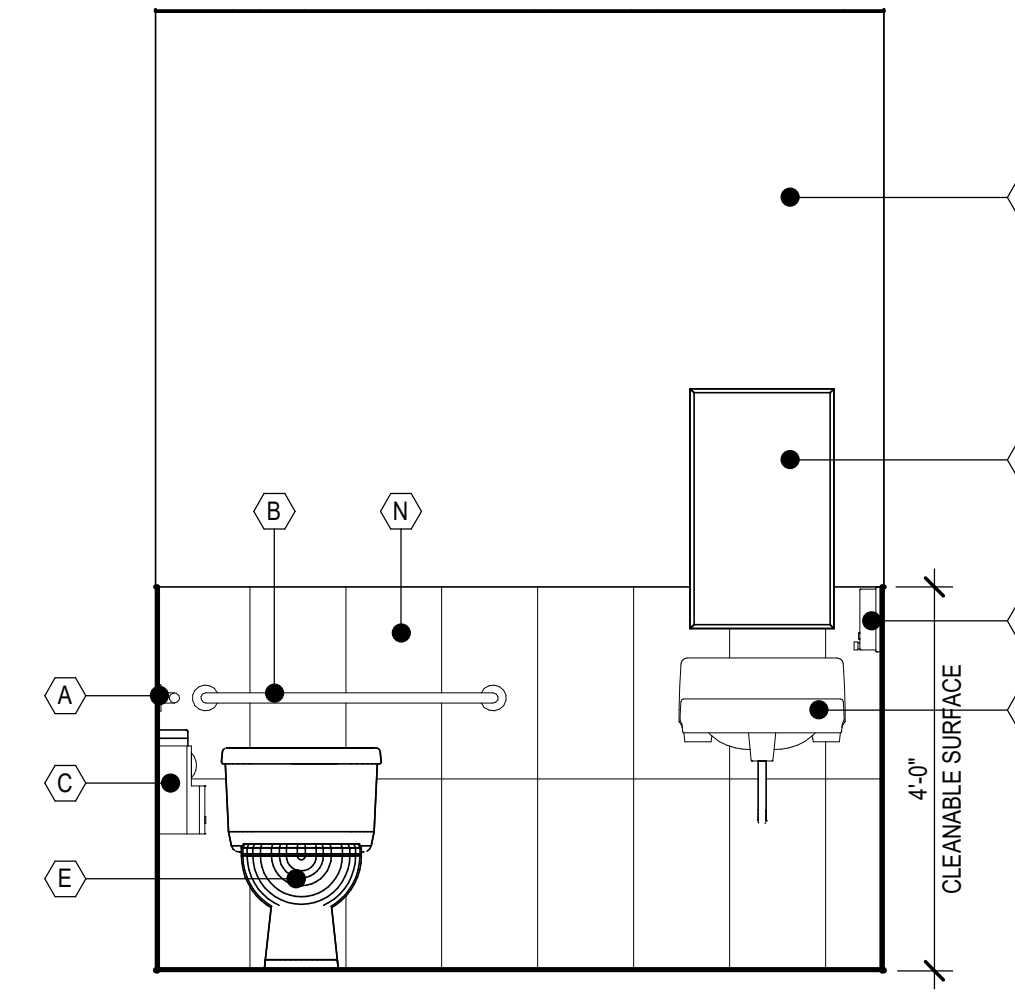
6 RR 111 - ELEVATION 6 A-505 | 1/2" = 1'-0"
