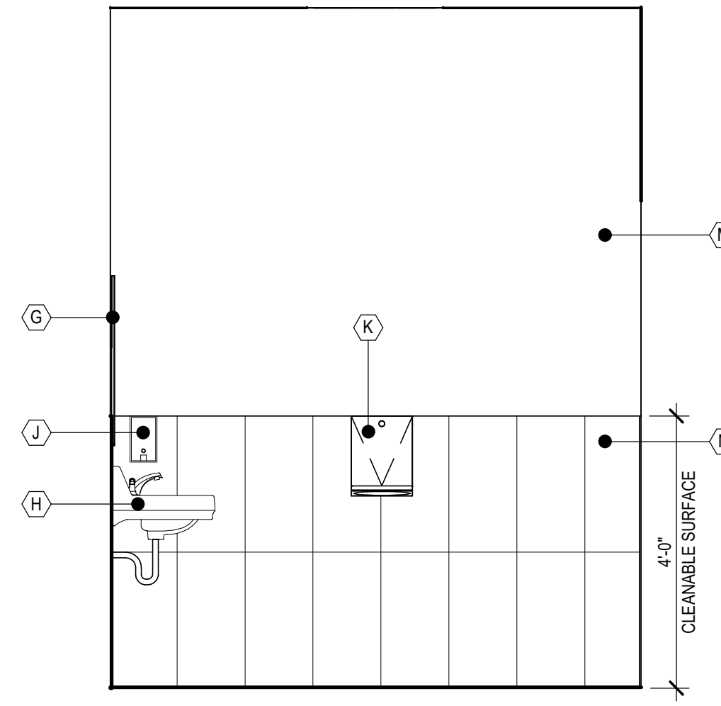
7 RR 111 - ELEVATION 7 A-505 | 1/2" = 1'-0"
