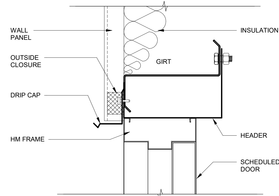
2 MTL. PANEL HEAD A-802 | 3" = 1'-0"
