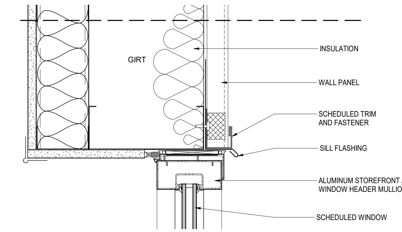
7 WINDOW HEADER - METAL WALL PANEL A-802 | 3" = 1'-0"
