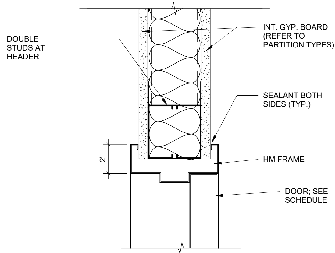
1 HM TYP. DETAIL A-802 | 3" = 1'-0"
