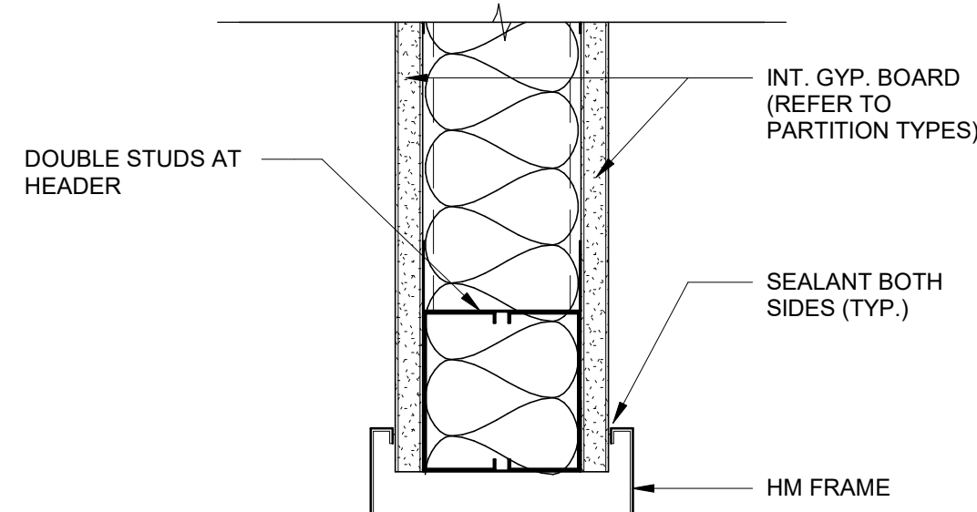
5 HM CASSED HEAD A-802 | 3" = 1'-0"
