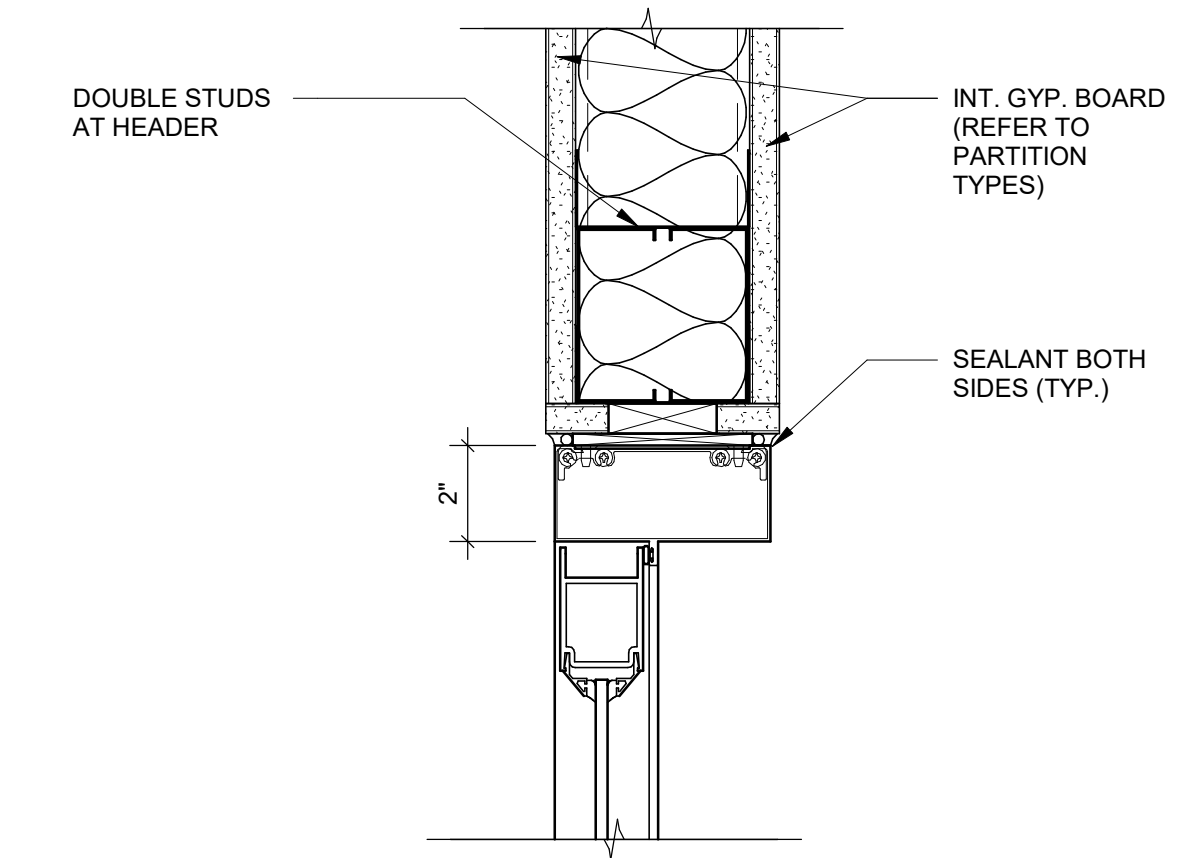
4 ALUM. DOOR INT. HEAD A-802 | 3" = 1'-0"
