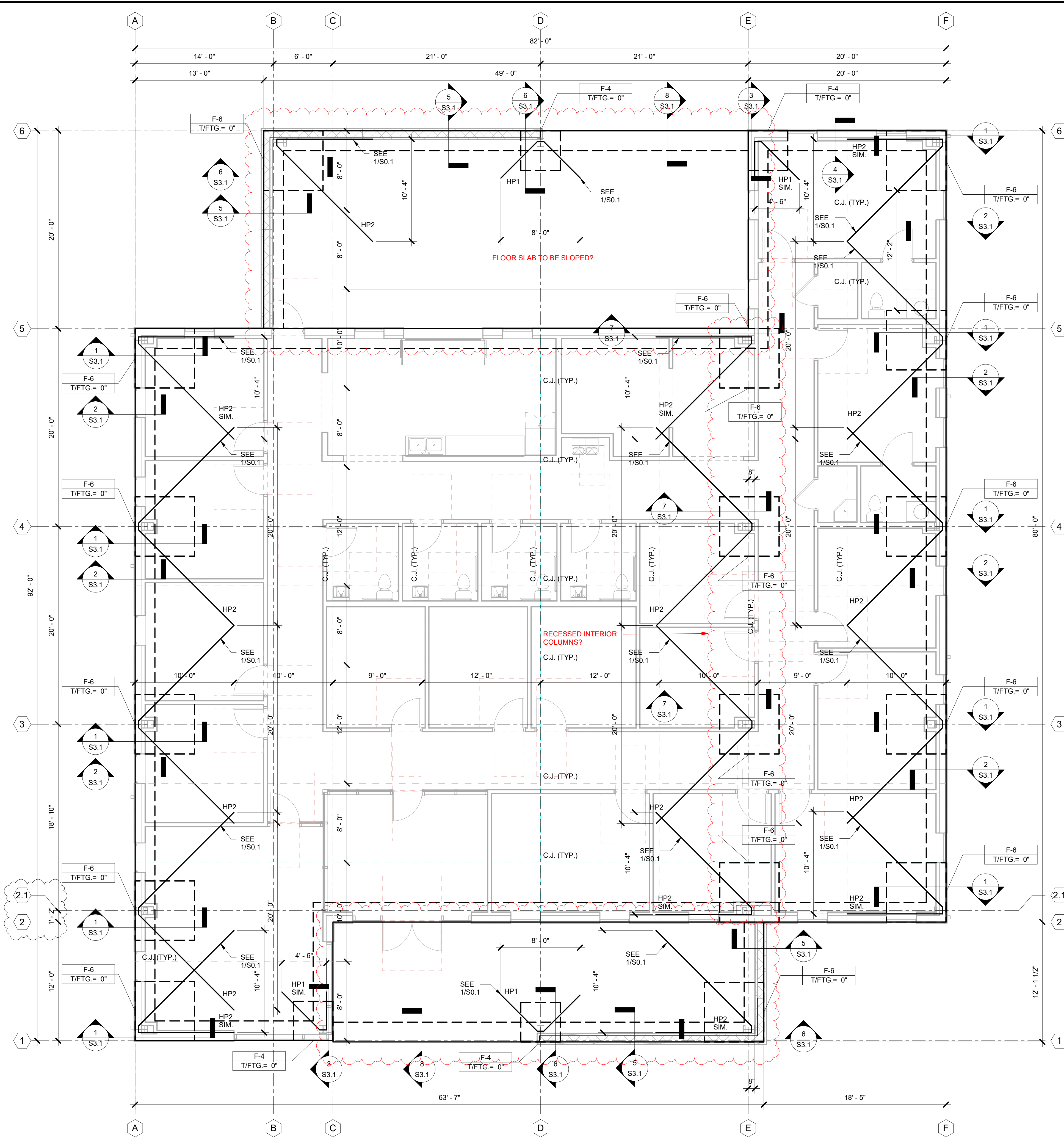
1 Foundation Plan S1.1 3/16" = 1'-0"
