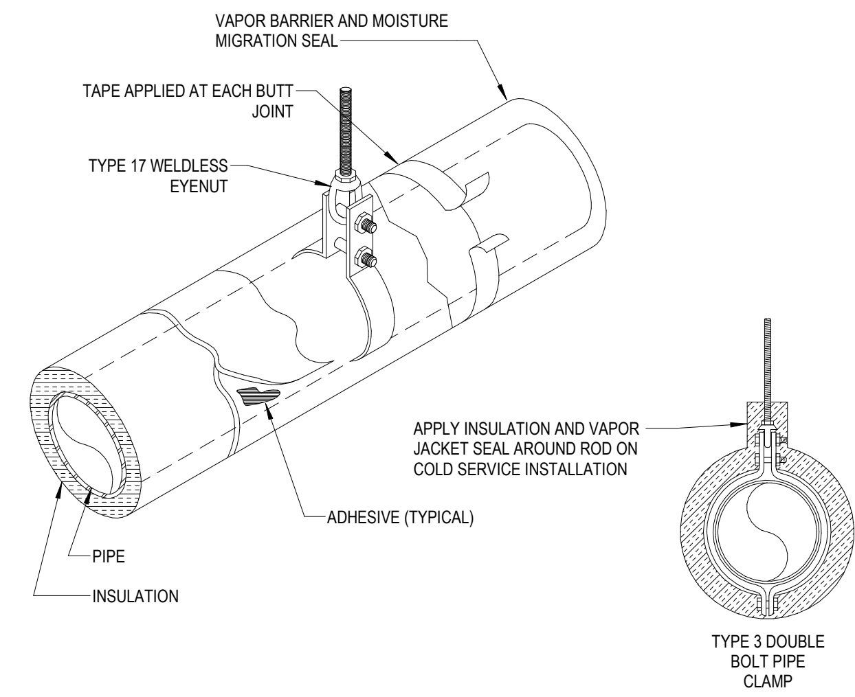
2 PIPE HANGER, INSULATION AND VAPOR JACKET M0.5 NOT TO SCALE
