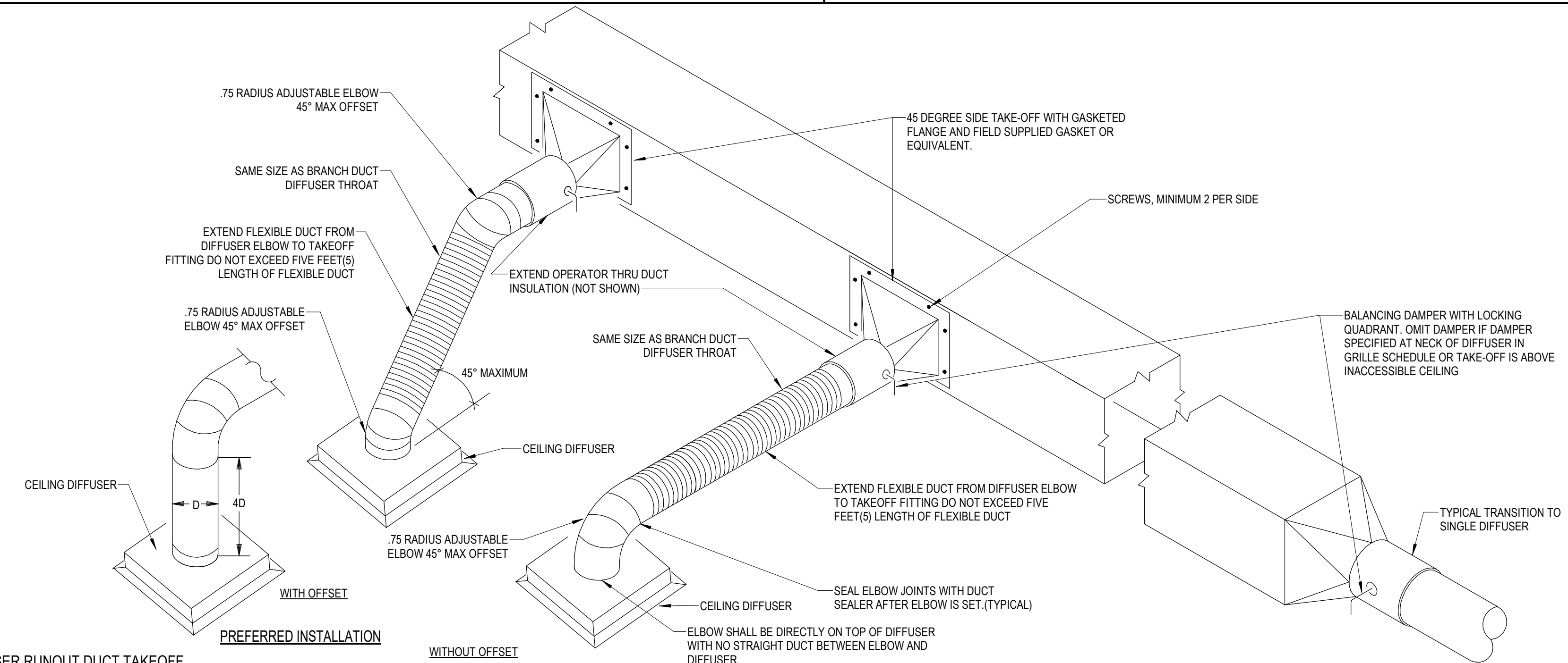
6 DIFFUSER RUNOUT DUCT TAKEOFF M0.5 NOT TO SCALE
