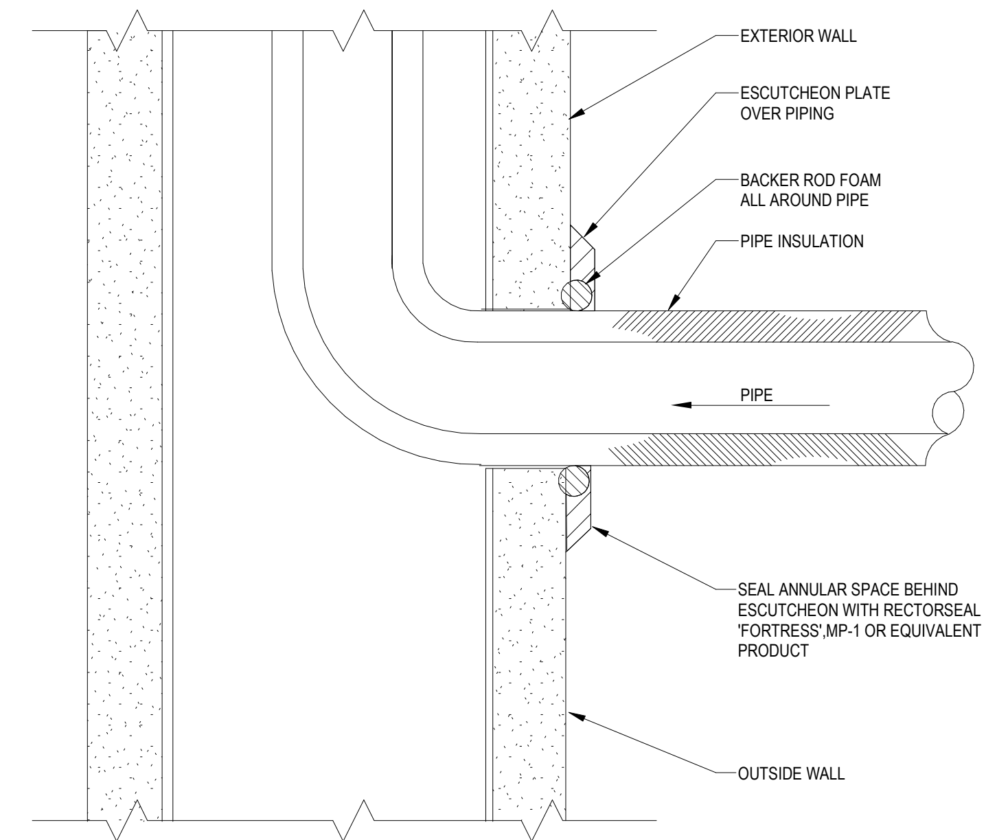
3 REFRIGERANT PIPE SLEEVE THROUGH WALL DETAIL M0.5 NOT TO SCALE
