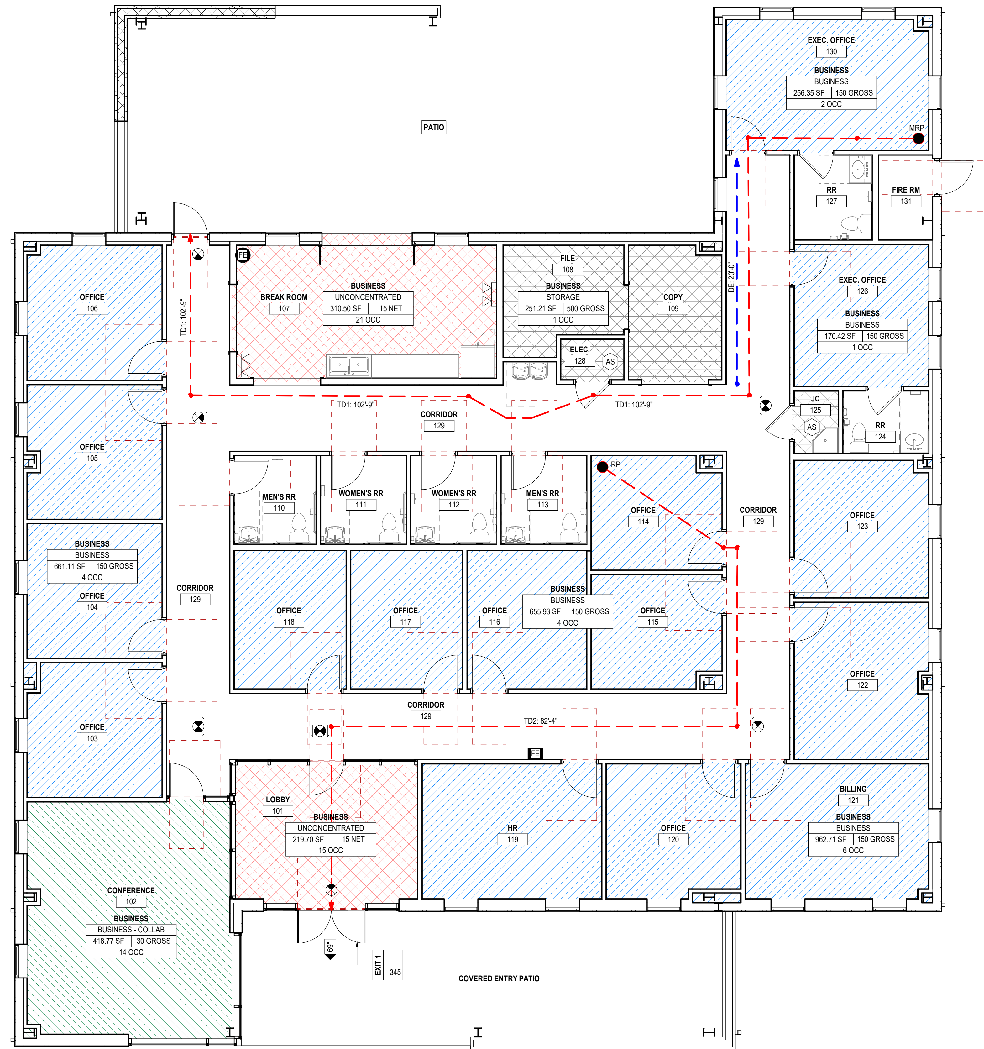
1 LIFE SAFETY PLAN LS101 | 3/16" = 1'-0"
