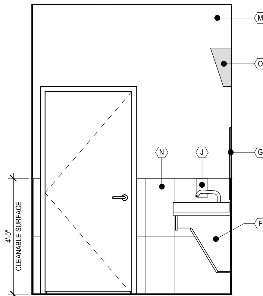
4 RR 127 - ELEVATION 4 A-506 | 1/2" = 1'-0"
