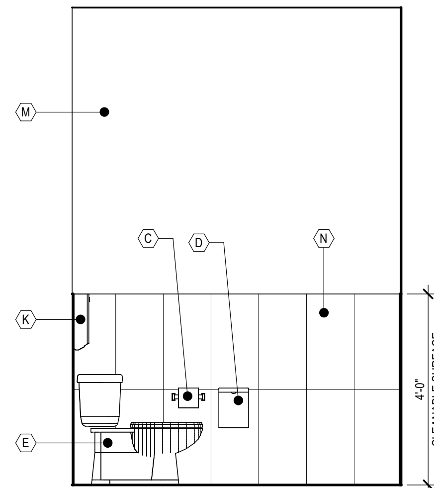
2 RR 127 - ELEVATION 2 A-506 | 1/2" = 1'-0"
