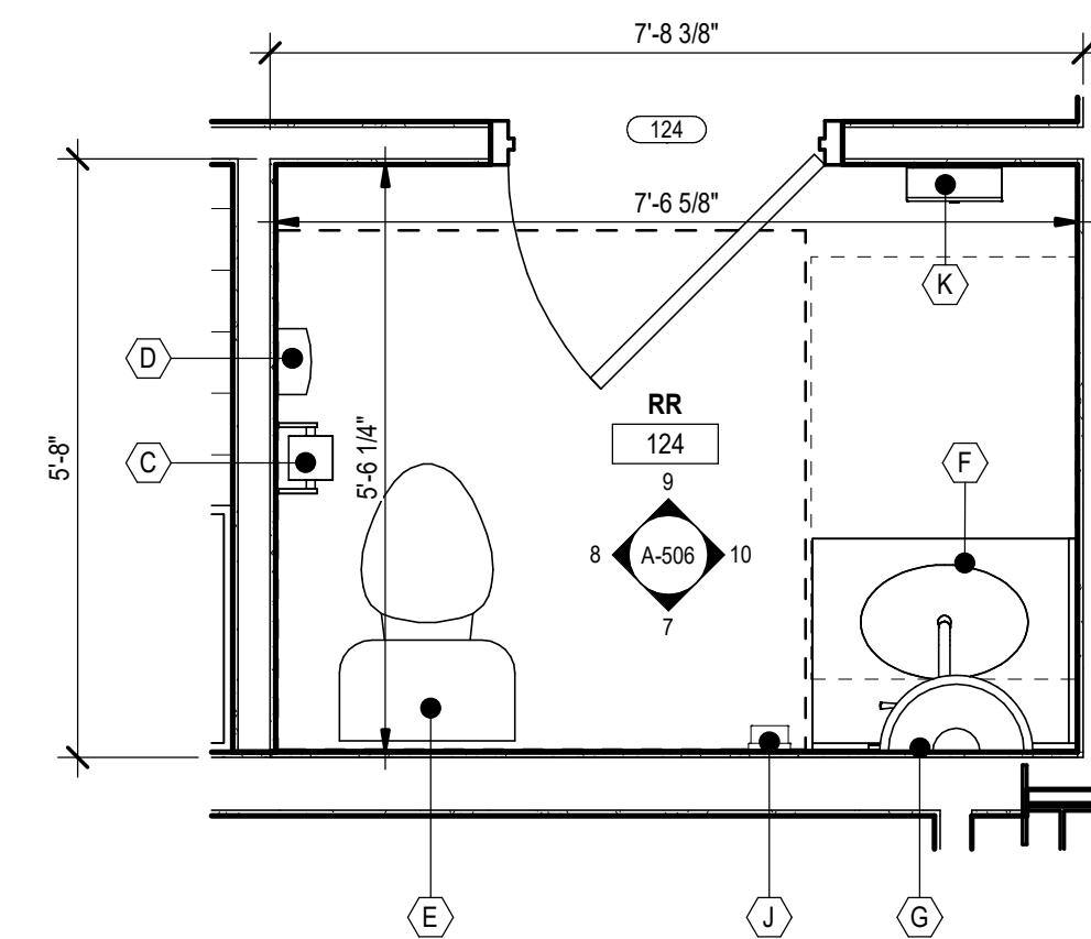
6 ENLARGED RR 124 FLOOR PLAN A-506 | 1/2" = 1'-0"
