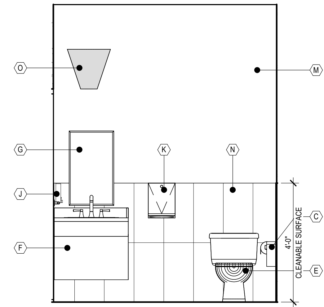
5 RR 127 - ELEVATION 5 A-506 | 1/2" = 1'-0"
