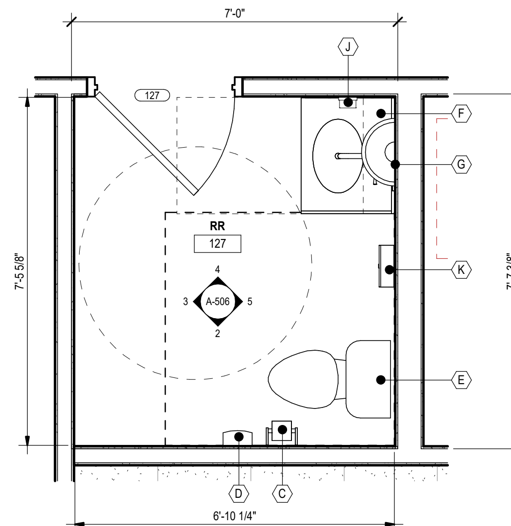
1 ENLARGED RR 127 FLOOR PLAN A-506 | 1/2" = 1'-0"
