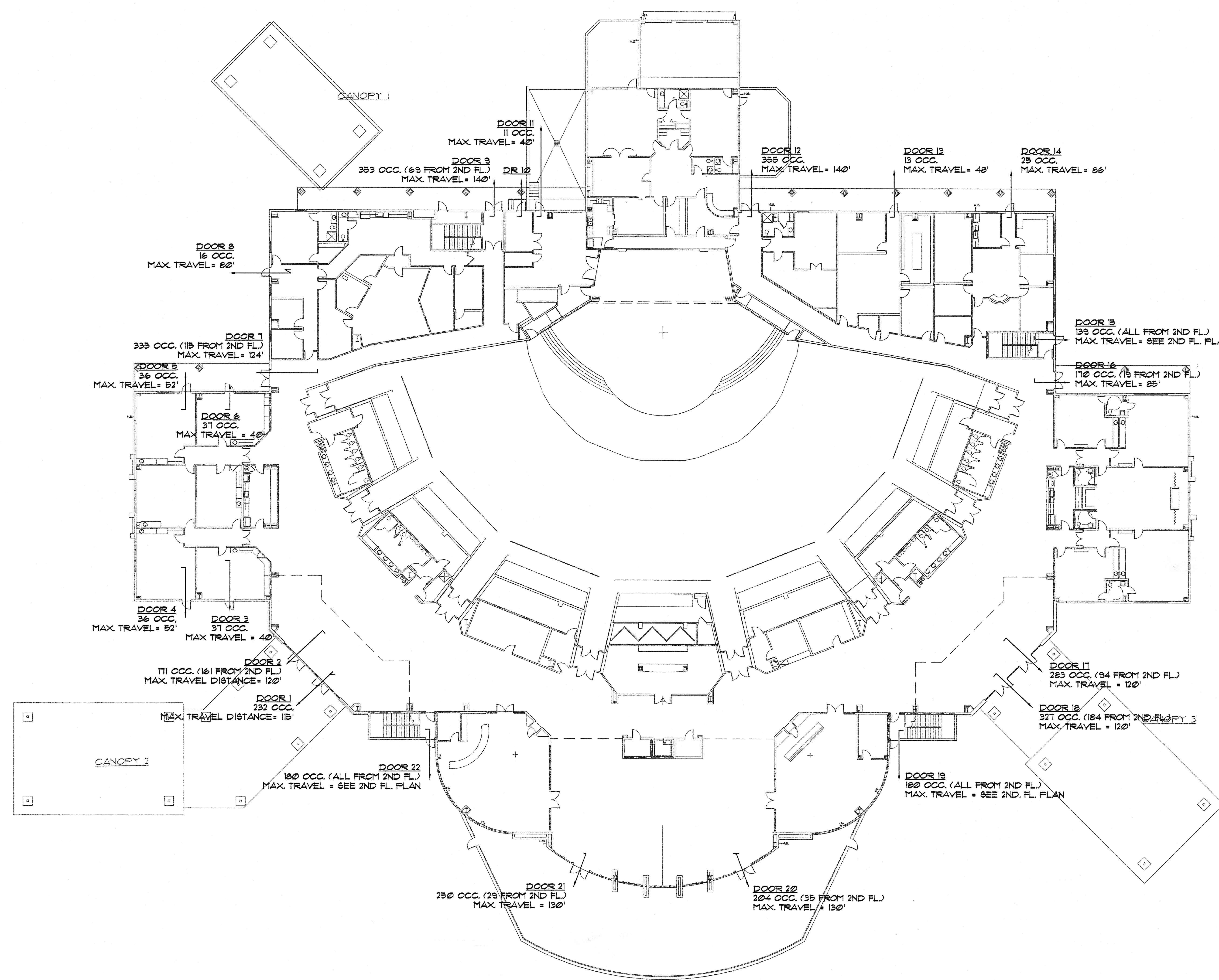
EGRESS / EXIT PLAN - FIRST FLOOR 1/16" = 1'-0" PLAN NORTH
