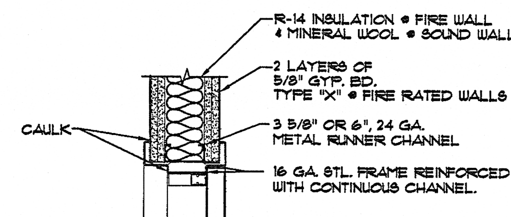
17 SOUND INSULATED DOOR HEAD DETAIL SCALE: 1 1/2\"/>
