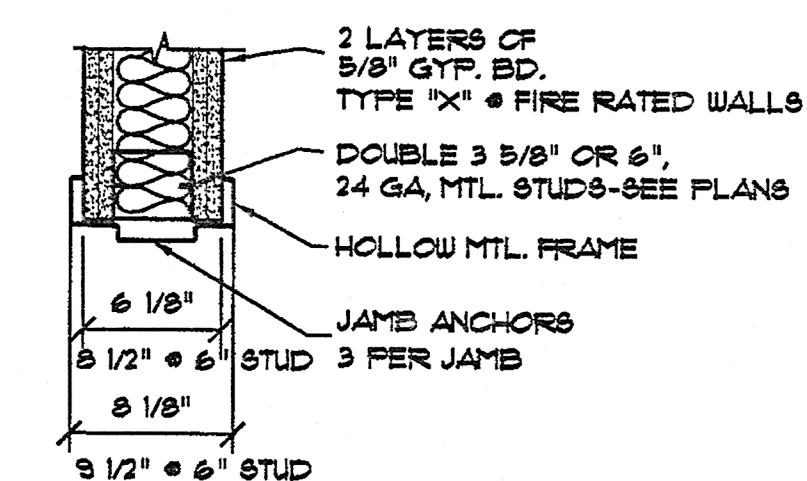
18 SOUND INSULATED DOOR JAMB DETAIL SCALE: 1 1/2\"/>
