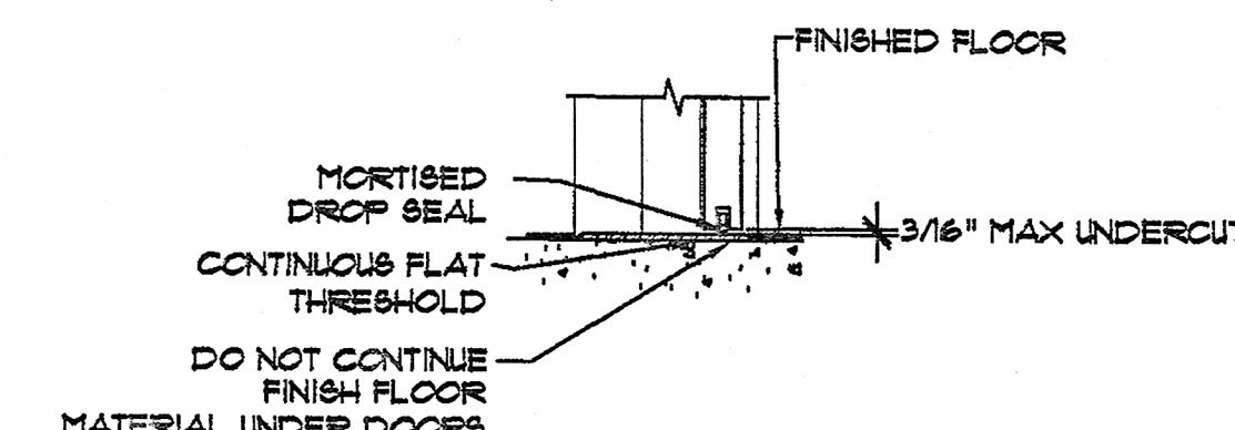
19 SOUND INSULATED DOOR SILL SECTION SCALE: 1 1/2\"/>
