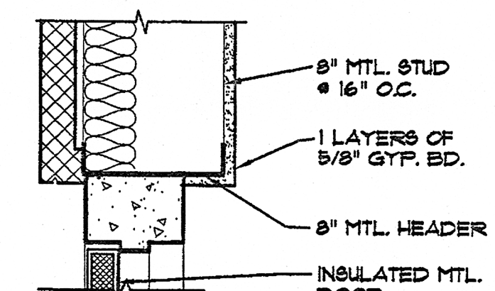
23 DOOR HEAD DETAIL SCALE: 1 1/2\"/>
