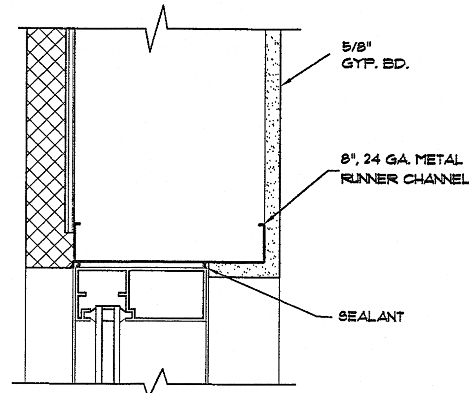
1 STOREFRONT HEAD DETAIL SCALE: 3\"/>
