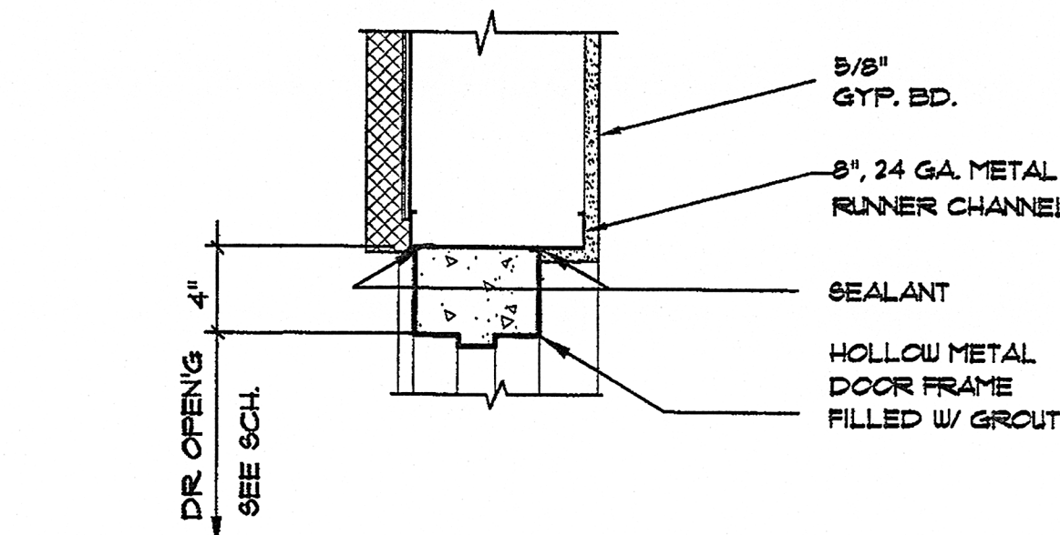
11 DOOR HEAD DETAIL SCALE: 1 1/2\"/>
