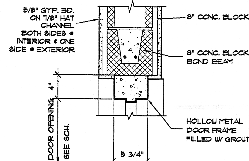
11 DOOR HEAD DETAIL SCALE: 1 1/2\"/>
