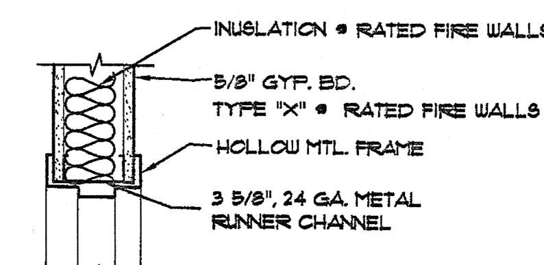
20 DOOR HEAD DETAIL SCALE: 1 1/2\"/>
