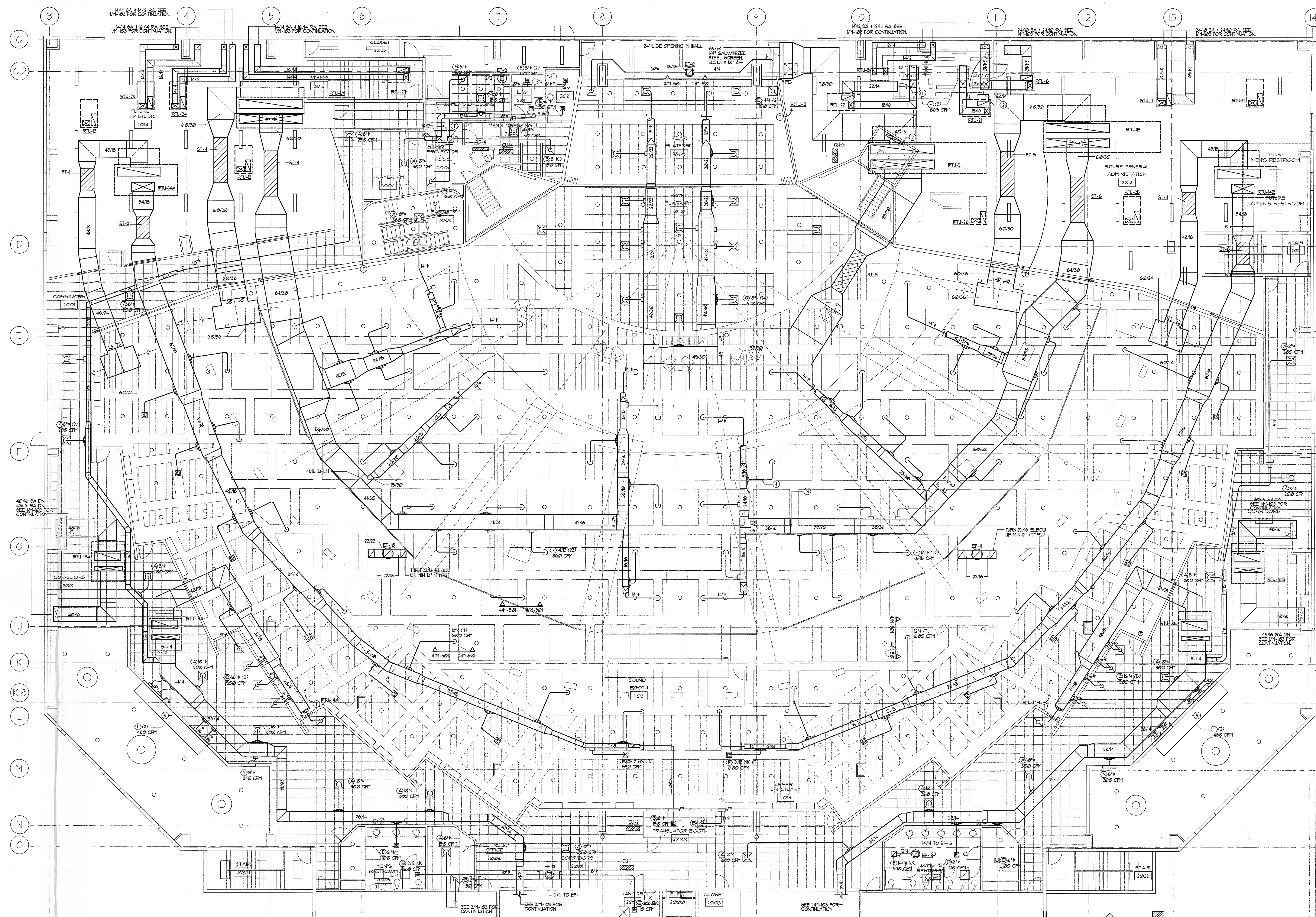
PLAN NORTH 1 PARTIAL 2nd FLOOR PLAN - HVAC SCALE: 1/8" = 1'-0"
