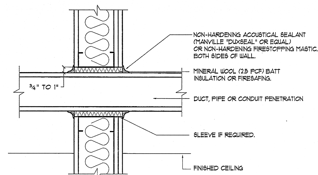
PENETRATION ABOVE FINISHED CEILING
