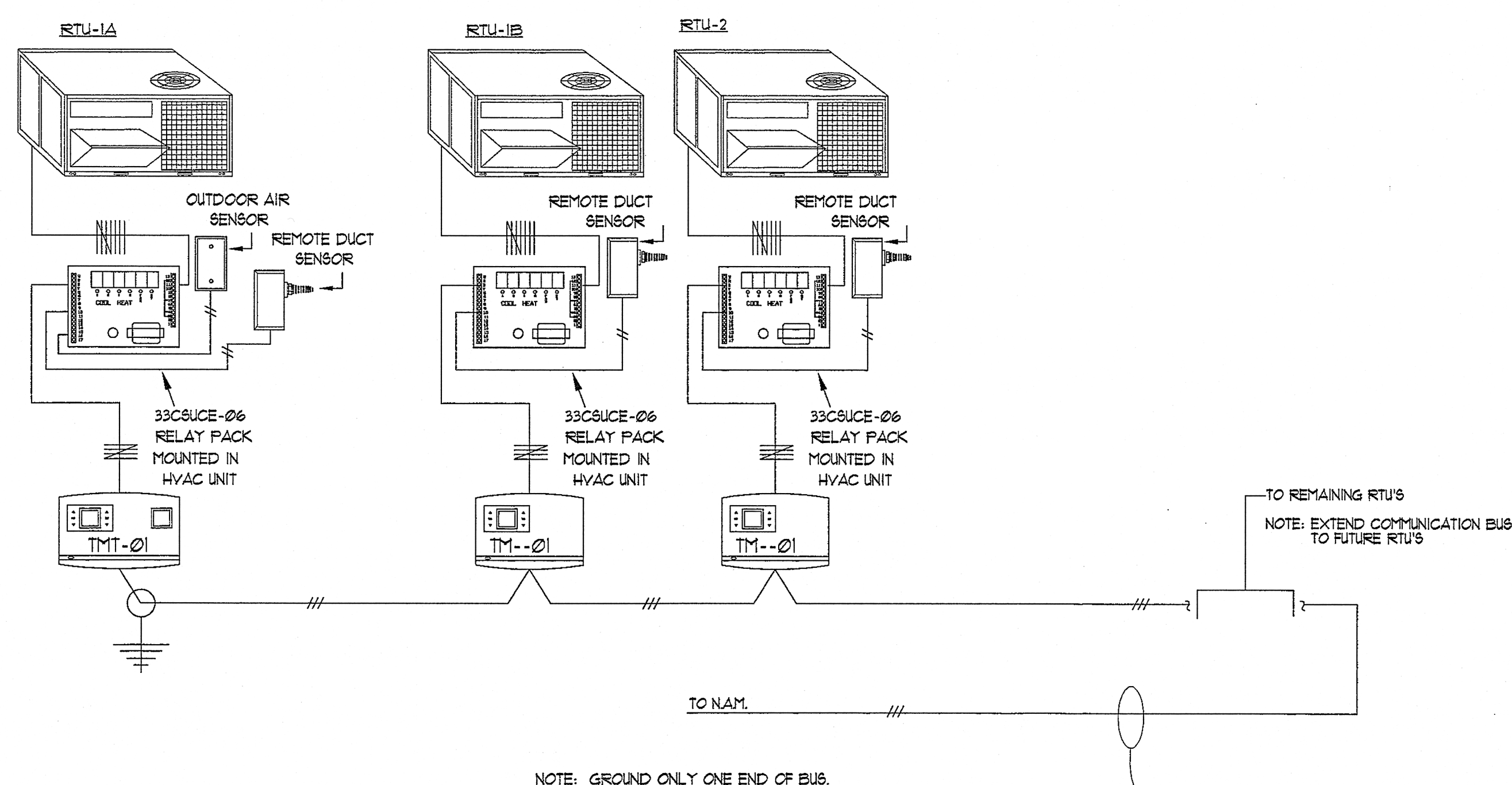
9 TYPICAL TEMP SYSTEM M-501
