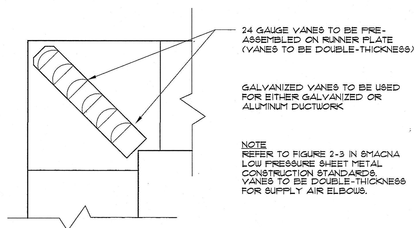
5 SQUARE ELBOW - DETAIL M-501 SCALE : NONE
