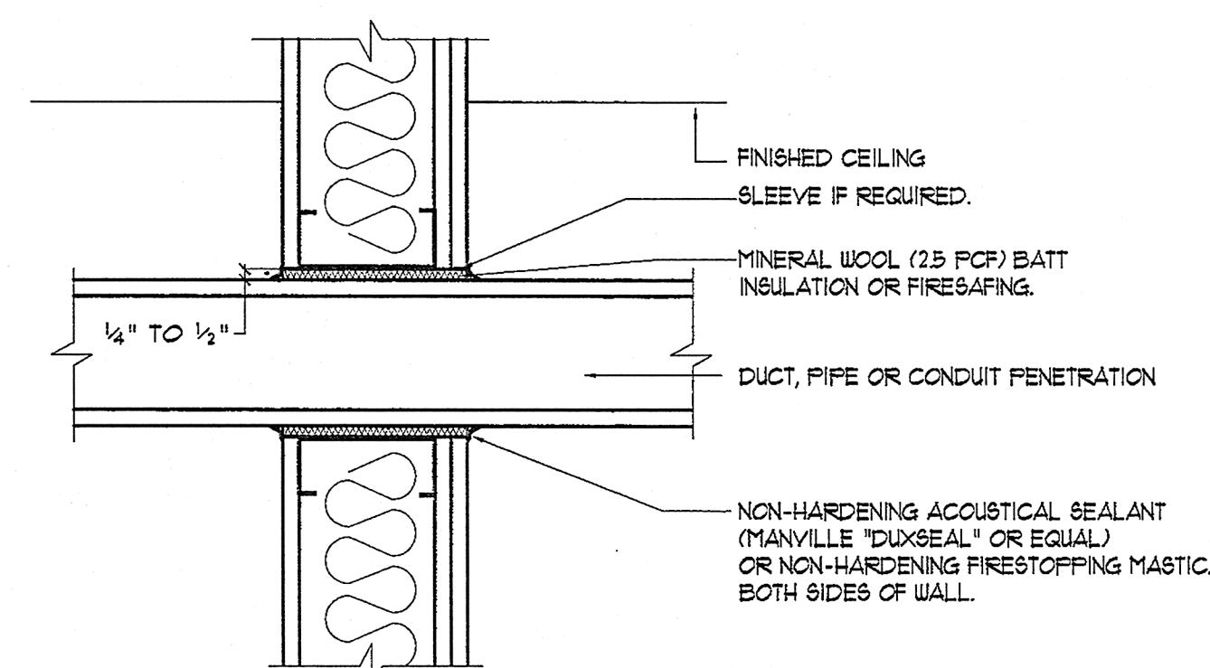
PENETRATION BELOW FINISHED CEILING
