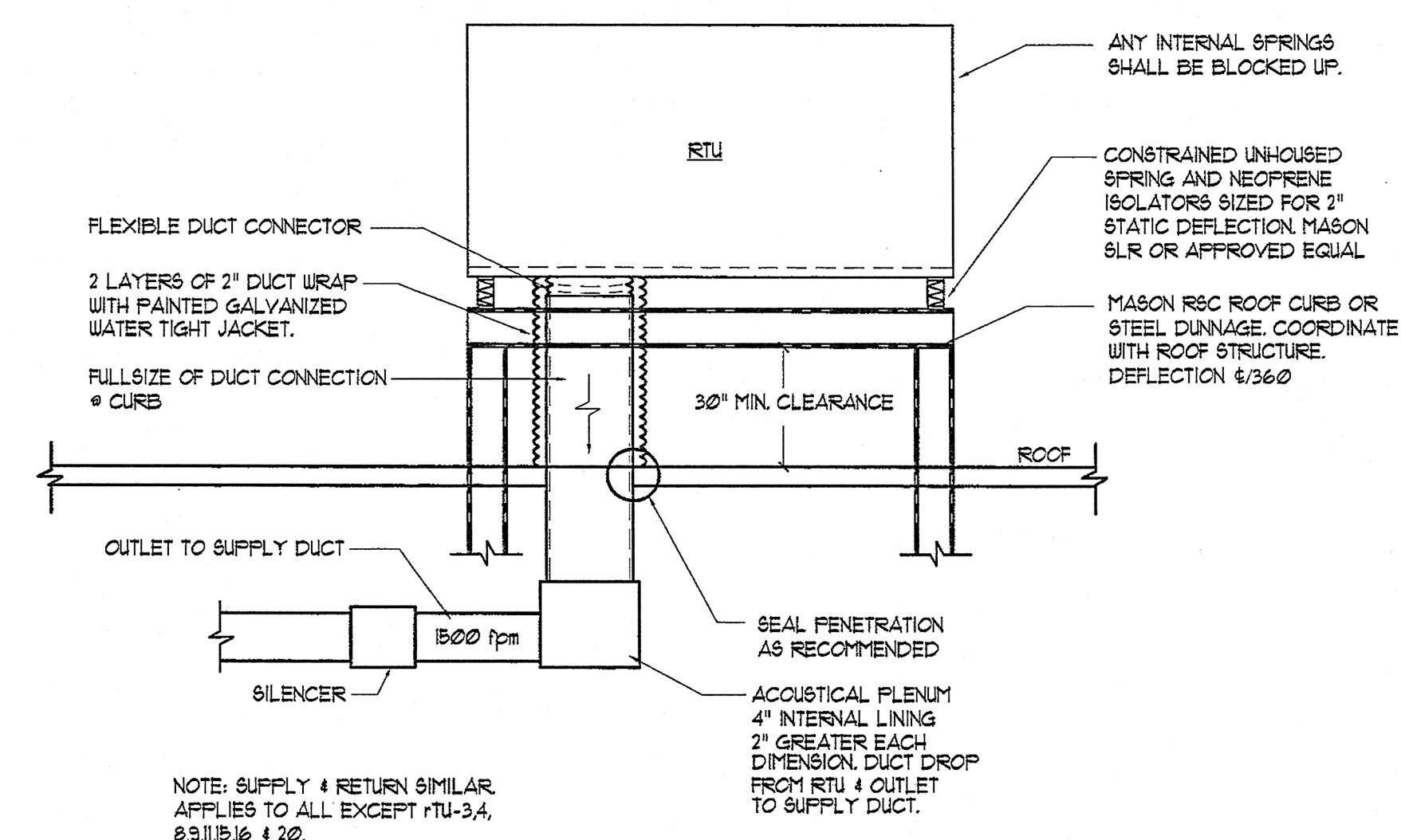
8 ROOFTOP UNIT MOUNTING AND ACOUSTIC PLENUMS - SCHEMATIC M-501 NONE
