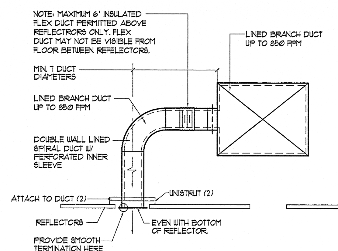
2 DETAIL M-501 NONE
