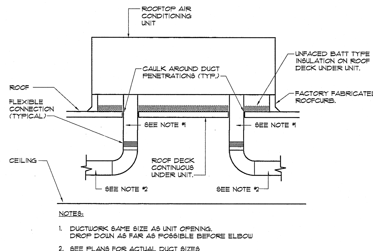
7 ROOFTOP A/C UNIT - DETAIL M-501 SCALE : NONE
