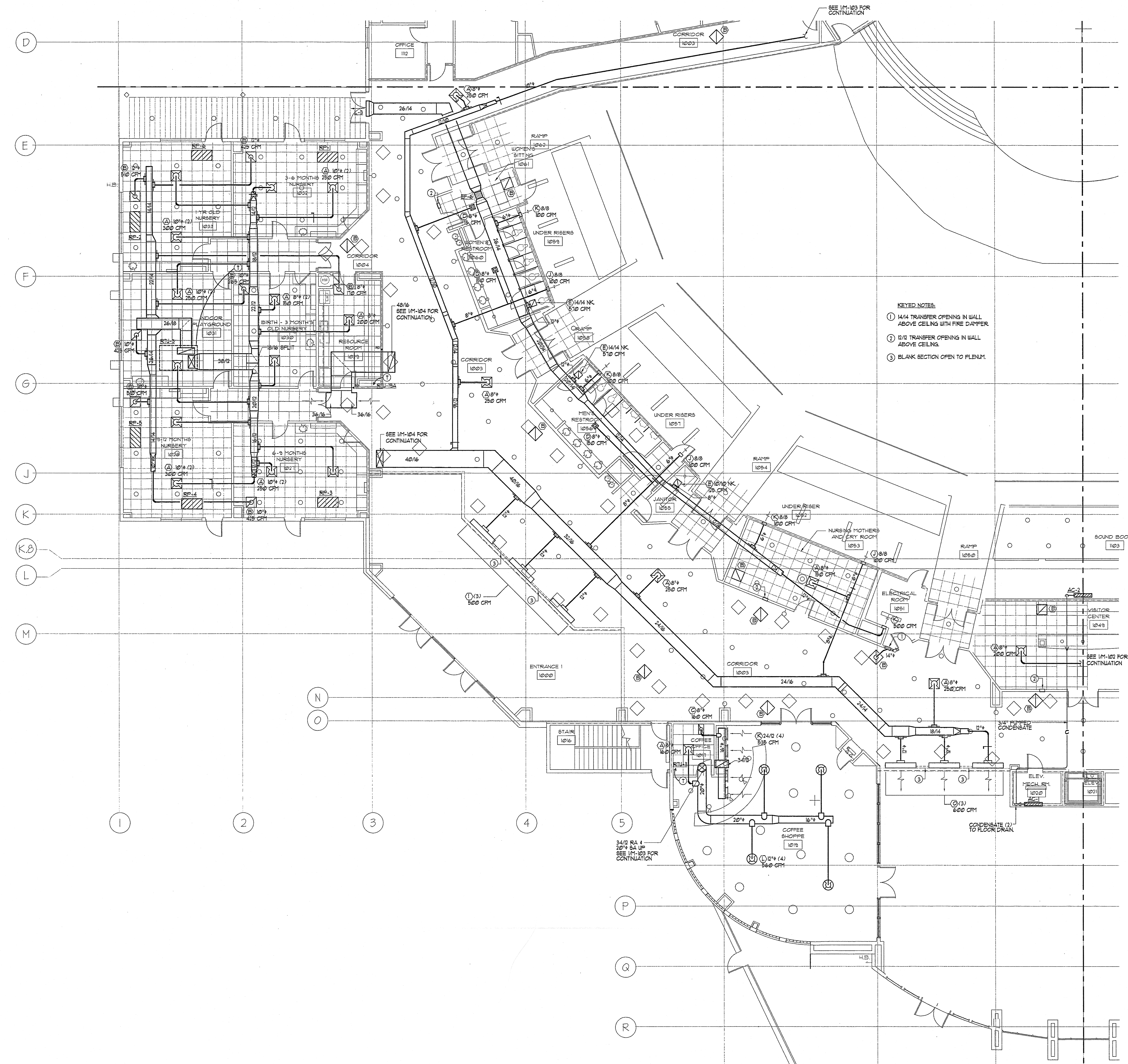
PARTIAL 1st FLOOR PLAN - HVAC SCALE: 1/8" = 1'-0"
