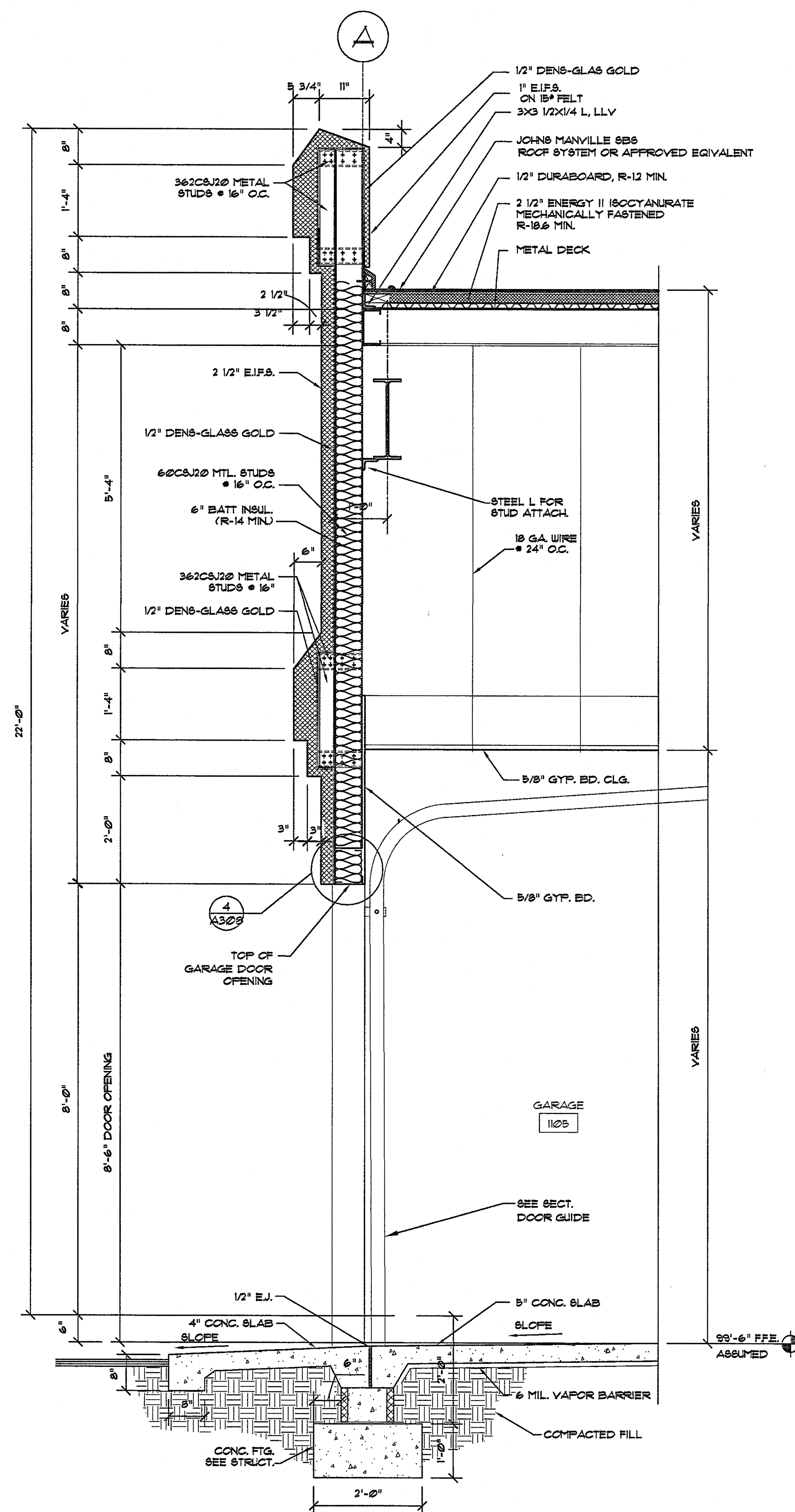
2 SECTION A308 3/4" = 1'-0"
