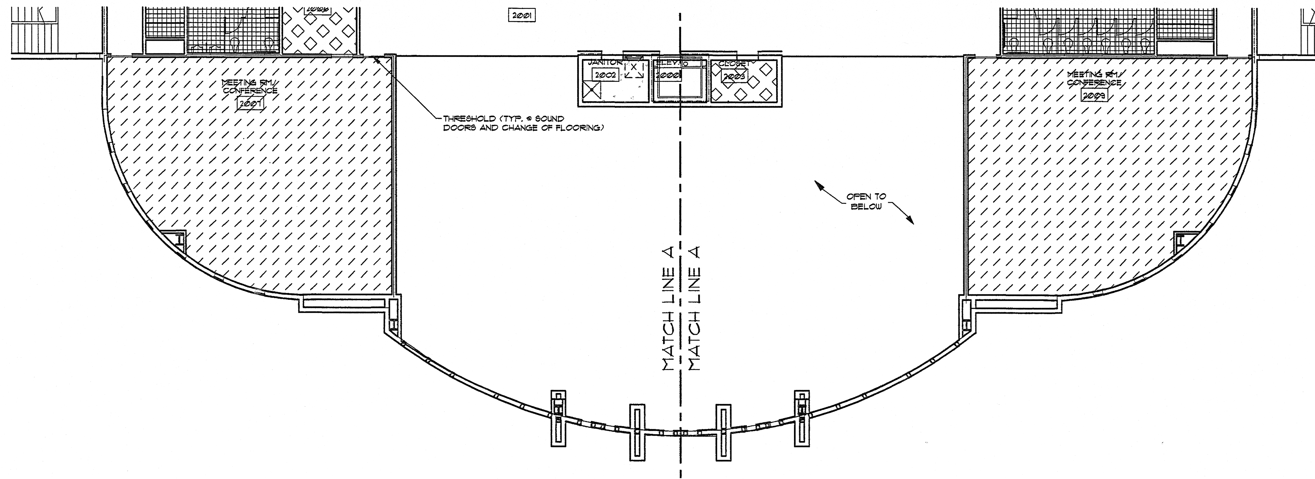
1 SECOND FLOOR FINISH PLAN - PART 2 A118 1/8" = 1'-0"
