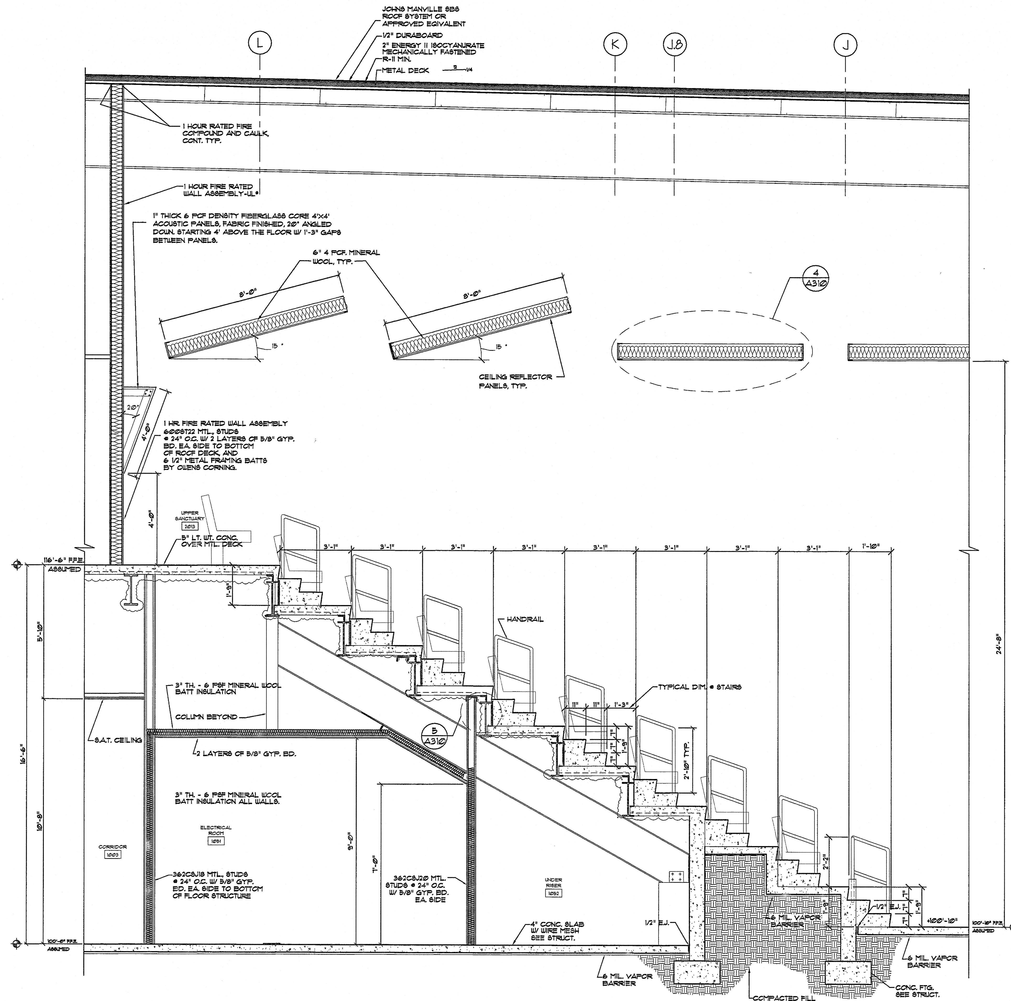
SECTION A320 1/2" = 1'-0"
