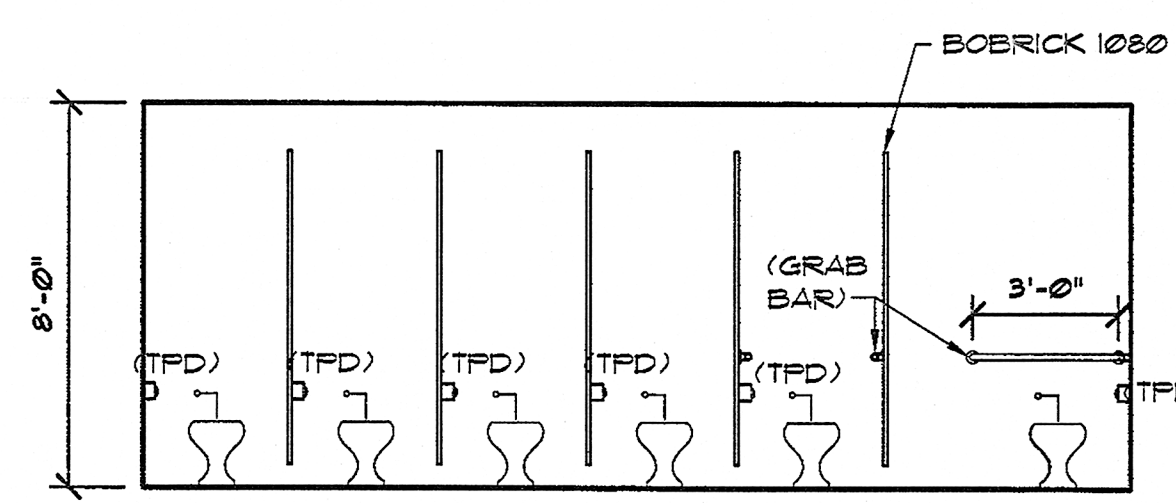
4 WOMEN'S REST ROOM ELEVATION A405 1/4" = 1'-0"
