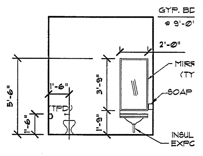
7 CHILDREN'S R R ELEVATIONS A405 1/4" = 1'-0"
