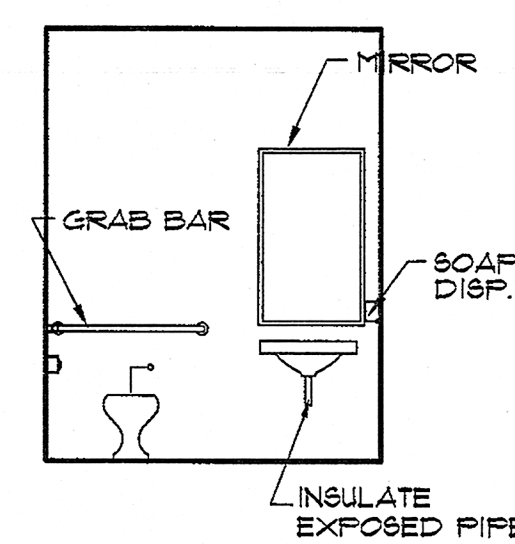
11 LAV ELEVATION A405 1/4" = 1'-0"
