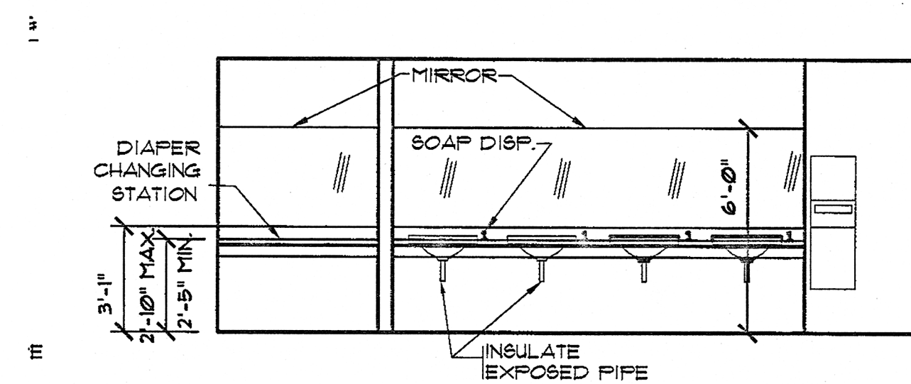
2 WOMEN'S REST ROOM ELEVATION A405 1/4" = 1'-0"
