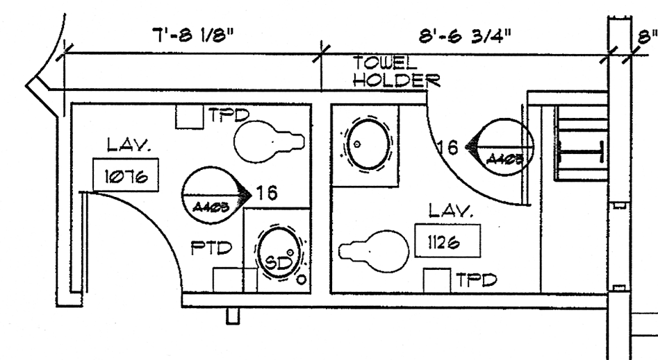
10 LAV PLAN A405 1/4" = 1'-0"
