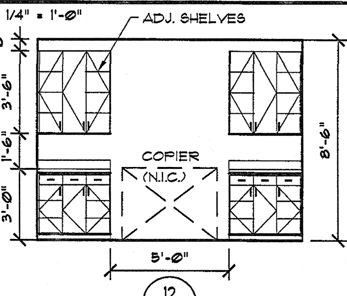
PRIVATE BATH ELEVATIONS A405 1/4" = 1'-0"
