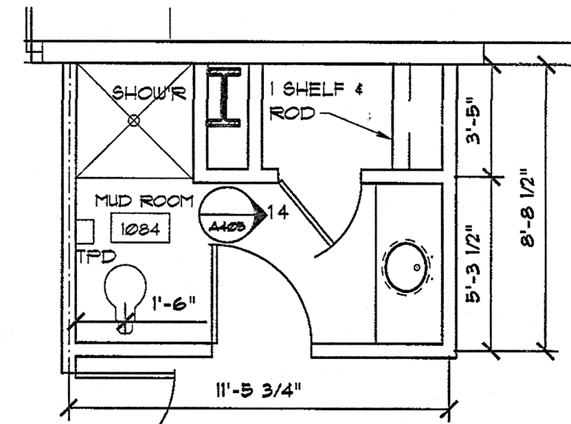
8 MUD ROOM PLAN A405 1/4" = 1'-0"
