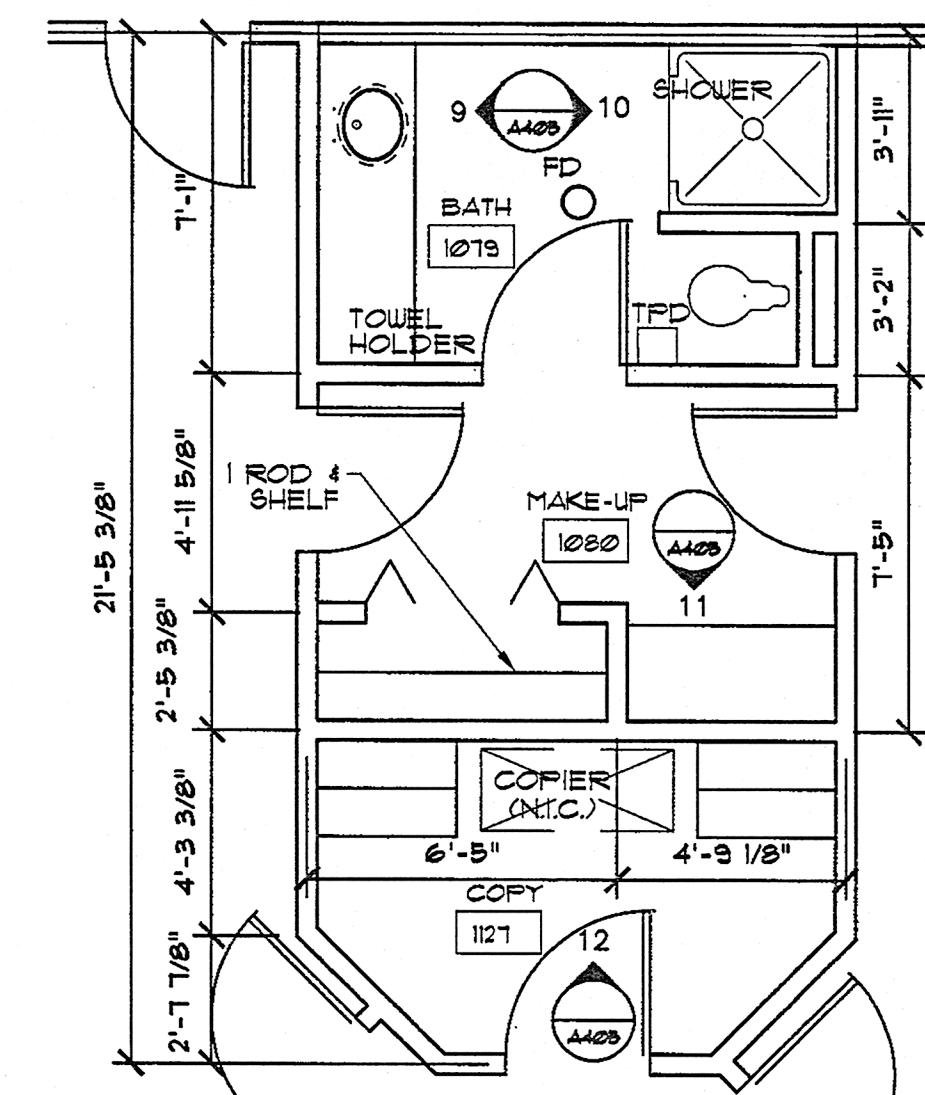
12 PRIVATE BATH PLAN A405 1/4" = 1'-0"
