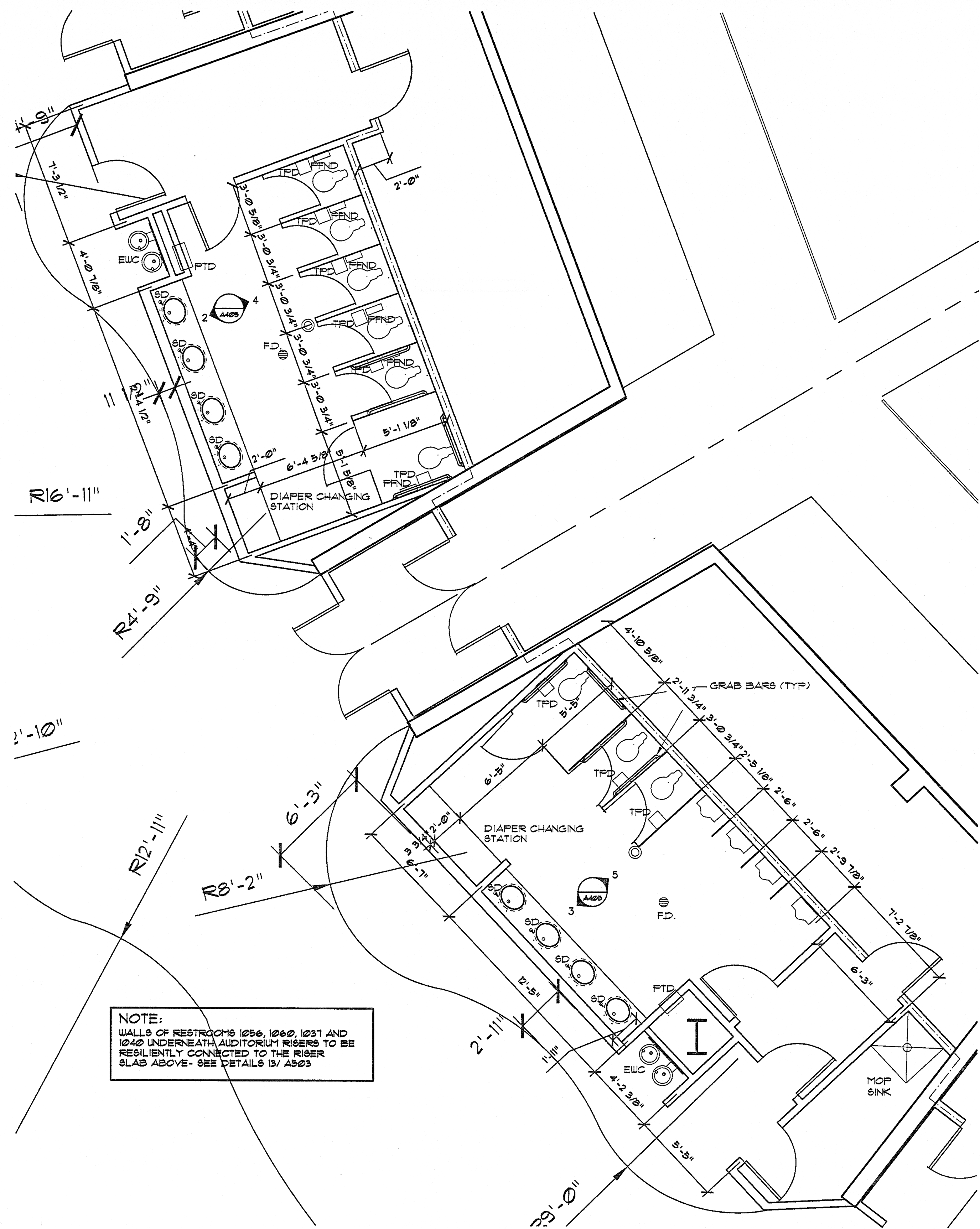
1 MEN & WOMEN REST ROOM PLANS A405 1/4" = 1'-0"
