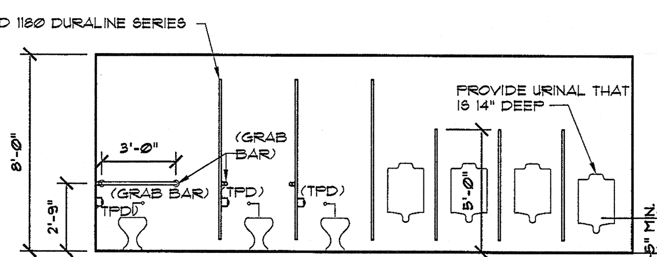
5 MEN'S REST ROOM ELEVATION A405 1/4" = 1'-0"
