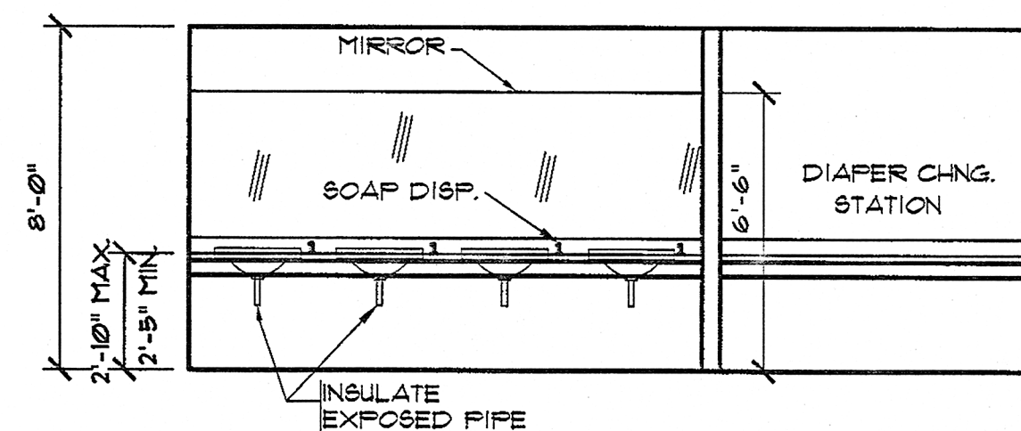
3 MEN'S REST ROOM ELEVATION A405 1/4" = 1'-0"
