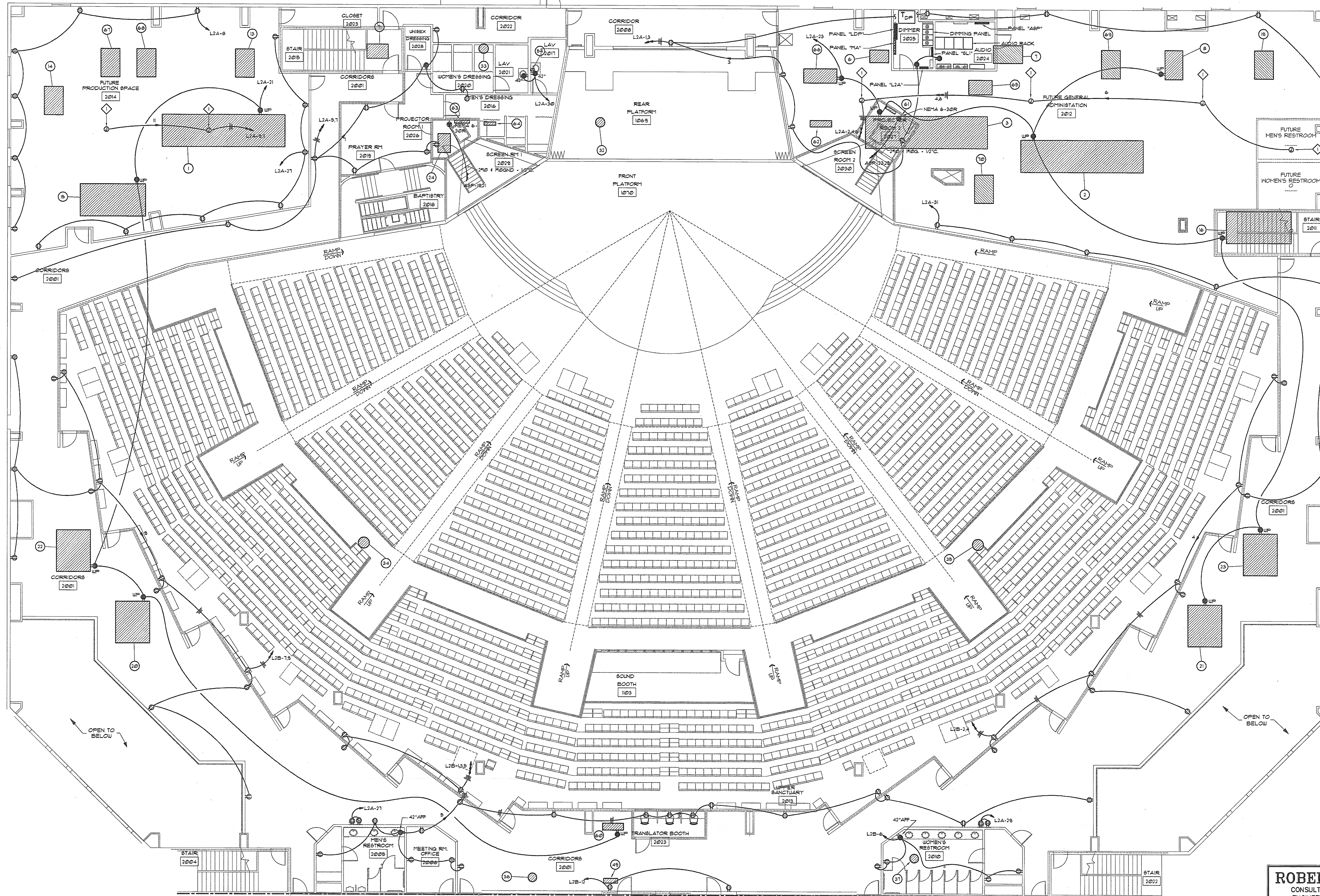
1 SECOND FLOOR PLAN - PART 1 - POWER E-106 SCALE: 1/8" = 1'-0"
