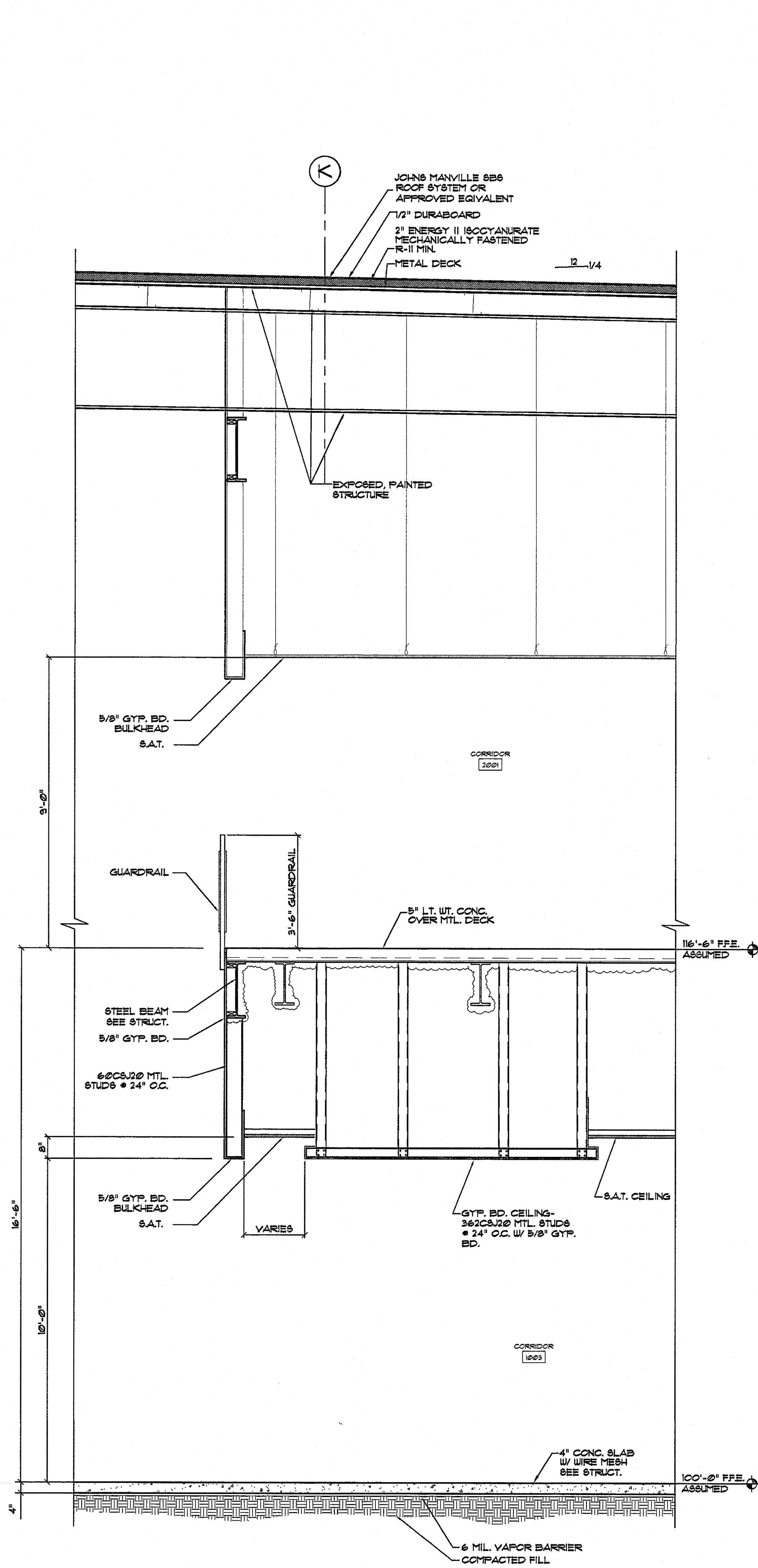
SECTION A312 1/2" = 1'-0"
