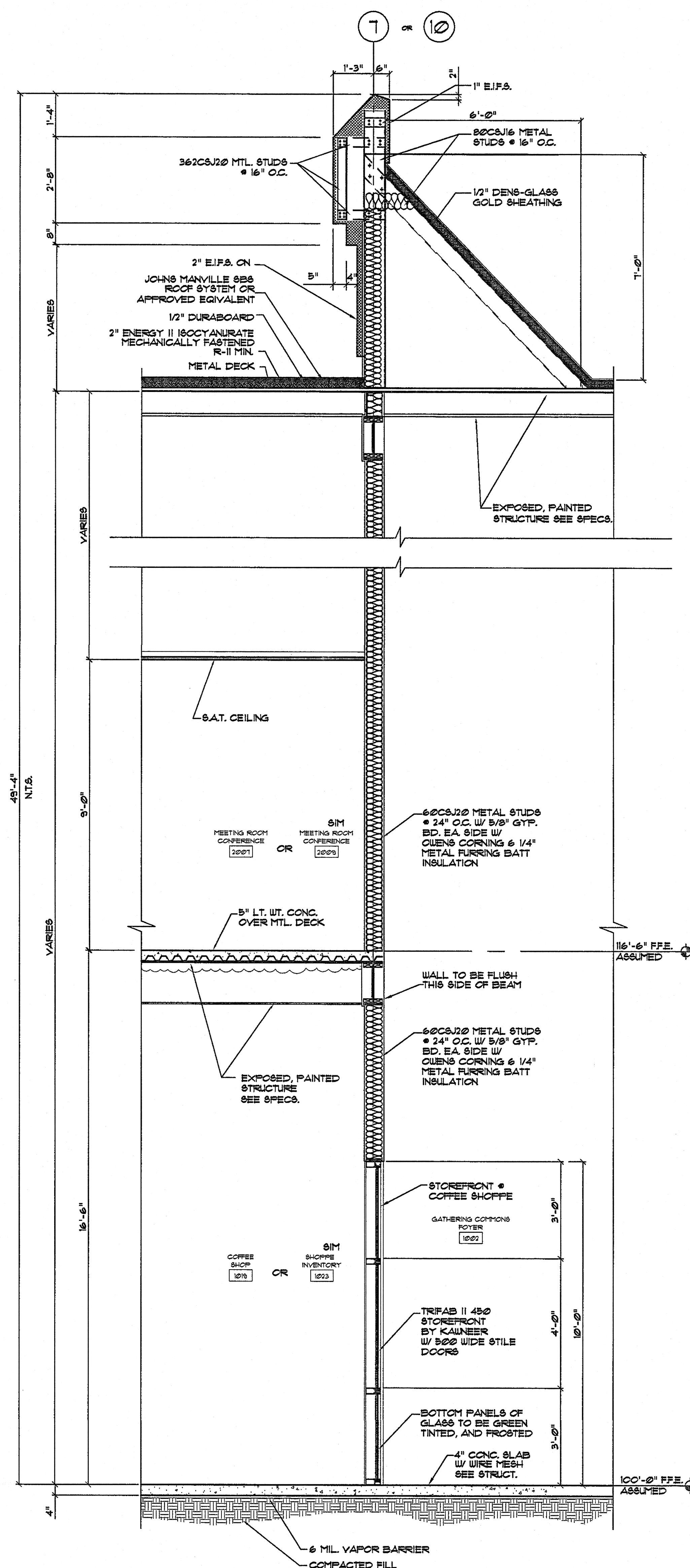
SECTION A312 1/2" = 1'-0"
