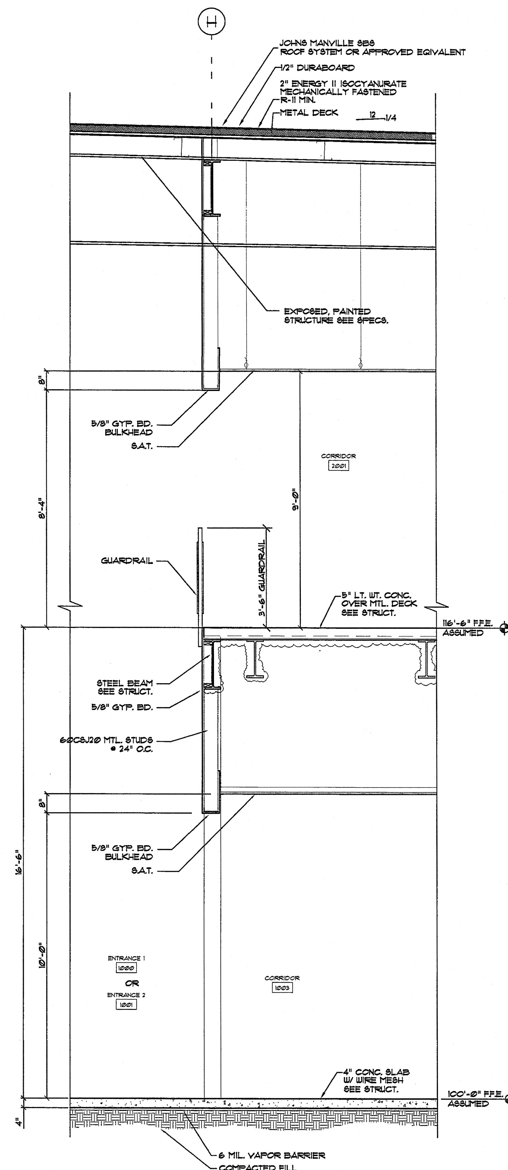
SECTION A312 1/2" = 1'-0"
