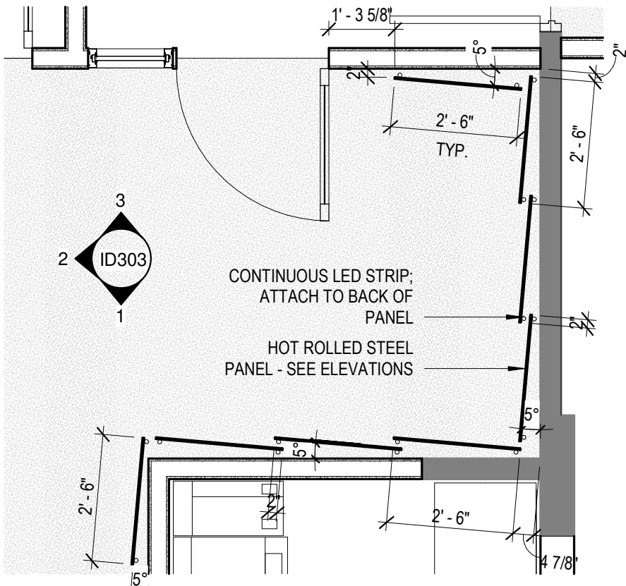
3 ENLARGED PLAN @ TIRE SOUTH ENTRY STEEL PANELS 3/8" = 1'-0"
