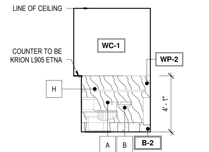
10 RR3 TOILET 1/4" = 1'-0"
