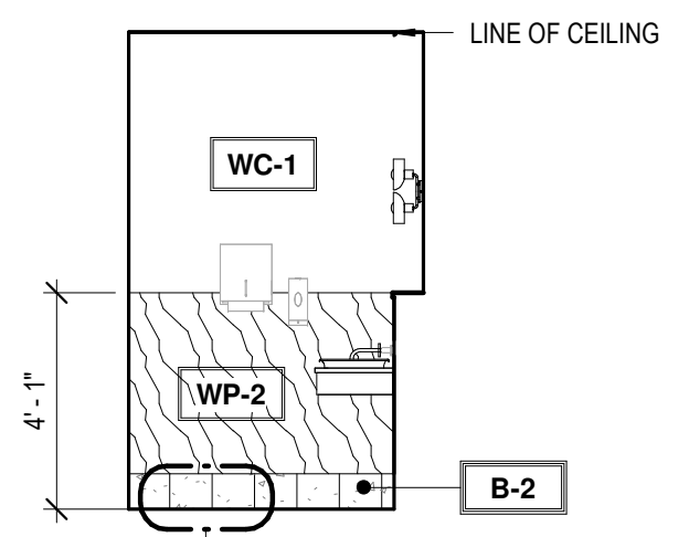
12 RR3 VANITY 1/4" = 1'-0"
