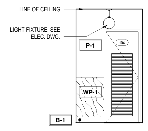
13 RR CORRIDOR TOWARDS JAN. 1/4" = 1'-0"
