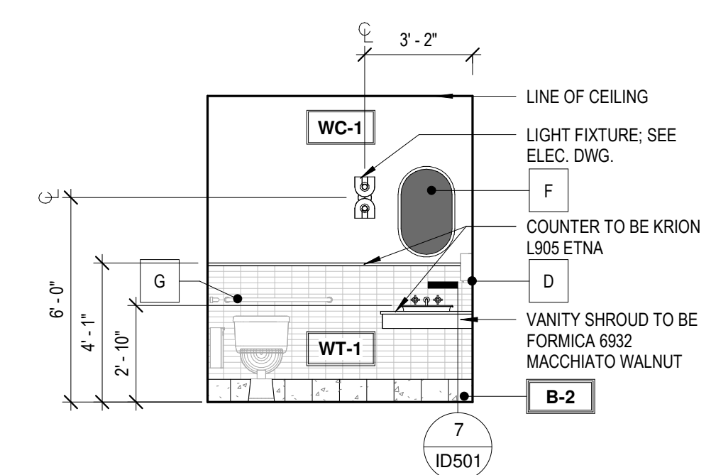
5 RR2 WET WALL 1/4" = 1'-0"
