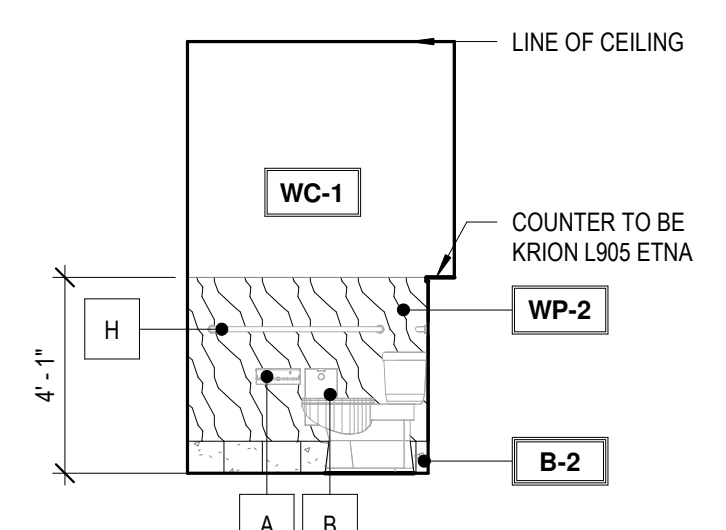
6 RR2 TOILET 1/4" = 1'-0"
