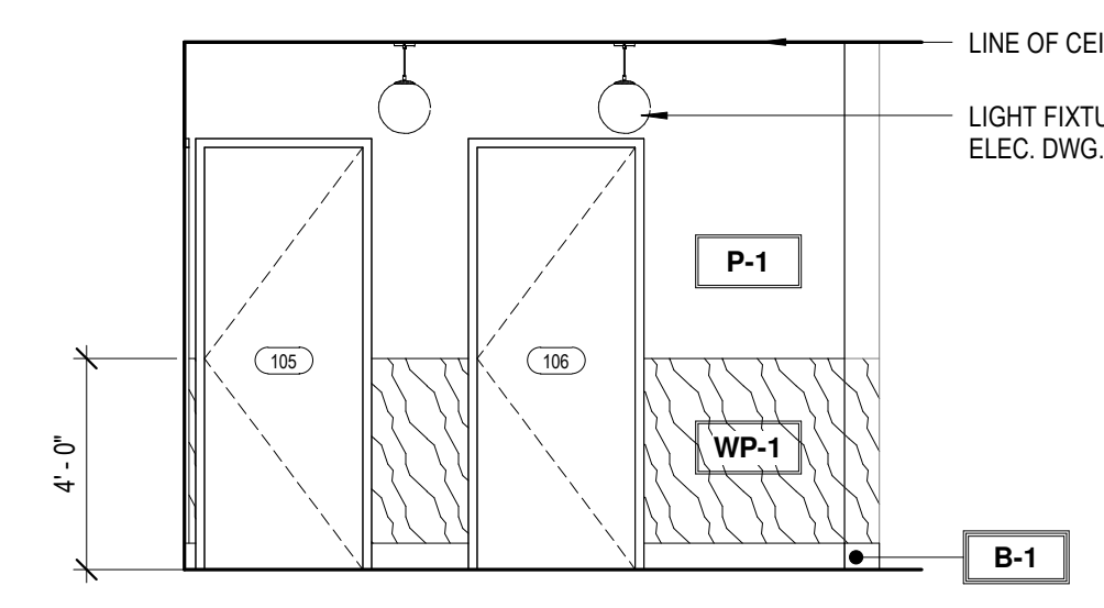
14 RR CORRIDOR TOWARDS RR2 & RR3 1/4" = 1'-0"
