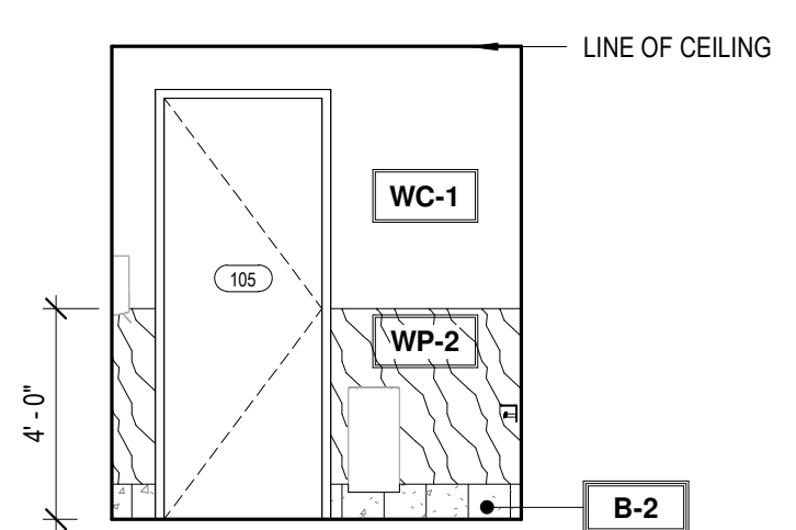
7 RR2 ENTRANCE 1/4" = 1'-0"
