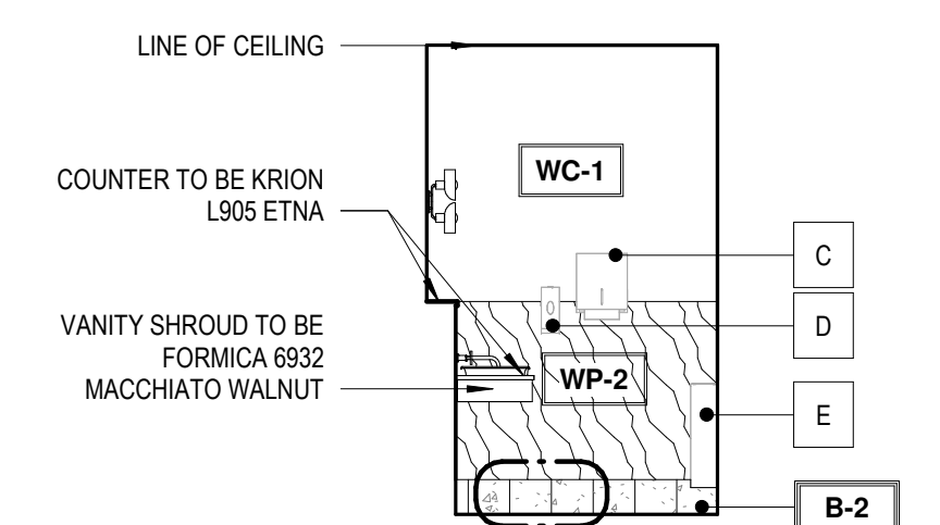
8 RR2 VANITY 1/4" = 1'-0"
