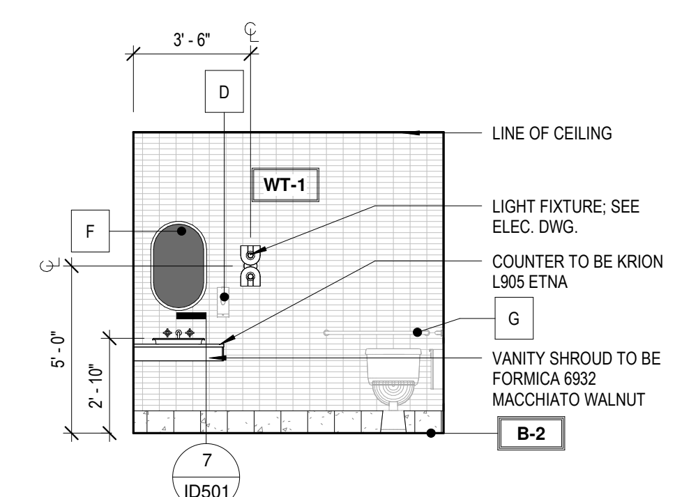
1 RR1 WET WALL 1/4" = 1'-0"
