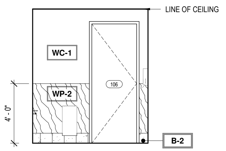
11 RR3 ENTRANCE 1/4" = 1'-0"
